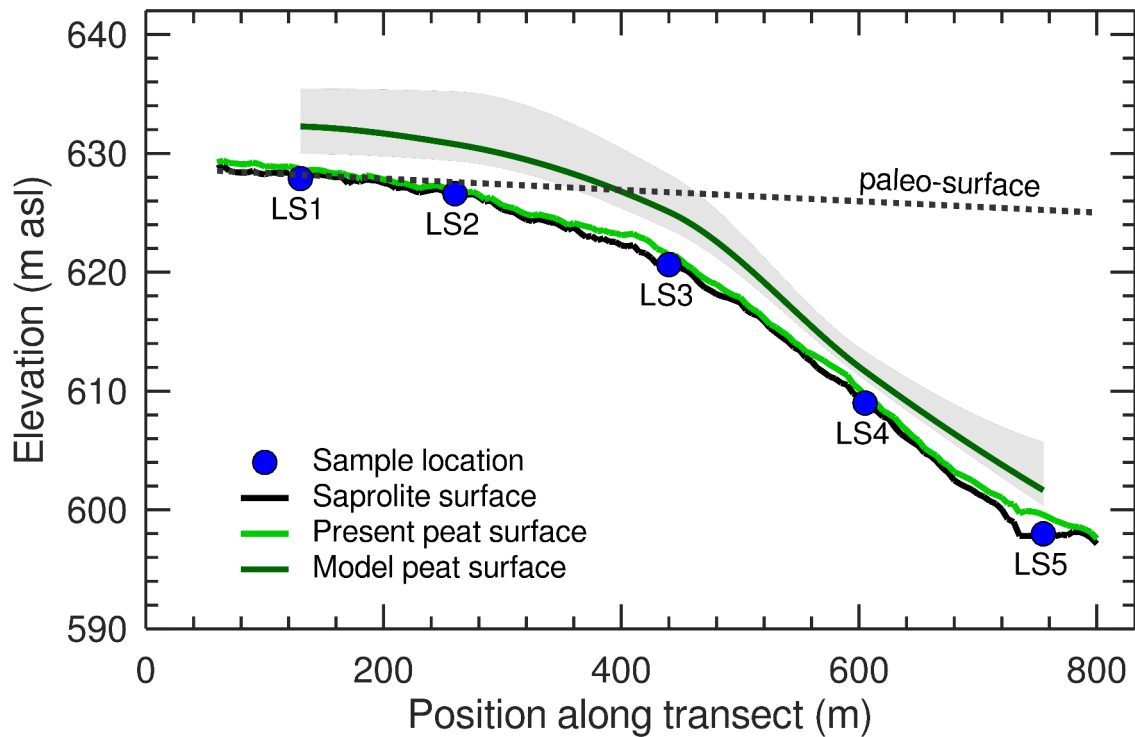
Figure 3: Study hillslope cross section with 10× vertical exaggeration with the five hillslope positions (LS1 to LS5). The black, solid line shows the elevation of the top of the saprolite surveyed with ground penetrating radar (Henrion et al., 2024). The light green line shows the elevation of the modern peat surface. The cosmogenic nuclide-based estimate of peat thickness, interpolated between measurement points, is shown by the dark green line and the 90% confidence interval by the grey band. The dashed, black line shows the elevation and dip of the pre-Senonian surface (labeled paleo-surface).
