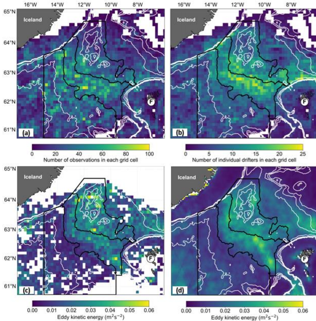
Figure 10. (a) Number of 6-hourly observations in each grid cell by the 101 drifters crossing the IFR. (b) Number of individual drifters (unique drifter ID numbers) entering each grid cell. (c) Distribution of eddy kinetic energy for drifter data. The eddy kinetic energy is only shown for grid cells with at least 5 different drifters passing. (d) Distribution of eddy kinetic energy for SWOT data. Observations in each grid cell for the SWOT is in Supplementary Fig. S7. The grid size for (a), (b) and (c) is 0.1 degrees latitude and 0.2 degrees longitude. The grid size used in (d) is 0.05 degrees latitude and 0.1 degrees longitude. The white lines on both maps show bottom contours for 300m, 350 m, 400 m, 500 m, 1000 m, 1500 and 2000 m. Black lines show the same areas as in Fig. 9. An F in a white circle shows the Faroe Islands.
