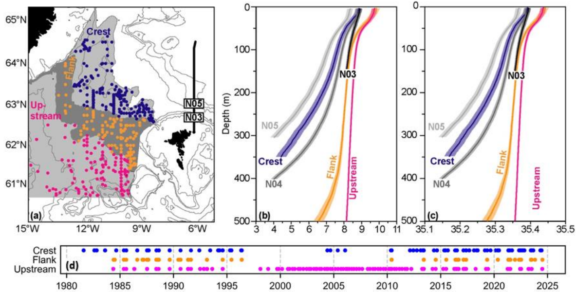
Figure 9. (a) The CTD profiles in the IFR area were divided into three regions: i) Upstream of the IFR (magenta). This region is in the Iceland Basin from 60.7° N and north to the 1000 m isobath and west of 9.6° W to 15° W. There are 209 CTD casts in this region. ii) The flank of the IFR (orange). This is from the 1000 m isobath to the 500 m isobath in the Iceland Basin. Here there are 139 CTD casts. iii) The ridge crest (blue). This region is from the 500 m isobath in the Iceland Basin to the 500 m isobath in the Norwegian Sea, with 330 CTD casts. CTD stations are shown with a dot. The area borders are shown with grey shading. The N-section is shown with a thick black line north of the Faroes and two standard CTD stations N03 and N05 are indicated. Thin grey lines show bottom contours for 200 m, 400 m, 500 m, 1000 m, 1500 m and 2000 m. Mean temperature (b) and salinity (c) profiles for the three regions in (a). Semi-transparent areas around each profile show the average \pm one standard error. Upstream and on the flank, only CTD casts that are at least 500 m deep were included. On the crest, only casts that are at least 350 m were included. The profiles for the three standard stations on the N-section N03, N04 and N05 are also shown down to the depth of the 4 °C isotherm, defined as the deep boundary of Atlantic water on the section (Hansen et al., 2023). (d) Time of observation for the profiles in the three regions.
