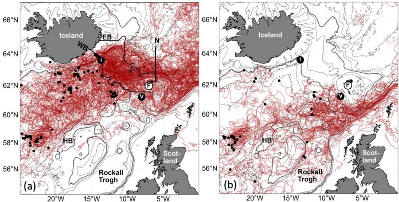
Figure 3. (a) Flow paths of 101 drifters crossing the IFR. Black curves show the western boundary (WB) and the eastern boundary (EB) defining the IFR area. The thick black line north of the Faroes (F) indicates the N-section. (b) 44 drifters passing south of the Faroes. Black circles on both maps show where the drifters were deployed if they fall inside the map area. In a) six deployment locations fall outside the map and in b) eight deployment locations fall outside. Drifter paths are shown with semi-transparent red lines. Grey lines show bottom contours for 200 m, 500 m, 1000 m, 1500 m, 2000 m and 3000 m with a thicker 1000 m contour. HB is Hatton Bank. Black circles with white letters show the locations of standard stations I and V.
