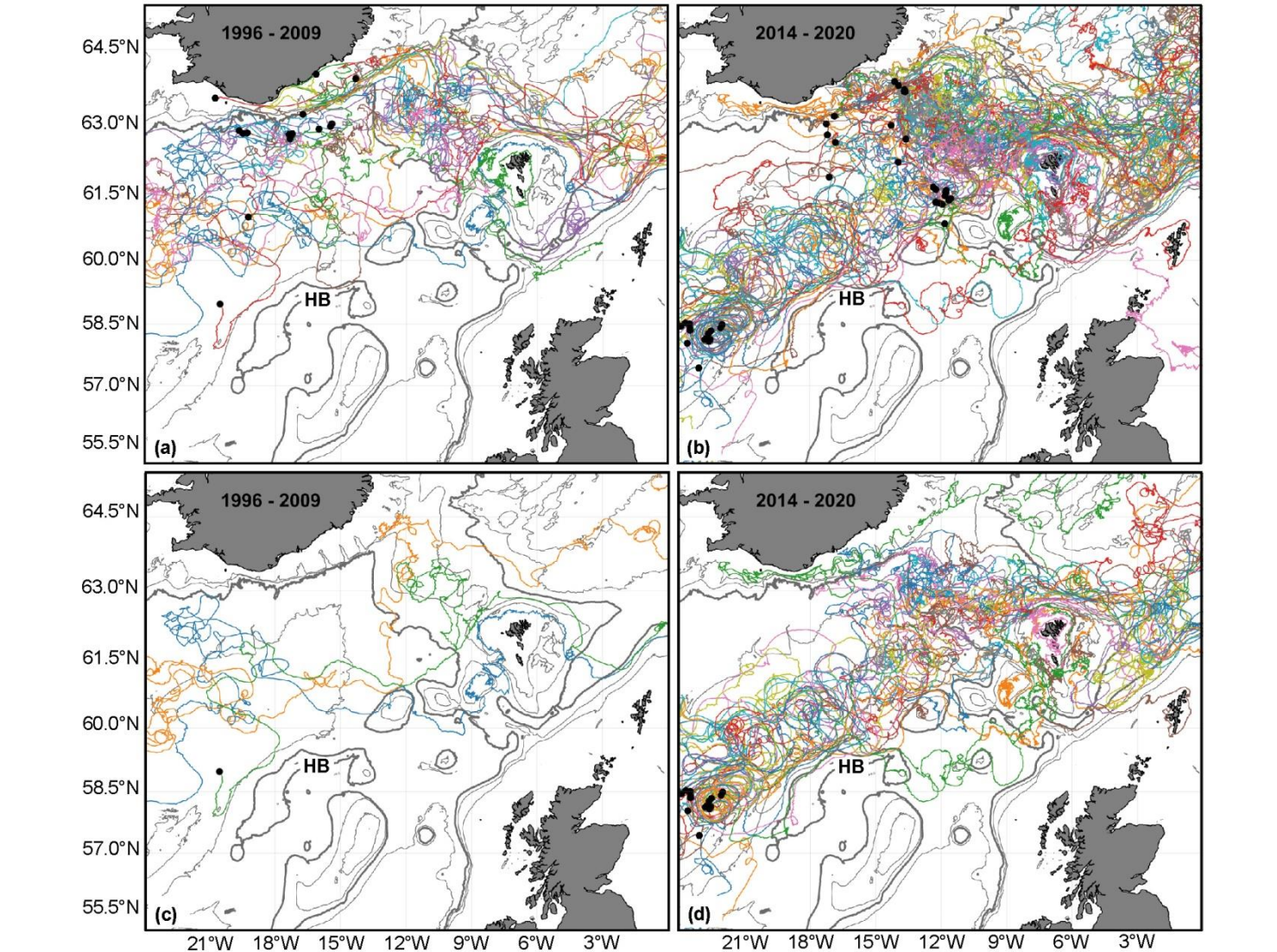
Figure 5 (a), (c) Drifters crossing IFR in a period with no or little intrusion of the SPG into the Iceland Basin ( pc_1 was low). (b), (d) Drifters crossing IFR in a period where SPG intruded far into the Iceland Basin ( pc_1 was high). (a) All the drifters (19) crossing in the period from 1996 to 2009. (c) The same as in (a), but only those drifters (3) that were deployed south of 60° N. (b) All drifters (50) crossing in the period from 2014 to 2020. (d) The same as in (b), but only drifters (23) deployed south of 60° N. Black circles show where the drifters were deployed if they fall inside the map area. In a) three deployment locations fall outside the map, in b) eight deployment locations fall outside, in c) two deployment locations fall outside and in d) eight deployment locations fall outside. Grey lines show bottom contours for 200 m, 500 m, 1000 m, 2000 m and 3000 m with a thicker 1000 m contour. HB: Hatton Bank.
