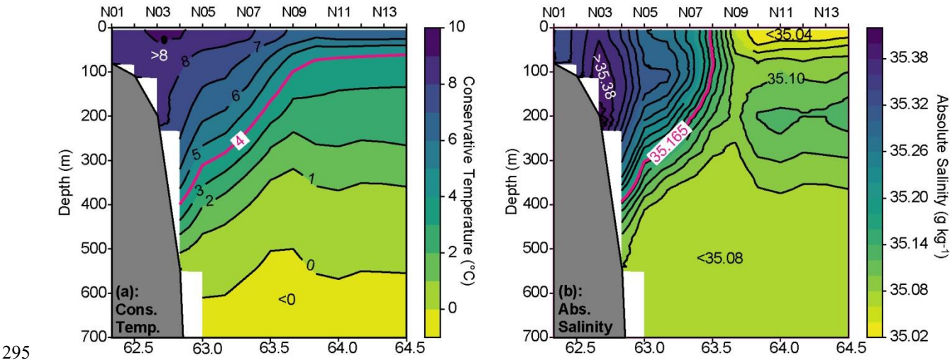
295 Figure 7. Average water mass characteristic at the N-section. Mean Conservative Temperature (a) and Absolute Salinity (b) for the period from 1993 to May 2024 from 99 cruises where all 14 standard stations were occupied. Magenta lines show the 4 °C isotherm and the 35.165 g kg -1 isohaline (corresponding to the 35.0 isohaline in practical salinity units), used by Hansen et al. (2023) to define the deep and northern 300 boundary of Atlantic water on the section.
