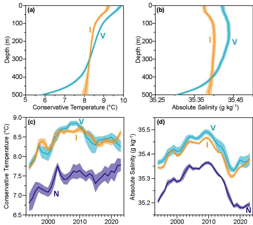
275 Figure 6. Average profiles of Conservative Temperature (a) and Absolute Salinity (b) for the two standard stations I (orange) and V (cyan) upstream of the IFR. For positions see Fig. 1. Three-year running mean de-seasoned temperature (c) and salinity (d) averaged from the surface to 500 m depth for the two standard stations I (orange) and V (cyan). Dark blue curves show transport-weighted temperature (c) and salinity (d) on the N-section (see text). In all the panels, semi-transparent areas indicate average \pm one standard error.
