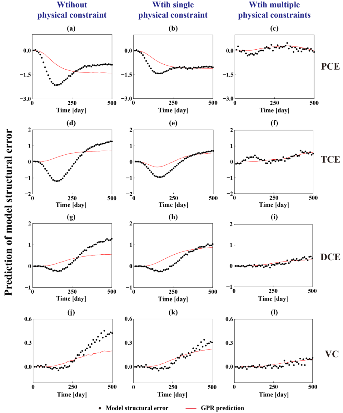
Figure 12. Predictions of model structural errors for the synthetic groundwater PCE reactive transport model without physical constraints (a, d, g, j), with single physical
