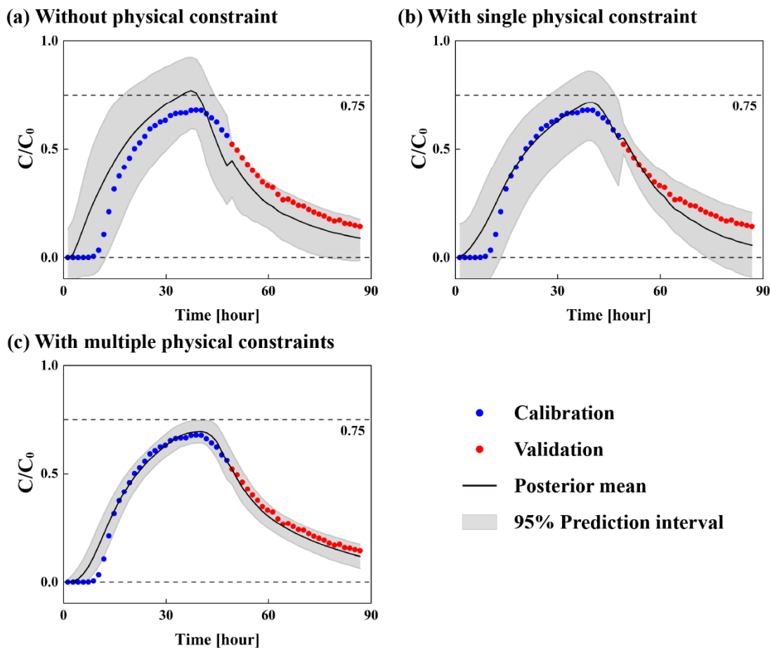
Figure 9. DDM predictions of cadmium concentration under the three scenarios.
