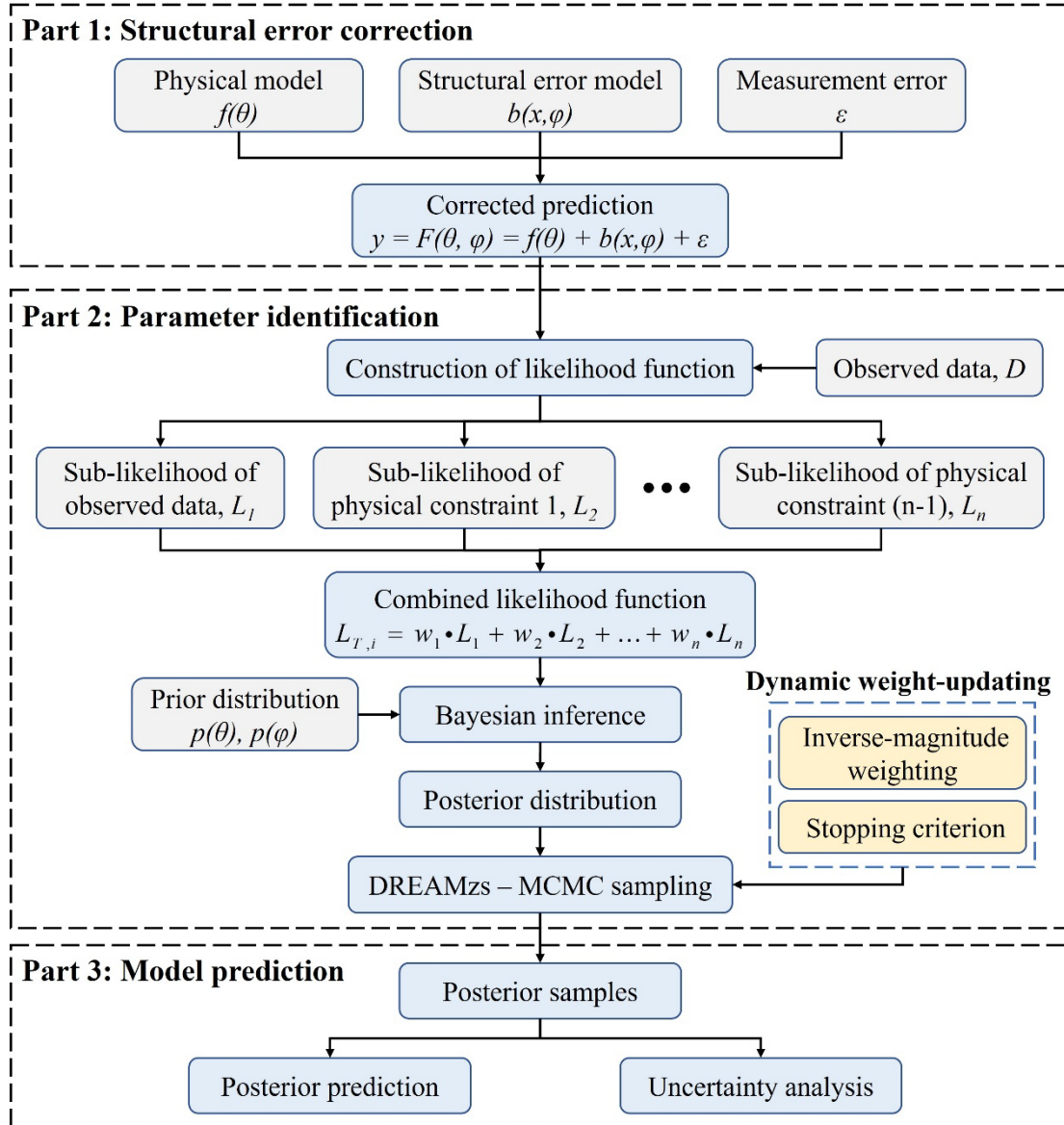
Figure 1. Overall workflow of the proposed framework.
