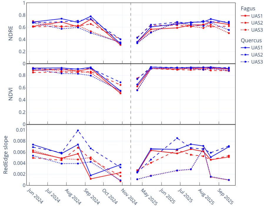
Figure 9. Averaged NDVI, NDRE, and red-edge slope values for beech and oak trees at three test sites, derived from UAS measurements during the vegetation periods of 2024 and 2025.
