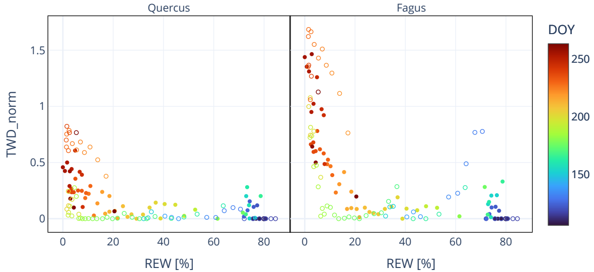
Figure 7. Mean normalized tree water deficit ( TWD_{norm} ) of Oak and Beech in relation to soil moisture expressed as relative extractable water (REW). Filled circles: 2024, open circles: 2025.
