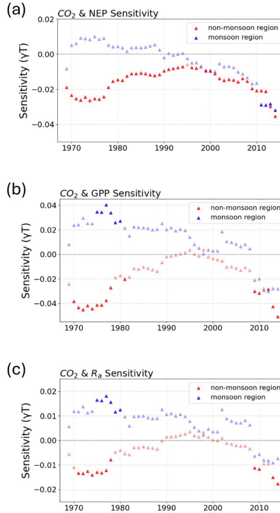
185 Figure 3. Time series of the sensitivity between atmospheric CO 2 growth and (a) NEP, (b) GPP, (c) R a over 20-year moving window in 1959-2023 (see Data and Methods for details). Markers show the ensemble mean of nine TRENDY models for the non-monsoon (red) and monsoon (blue) regions. Dark markers indicates statistically significant regression slope within each moving window, whereas faded markers indicate non-significant slope; p>0.1 was considered statistically non-significant.
