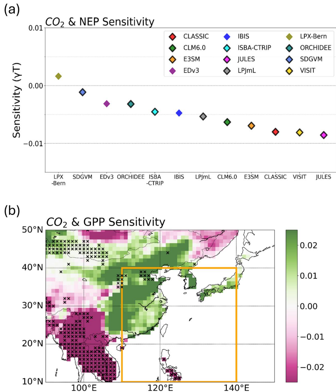
155 Figure 2. (a) Scatter plot of the sensitivity between atmospheric CO_2 growth and NEP during 1959-2023, based on 12 models from TRENDY v13. Each scatter represents atmospheric CO_2 growth and NEP sensitivity of an individual model. Models with statistically significant relationships at the 95% confidence level (from the last 20-year window)
