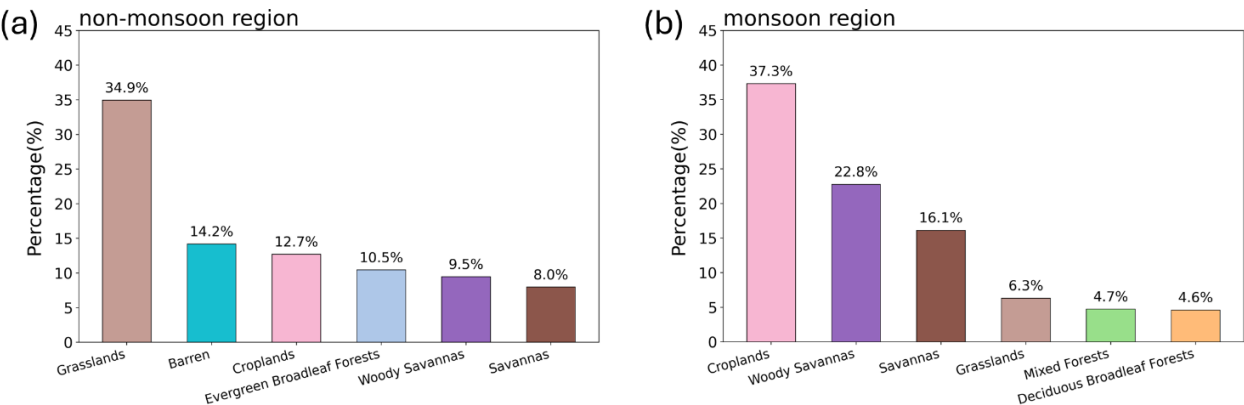
Figure 7. East Asian land cover distribution based on IGBP classification. MODIS land cover averaged during 2001-2023, regridded to 1.0^{\circ} \times 1.0^{\circ} spatial resolution, showing the percentage distribution of land cover types in the (a) non-monsoon and (b) monsoon region. For all panels, see Data and Methods for details.
