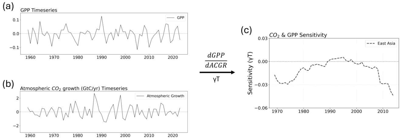
Figure 1. Methodological procedure for ecosystem productivity sensitivity to atmospheric \text{CO}_2 growth. (a) Detrended time series of GPP over East Asia from nine TRENDY v13 models. (b) Detrended atmospheric \text{CO}_2 growth from the Global Carbon Budget 2024. (c) Sensitivity of atmospheric \text{CO}_2 growth and GPP over 20-year moving windows in for the entire 1959-2023 period. For all panels, see Data and Methods for details.
