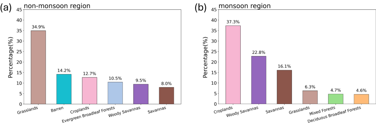
335 Figure 7. East Asian land cover distribution based on IGBP classification. MODIS land cover averaged during 2001-2023, regridded to 1.0° × 1.0° spatial resolution, showing the percentage distribution of land cover types in the (a) non-monsoon and (b) monsoon region. For all panels, see Data and Methods for details.
