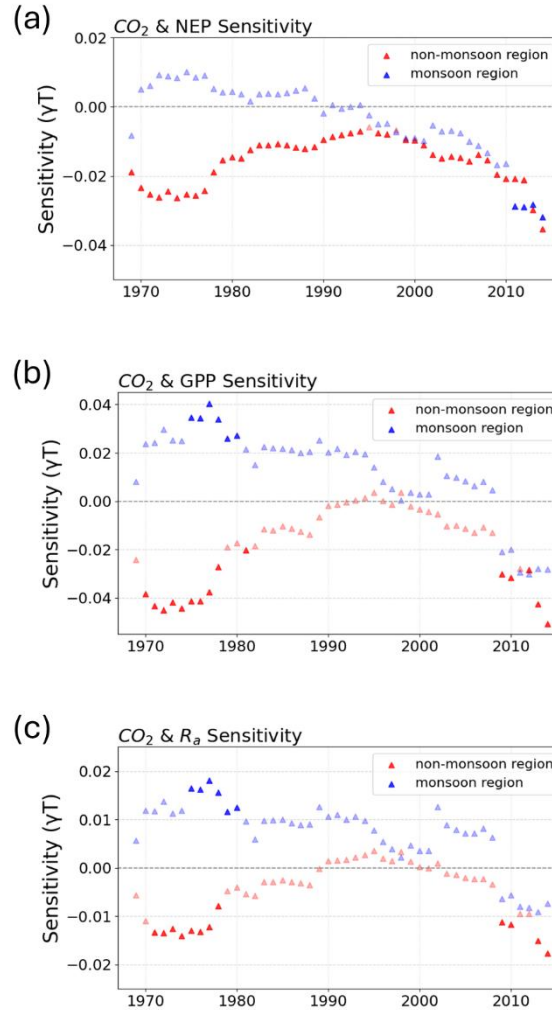
Figure 3. Time series of the sensitivity between atmospheric CO 2 growth and (a) NEP, (b) GPP, and (c) R a overusing 20-year moving window in windows over the entire period from 1959- to 2023 (see Data and Methods for details). Markers show the ensemble mean of nine TRENDY models for the non-monsoon (red) and monsoon (blue) regions. Dark markers indicate statistically significant regression slope within each moving window, whereas faded markers indicate non-significant slope; p > 0.1 was considered statistically non-significant.
