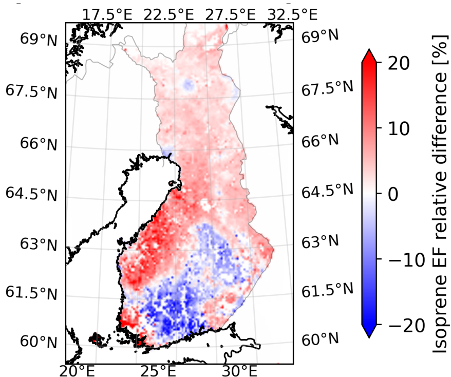
Figure 5. Relative difference between the isoprene emission factors calculated using the "simple" speciation compared to the "advanced" speciation. The "advanced" EFs have been used as a reference.
