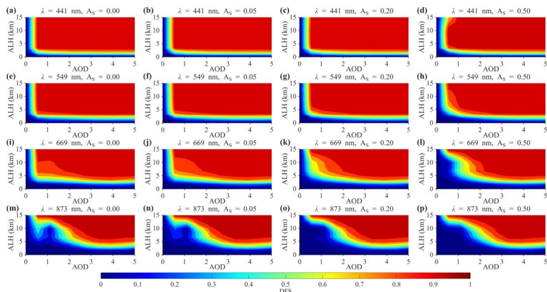
Fig. 1. Characteristics of ALH-AOD 441 -DFS distributions derived from radiance under different spectral bands and surface reflectance conditions. The simulations were conducted for smoke aerosols, with AOD 441 ranging from 0 to 5 as the common reference aerosol loading parameter. For all subplots, the x-axis represents AOD 441 . Rows correspond to wavelengths of 441 nm, 549 nm, 669 nm, and 873 nm, respectively, while columns represent different surface reflectance conditions ( A_s = 0.00, 0.05, 0.20, 0.50 ). Colors indicate the DFS values of ALH, ranging from 0 to 1.
