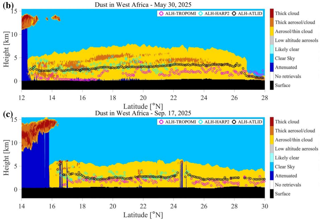
Fig. 11. Comparison of ALH-HARP2 and ALH-TROPOMI with the corresponding ATLID measurements for dust cases on the feature classification curtain plot. Panels (a)-(c) present comparisons of ALH-HARP2 and ALH-TROPOMI with ATLID in three dust cases, respectively.
