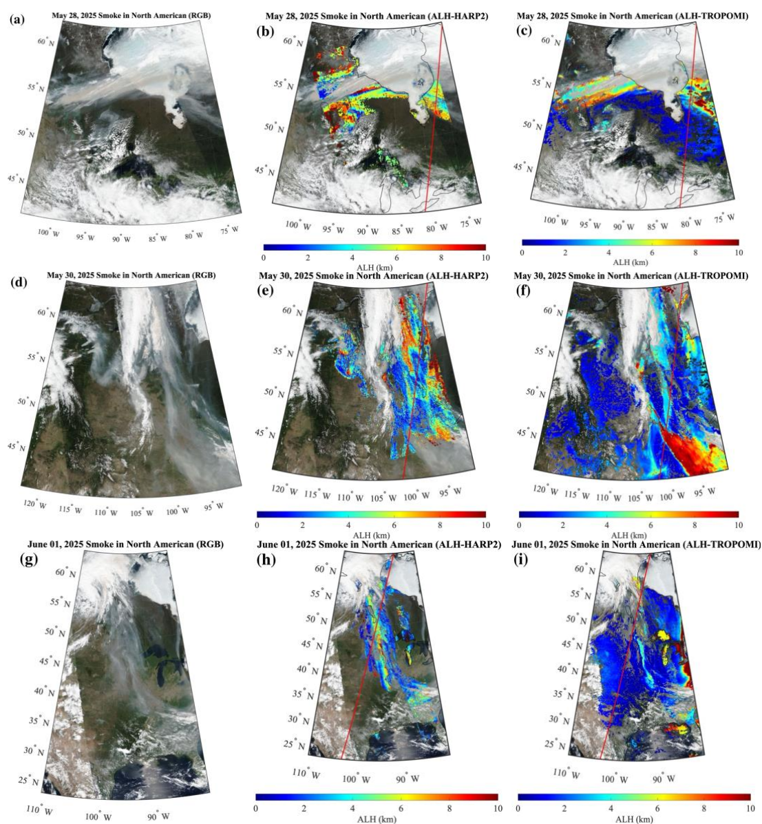
Fig. 8. Examples of retrieval for smoke cases. The first column presents the corresponding true-color images from VIIRS/Suomi-NPP. The second column displays the HARP2-derived ALH
