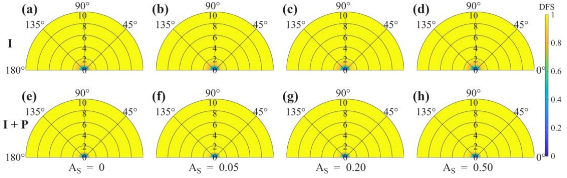
Fig. 6. Same as Fig. 2, but with VZA = 80^\circ .
