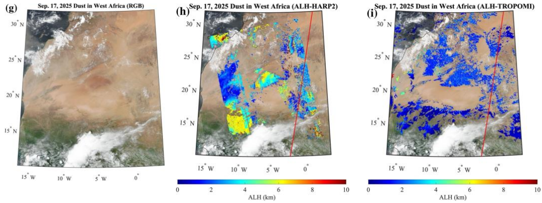
Fig. 10. Examples of retrieval for dust cases. The first column presents the corresponding true-color images from VIIRS/Suomi-NPP. The second column displays the HARP2-derived ALH relative to sea level with the red line representing the EarthCARE track. The third column presents the TROPOMI Level 2 ALH product.
