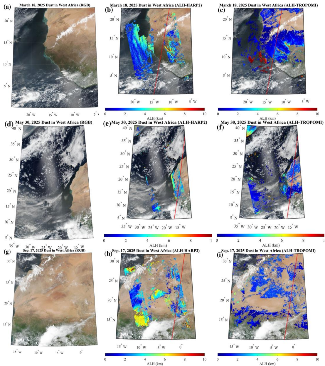
Fig. 10. Examples of retrieval for dust cases. The first column presents the corresponding true-color images from VIIRS/Suomi-NPP. The second column displays the HARP2-derived ALH relative to sea level with the red line representing the EarthCARE track. The third column presents the TROPOMI Level 2 ALH product.
