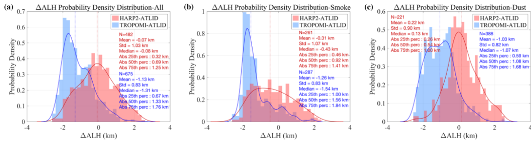
Fig. 14. Histograms and statistical metrics of the differences between ALH-HARP2, ALH-TROPOMI, and ATLID observations at the co-located are presented. The statistics include the total number of data points (N), mean, standard deviation (Std), and median, with the dashed line representing the median value. Panel (a) includes all cases, while Panels (b) and (c) correspond to smoke and dust cases, respectively.
