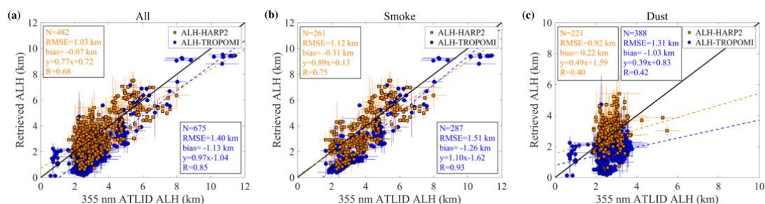
Fig. 13. Comparison of the ALH-HARP2, ALH-TROPOMI with the corresponding ATLID in all cases on a pixel-by-pixel measurement value. (a) Scatter plots of matched ALH-HARP2 (orange markers) and ALH-TROPOMI (blue markers) against ATLID observations, including all matched pixel pairs from all cases. (b) Same as (a), but only including the smoke aerosol cases. (c) Same as (a), but only including the dust cases. The dashed lines in the scatter plots represent the linear regression fits. The one-to-one reference line (black solid line), the number of samples (N), the linear regression equation, and the correlation coefficient (R) are also indicated in the figure. Error bars for both the retrieved ALH and the ATLID-observed ALH represent the standard deviation of values aggregated within a 10 \text{ km} \times 10 \text{ km} spatial window.
