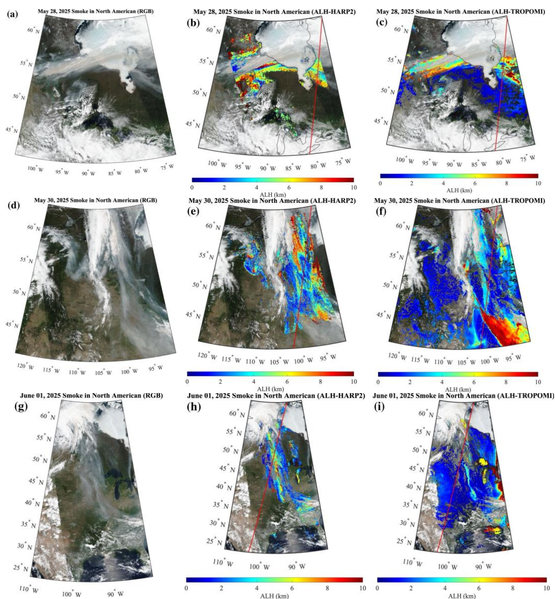
Fig. 8. Examples of retrieval for smoke cases. The first column presents the corresponding true-color images from VIIRS/Suomi-NPP. The second column displays the HARP2-derived ALH relative to sea level with the red line representing the EarthCARE track. The third column presents the TROPOMI Level 2 ALH product.
