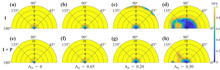
Fig. 4. Same as Fig. 2, but with VZA = 40^\circ .
