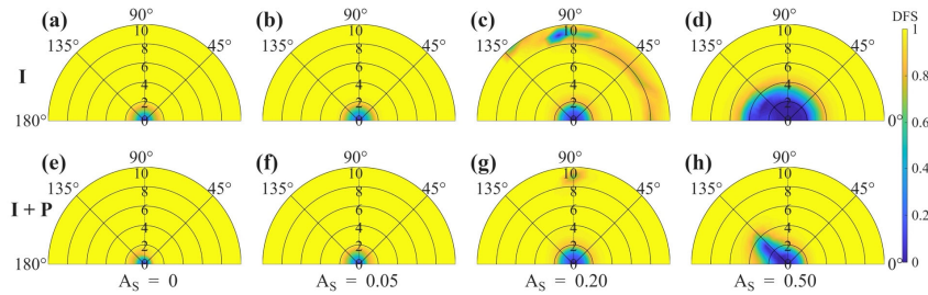
Fig. 3. Same as Fig. 2, but with VZA = 20^\circ .
