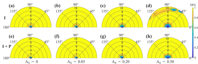
Fig. 5. Same as Fig. 2, but with VZA = 60^\circ
