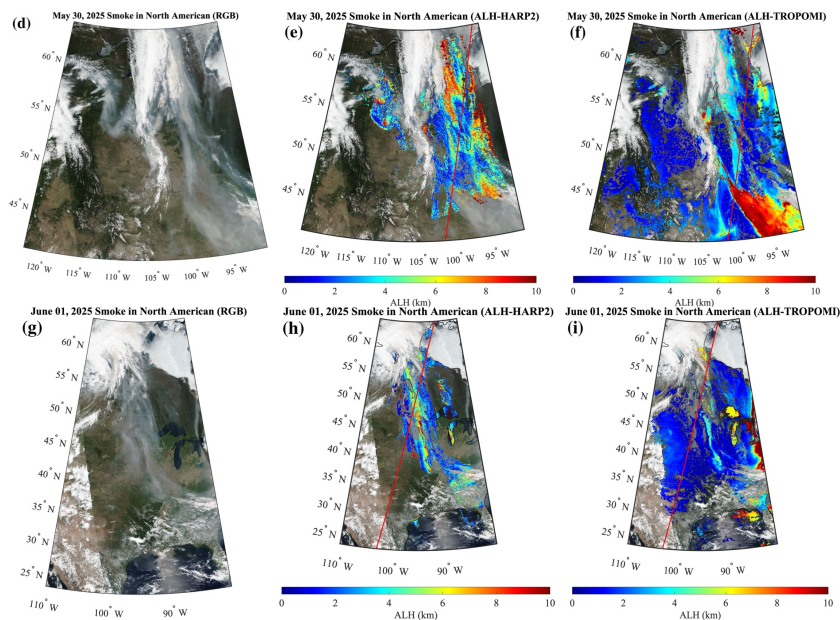
Fig. 8. Examples of retrieval for smoke cases. The first column presents the corresponding true-color images from VIIRS/Suomi-NPP. The second column displays the HARP2-derived ALH relative to sea level with the red line representing the EarthCARE track. The third column presents the TROPOMI Level 2 ALH product.
