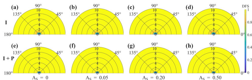
Fig. 6. Same as Fig. 2, but with VZA = 80^\circ .
