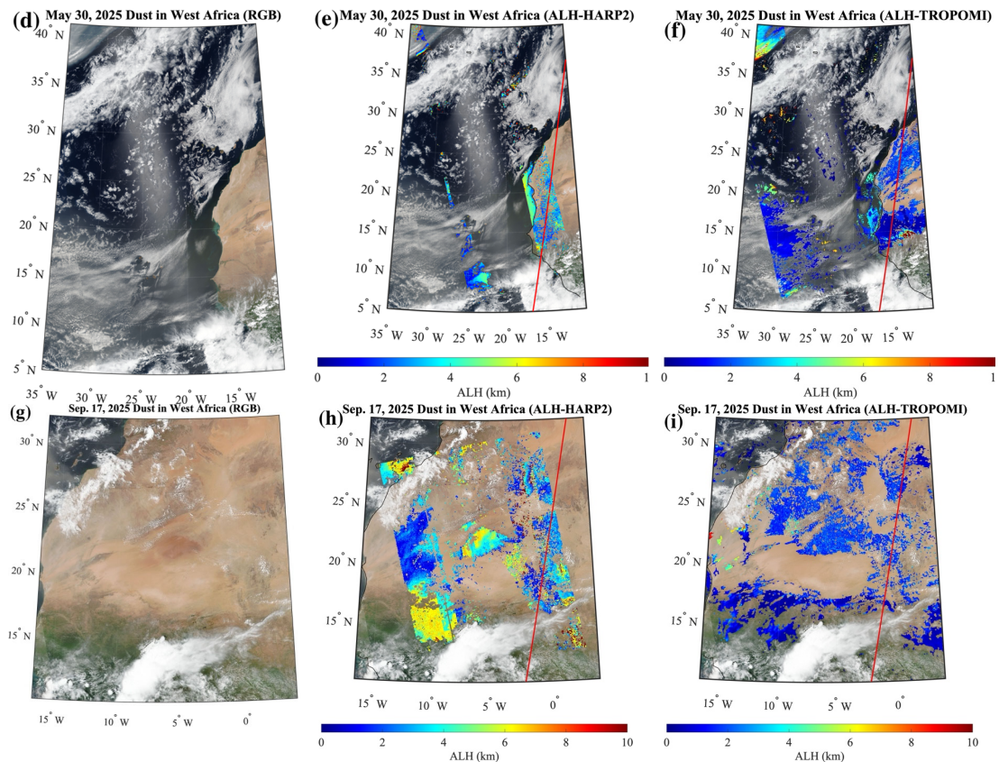
Fig. 10. Examples of retrieval for dust cases. The first column presents the corresponding true-color images from VIIRS/Suomi-NPP. The second column displays the HARP2 -derived ALH relative to sea level with the red line representing the EarthCARE track. The third column presents the TROPOMI Level 2 ALH product.
