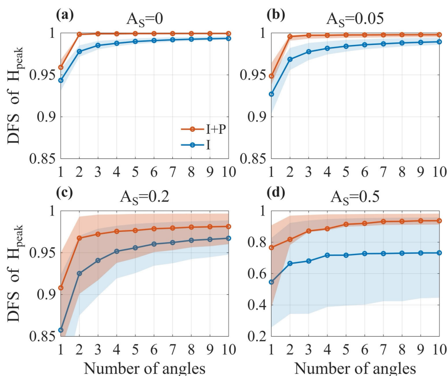
Fig. 7. Influence of the number of viewing angles and polarization information on the DFS under different surface reflectance conditions A_s . Panels (a)-(d) correspond to surface reflectance values of 0, 0.05, 0.20, and 0.50, respectively. Red curves represent joint observations of radiance and polarization (I+P), while blue curves correspond to radiance-only (I) observations. Shaded areas indicate the variation of DFS due to SZA changes within the range of 25^\circ to 60^\circ .
