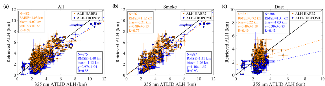
Fig. 13. Comparison of the ALH-HARP2, ALH-TROPOMI with the corresponding ATLID in all cases on a pixel-by-pixel measurement value. (a) Scatter plots of matched ALH-HARP2 (orange markers) and ALH-TROPOMI (blue markers) against ATLID observations, including all matched pixel pairs from all cases. (b) Same as (a), but only including the smoke aerosol cases. (c) Same as (a), but only including the dust cases. The dashed lines in the scatter plots represent the linear regression fits. The one-to-one reference line (black solid line), the number of samples (N), the linear regression equation, and the correlation coefficient (R) are also indicated in the figure. Error bars for both the retrieved ALH and the ATLID-observed ALH represent the standard deviation of values aggregated within a 10 \text{ km} \times 10 \text{ km} spatial window.
