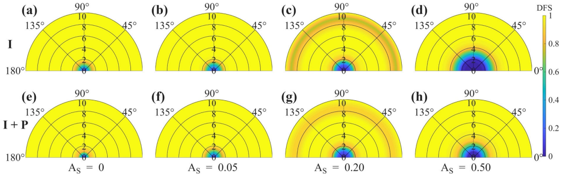
Fig. 2. Comparison of ALH-DFS distributions under different combinations of observational information ( I vs. I+P ) and surface reflectance conditions. The DFS values were calculated by varying ALH (radial axis: 0–10 km) and RAA (angular axis: 0–180°), while other parameters were fixed at with VZA = 0^\circ , SZA = 40^\circ , and AOD = 0.3 . The top row shows DFS calculated using radiance ( I ) only, while the bottom row shows DFS obtained by combining radiance and polarization information ( I+P ). Columns correspond to different surface reflectance values ( A_s = 0.00, 0.05, 0.20, 0.50 ).
