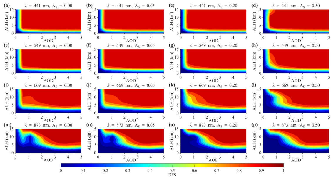
Fig. 1. Characteristics of ALH-AOD 441 -DFS distributions derived from radiance under different spectral bands and surface reflectance conditions. The simulations were conducted for smoke aerosols, with AOD 441 ranging from 0 to 5 as the common reference aerosol loading parameter. For all subplots, the x-axis represents AOD 441 . Rows correspond to wavelengths of 441 nm, 549 nm, 669 nm, and 873 nm, respectively, while columns represent different surface reflectance conditions ( A_s = 0.00, 0.05, 0.20, 0.50 ). Colors indicate the DFS values of ALH, ranging from 0 to 1.
