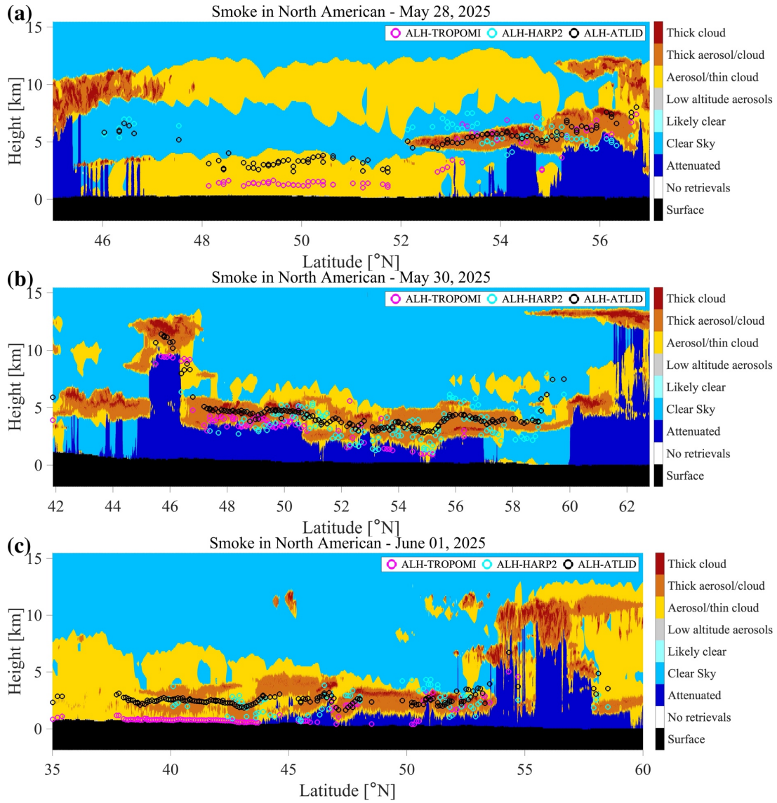
Fig. 9. Comparison of ALH-HARP2 and ALH-TROPOMI with the corresponding ATLID measurements for smoke cases on the feature classification curtain plot. Panels (a)-(c) present comparisons of ALH-HARP2 and ALH-TROPOMI with ATLID in three smoke cases, respectively.
