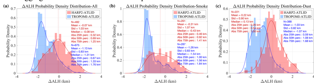
Fig. 14. Histograms and statistical metrics of the differences between ALH-HARP2, ALH-TROPOMI, and ATLID observations at the co-located are presented. The statistics include the total
