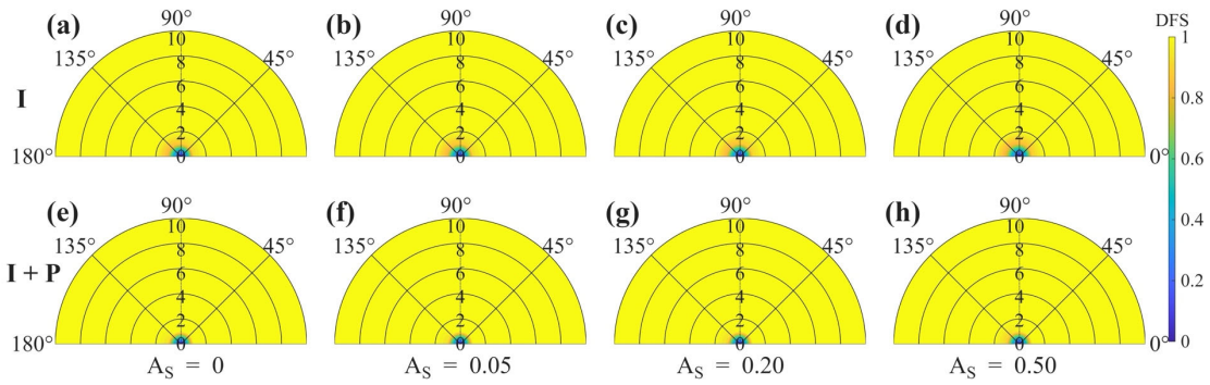
Fig. 6. Same as Fig. 2, but with VZA = 80°.
