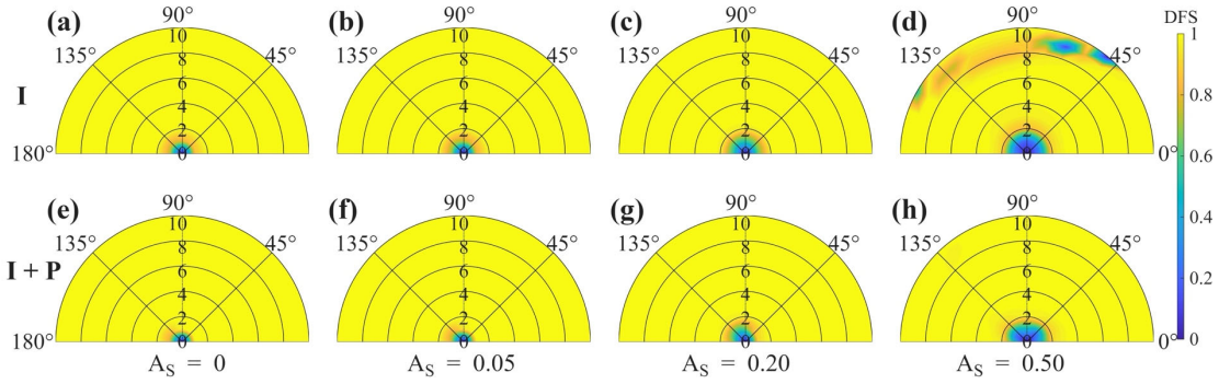
Fig. 5. Same as Fig. 2, but with VZA = 60°
