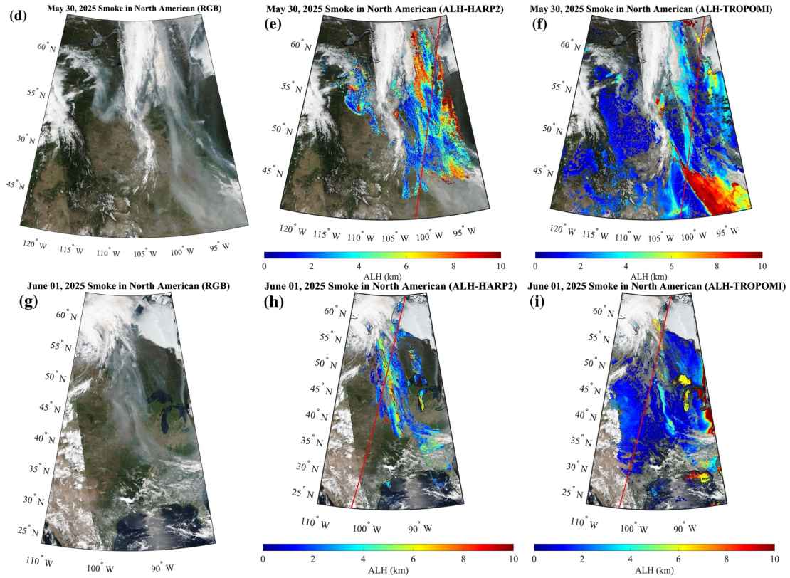
Fig. 8. Examples of retrieval for smoke cases. The first column presents the corresponding true-color images from VIIRS/Suomi-NPP. The second column displays the HARP2 -derived ALH relative to sea level with the red line representing the EarthCARE track. The third column presents the TROPOMI Level 2 ALH product.
