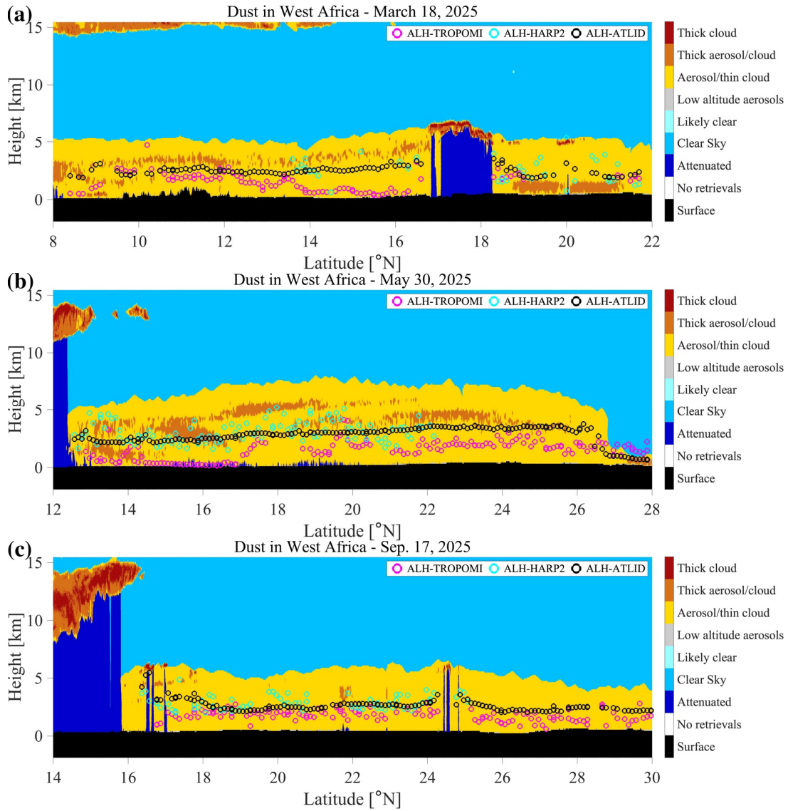
Fig. 11. Comparison of ALH-HARP2 and ALH-TROPOMI with the corresponding ATLID measurements for dust cases on the feature classification curtain plot. Panels (a)-(c) present comparisons of ALH-HARP2 and ALH-TROPOMI with ATLID in three dust cases, respectively.
