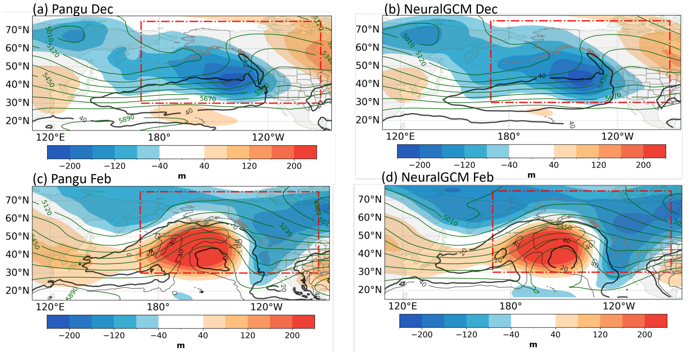
Figure A3. Same as Fig. 1 (b, d), but showing model replay with (a, c) Pangu-Weather and (b, d) NeuralGCM.
