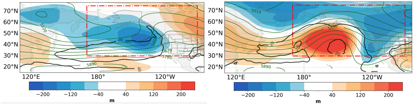
Figure A1. Same as Fig. 1 (b, d), but showing NeuralGCM replay with the fixed SST forcing for Case 1 (Left) and Case 2 (Right).
