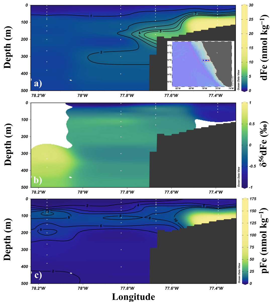
Figure S1. GEOTRACES P16 transects of a) dFe, b) \delta^{56}\text{dFe} , and c) pFe. Data are from GEOTRACES Intermediate Data Product 2025 (GEOTRACES IDP, 2025). The diagram was produced using Ocean Data View (Schlitzer, 2023).
