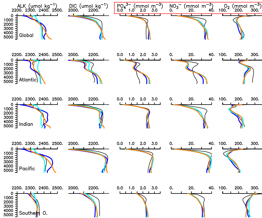
Figure 7. Biogeochemical tracer profiles for the optimal parameter sets (BL; dark blue, TID; light blue, CON; orange) of the online simulations. Black lines are observations (Key et al., 2004; Garcia et al., 2010a, b). The red box highlights the profiles targeted for calibration.
