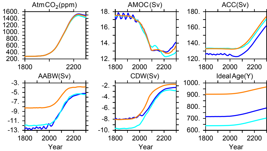
Figure 10. Global physical response to CO 2 emissions forcing for all three calibrated models. Dark blue is BL, light blue is TID, orange is CON.
