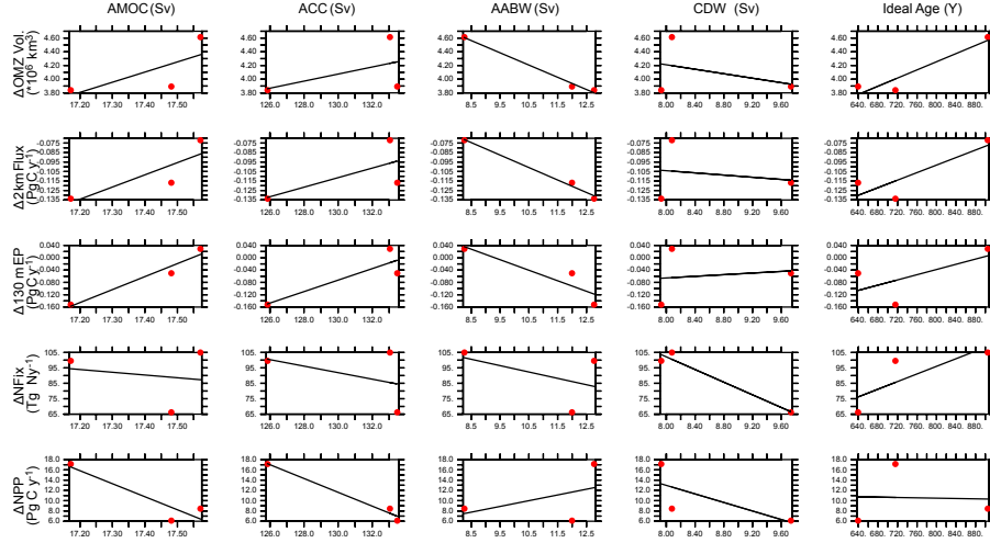
Figure A3. Calibrated model pre-industrial physical metrics (x axes) versus biogeochemical response (Year 2300-1765) metrics (y axes); red dots. Linear regression lines; black line.
