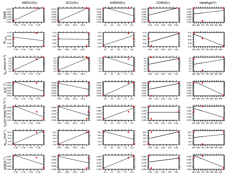
Figure A1. Calibrated model pre-industrial physical metrics (x axes) versus optimal biogeochemical parameter value or minimum calibration misfit (y axes); red dots. Linear regression lines; black line.
