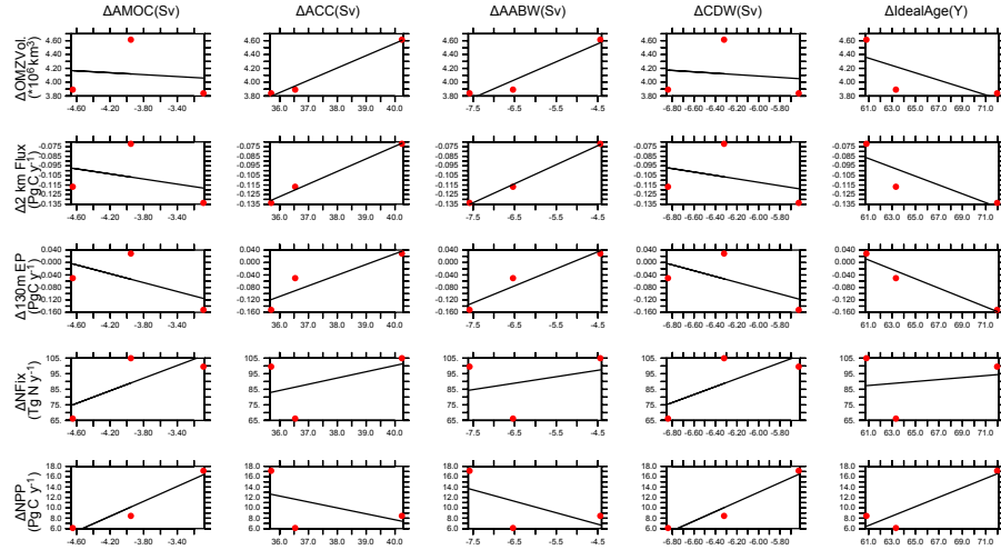
Figure A4. Calibrated model physical response (Year 2300-1765) metrics (x axes) versus biogeochemical response (Year 2300-1765) metrics (y axes); red dots. Linear regression lines; black line.
