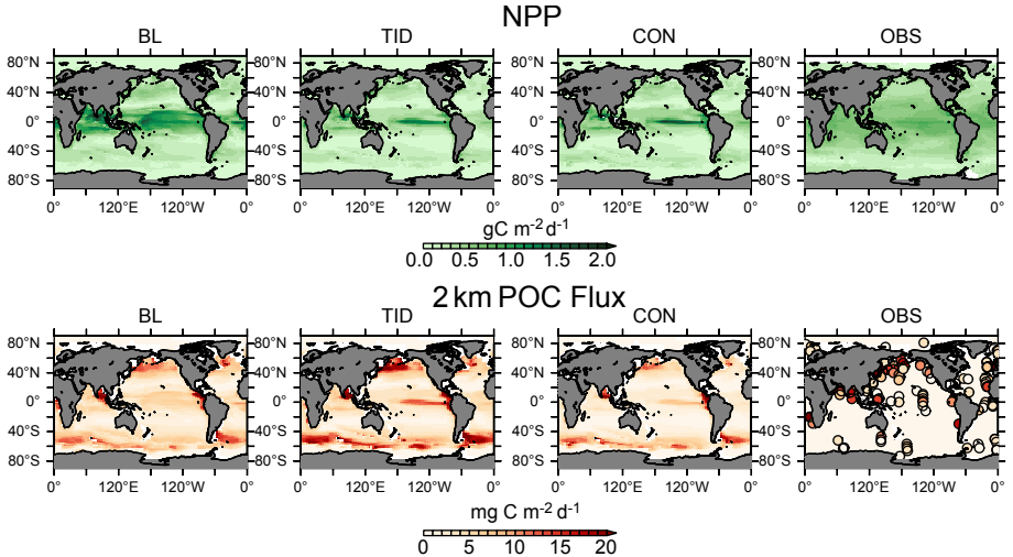
Figure 8. Top: Annual average pre-industrial depth-integrated net primary production (NPP) for all three calibrated models. Bottom: Annual average pre-industrial deep particulate organic carbon (POC) flux at 2 km depth for all three calibrated models. Observations are satellite-derived NPP climatology (2012-2018) (NASA, 2018), and 2 km depth sediment trap data (Honjo et al., 2008).
