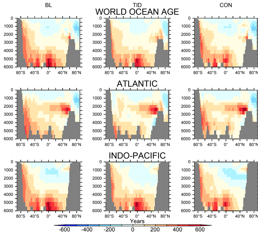
Figure 11. Change in ideal age (years 2300-1765) for the three vertical mixing schemes (BL, TID, CON).
