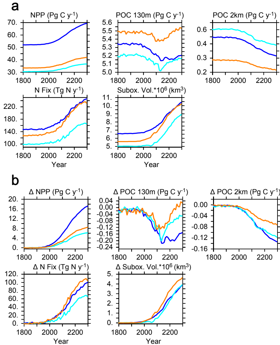
Figure 12. Panel A: Global biogeochemical metrics for all three calibrated models. Suboxic volume is calculated using a 5 mmol O 2 m -3 threshold. Panel B: Global biogeochemical response to CO 2 emissions forcing for all three calibrated models (Δ, year - pre-industrial value). Dark blue is BL, light blue is TID, orange is CON.
