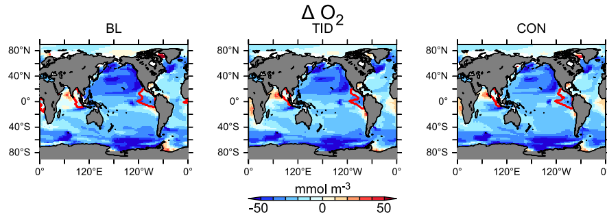
Figure 15. Change in oxygen concentration at 300 m depth (years 2300-1765) for all three calibrated models. Regions where concentrations are below 5 mmol O 2 m -3 at year 2300 are delineated in red to highlight regions in which denitrification occurs.
