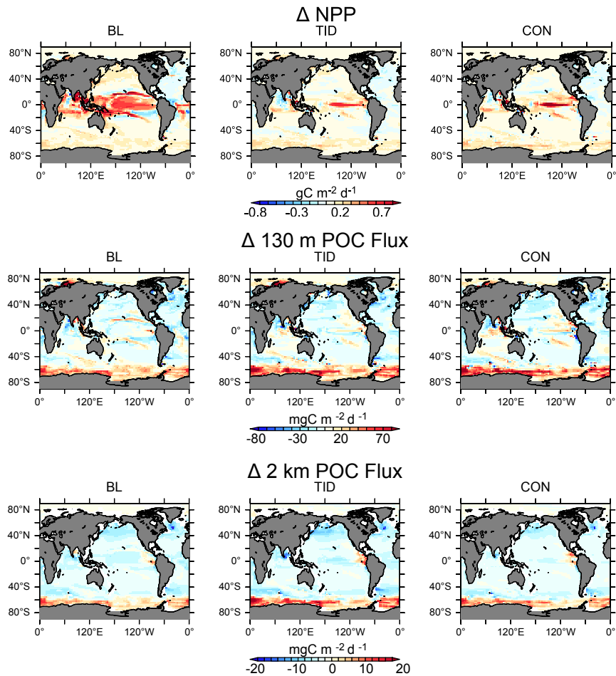
Figure 13. Top: Change in annually averaged depth-integrated net primary production (NPP, years 2300-1765) for the three calibrated models. Middle: Change (years 2300-1765) in annually averaged POC flux at 130 m depth. Bottom: Change in deep POC flux at 2 km depth.
