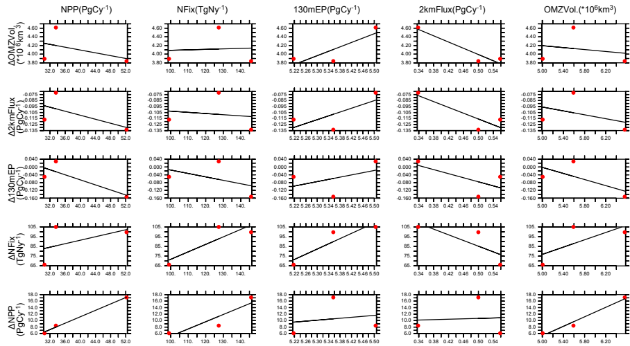
Figure A5. Calibrated model pre-industrial biogeochemical metrics (x axes) versus biogeochemical response (Year 2300-1765) metrics (y axes); red dots. Linear regression lines; black line.
