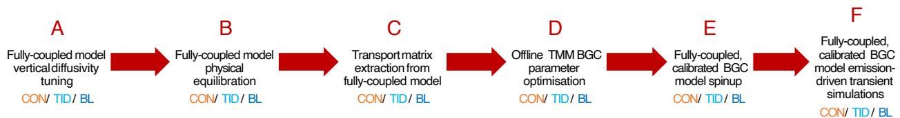
Figure 1. Work flow used in the model set-up and simulations. CON, TID, and BL stand for constant, tidal, and Bryan-Lewis vertical mixing schemes, respectively.
