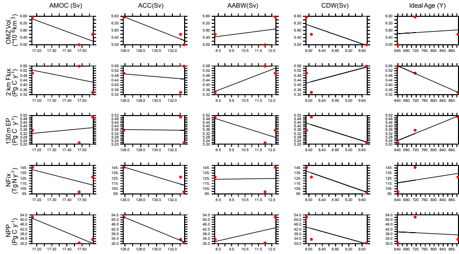
Figure A2. Calibrated model pre-industrial physical metrics (x axes) versus pre-industrial biogeochemical metrics (y axes); red dots. Linear regression lines; black line.
