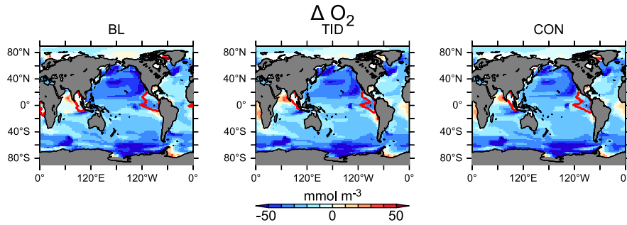
Figure 15. Change in oxygen concentration at 300 m depth (years 2300-1765) for all three calibrated models. Regions where concentrations are below 5 mmol O 2 m -3 at year 2300 are delineated in red to highlight regions in which denitrification occurs.
