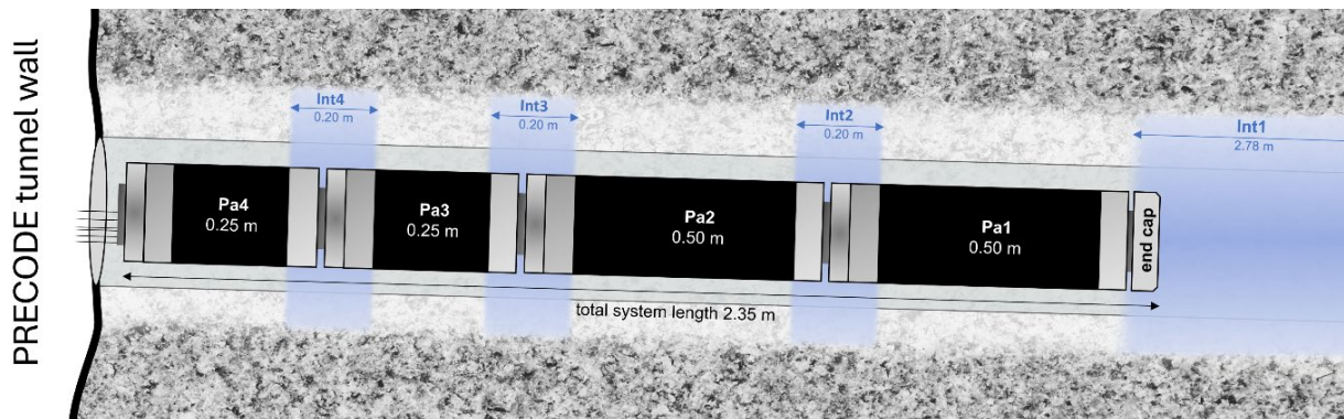
682 Figure 8: Schematic illustration of the modular multi-packer system (MMPS) installed in boreholes 683 BPR_B_10 and BPR_B_11. The configuration is identical for both boreholes. Packer sleeve lengths (Pa1- 684 Pa4) and the resulting hydraulically isolated test intervals are indicated (Int1-Int4)
