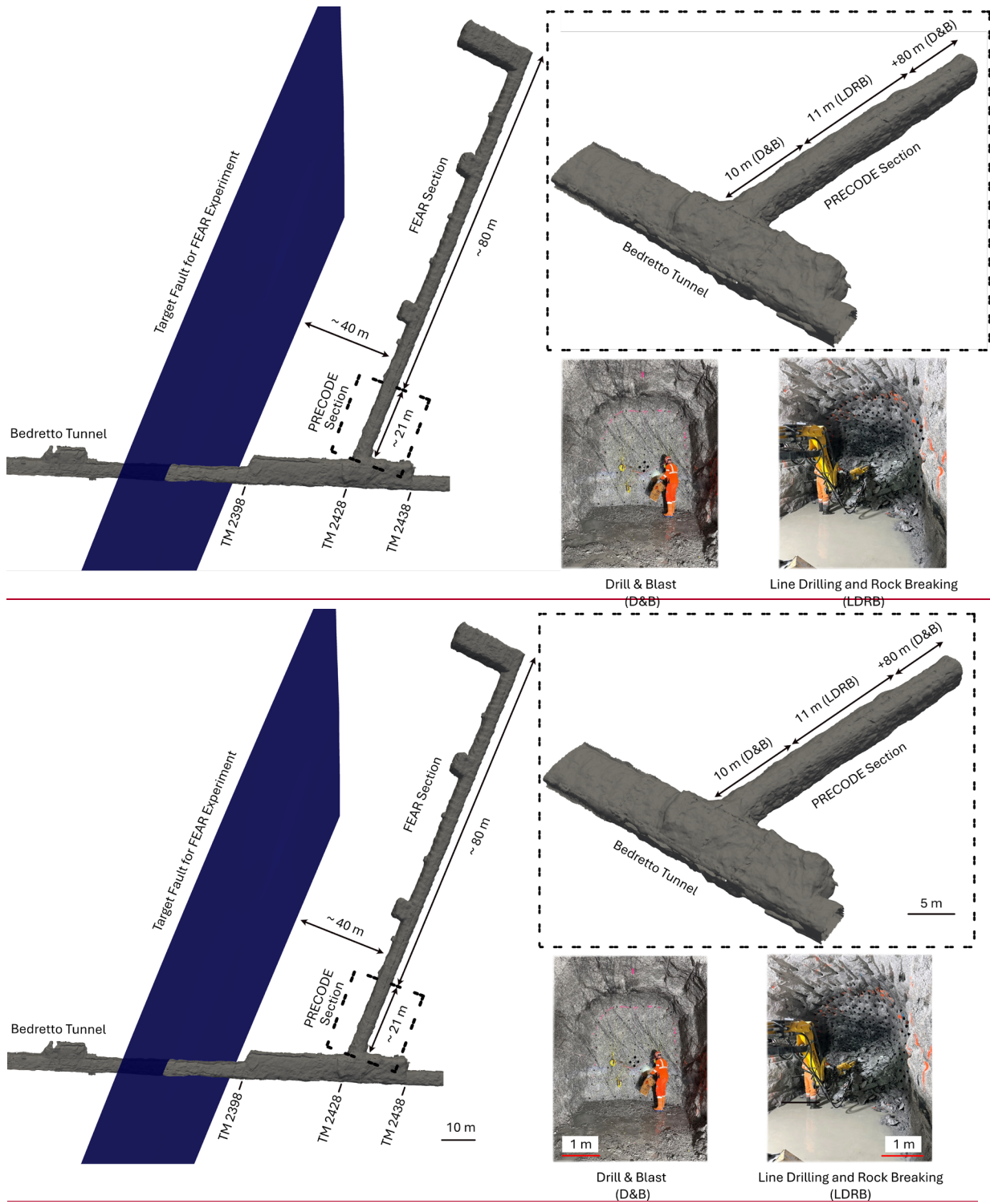
Figure 4: Left: Isometric view of the Bedretto Tunnel and the newly-excavated PRECODE/FEAR Tunnel, Right: As-built geometry of the PRECODE Section, showing D&B and LDRB sections
