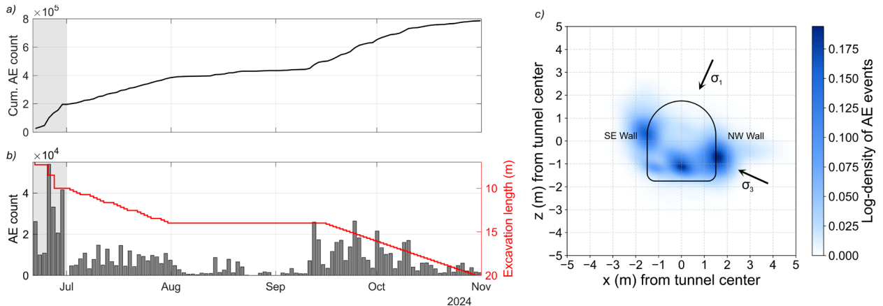
Figure 11: AE monitoring during PRECODE tunnel excavation: a) cumulative AE count during PRECODE excavation (shaded area indicates drill and blast excavation); b) AE count during PRECODE tunnel excavation with excavation lengths marked as red solid line; c) Log-density of AE events registered during the PRECODE tunnel excavation in an x-z plane. The ideal tunnel geometry is marked for reference.
