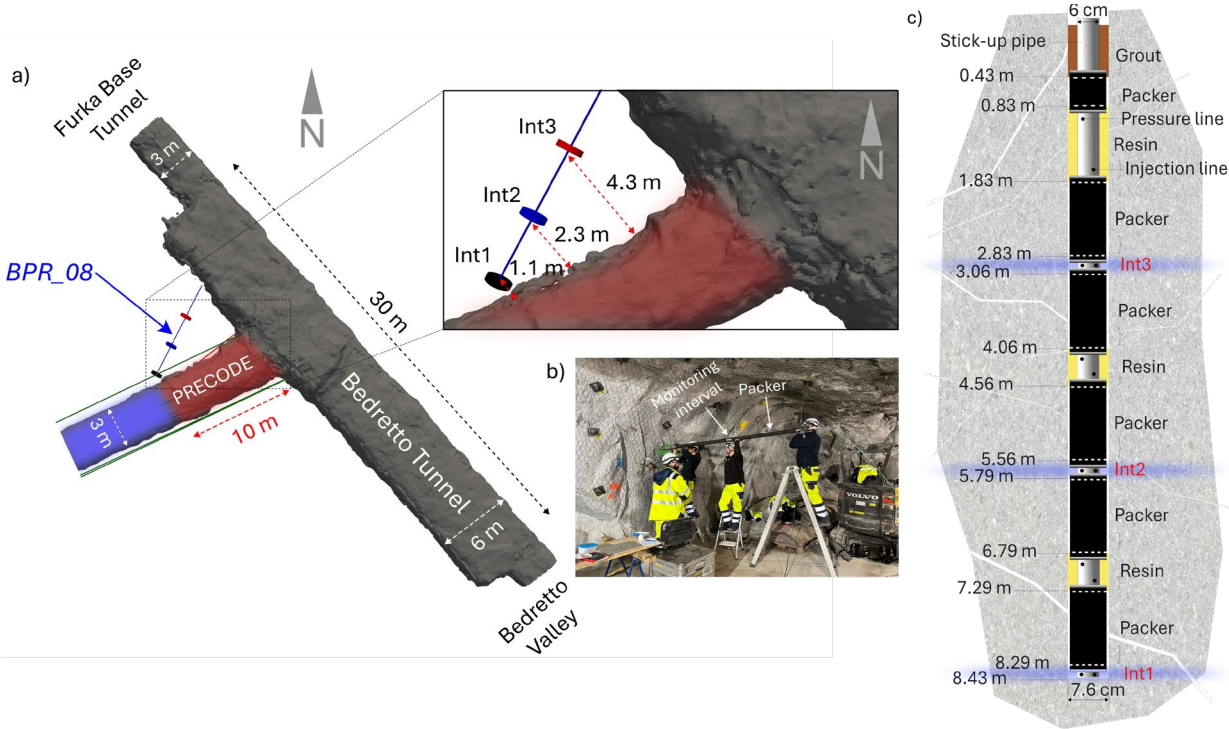
Figure 7: a) Instrumentation of the BPR_08 pressure monitoring borehole during the PRECODE experiment; b) an image of the packer system during installation, c) the detail of the three monitoring intervals
