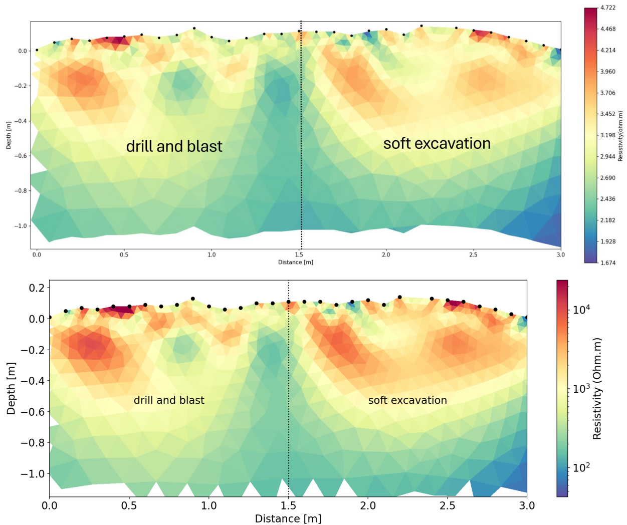
Figure 14: Inversion results for electrical resistivity tomography spanning the drill and blast, and soft excavation zones. The results show some prominent very high resistivity zones in the shallow few centimeters, likely resulting from loose slabs of rock along the wall. The information at depth reveals a higher resistivity zone for the soft excavation, suggesting more intact rock compared to the drill and blast zone.
