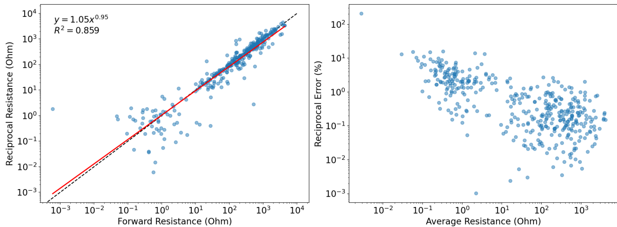
Figure 13: The left-length panel shows a comparison of forward and reciprocal electrical resistivity measurements for the profile under examination, alongside the perfect match line. The forward and reciprocal measurements overlap well, especially for high resistivities, suggesting high precision. The right-right panel shows the reciprocal error compared to the average resistance for the measurements. Reciprocal errors above 10% are not included in the data inversion.
