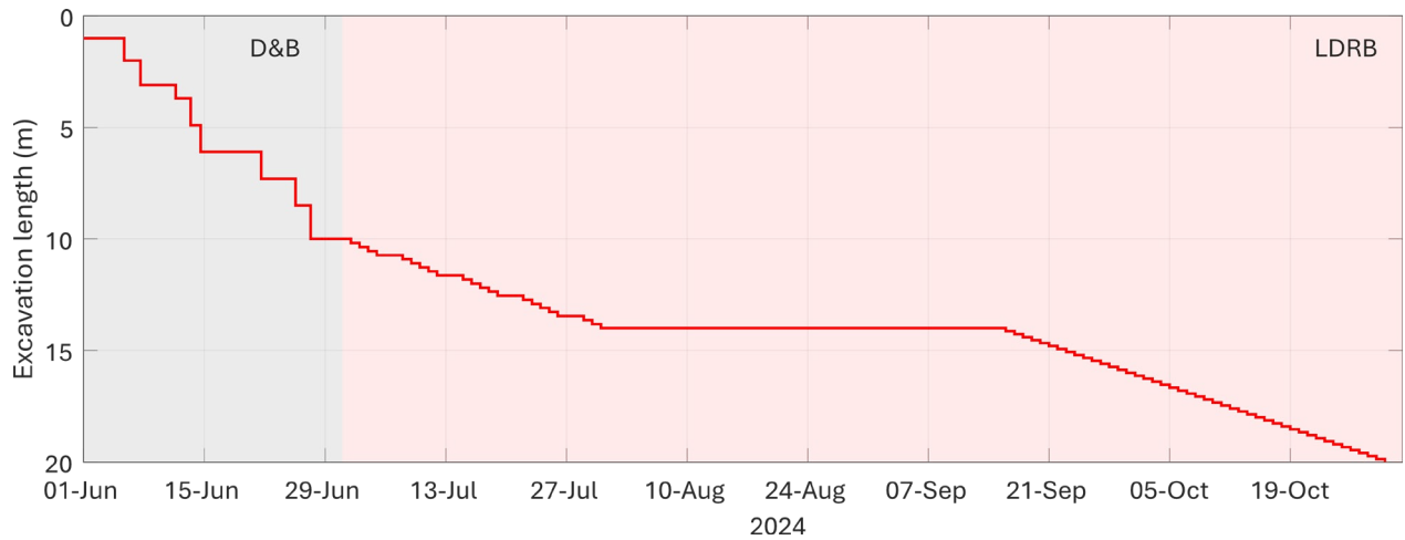
Figure 5: Excavation advancement for the PRECODE section
