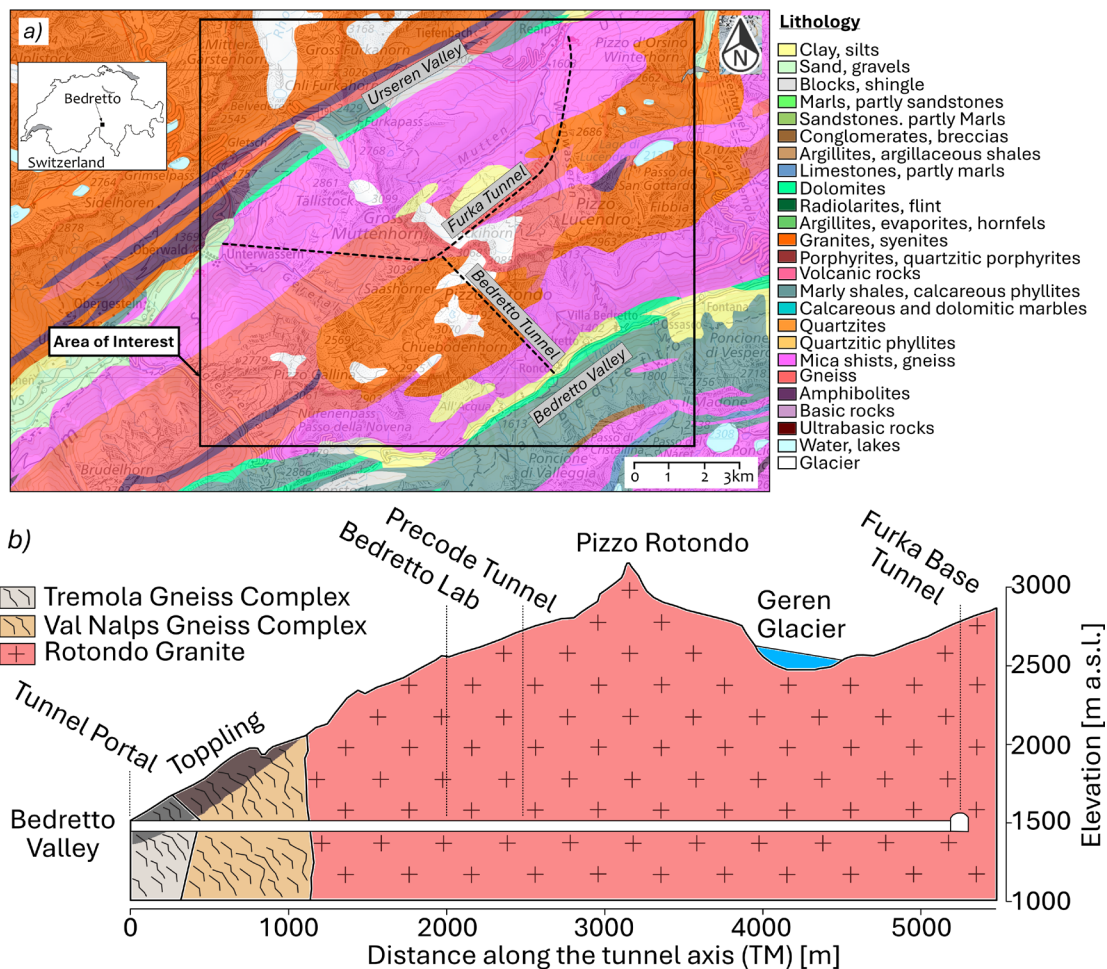
Figure 3: a) Lithology of the Bedretto Valley and surrounding area (source: SwissTopo), b) cross section along Bedretto Tunnel, with highlighted location of BedrettoLab and PRECODE Tunnel (modified after Keller & Schneider, 1982)
