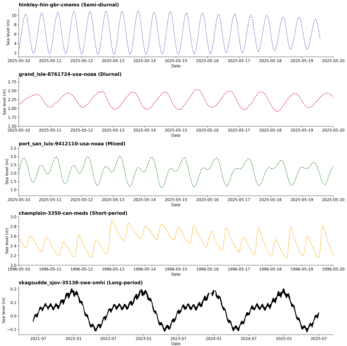
Figure B2. Time series of tide gauge data within each tidal band, as discussed in Figure 4. For the long-period example, non-tidal variability has been removed to highlight only the tidal contributions.
