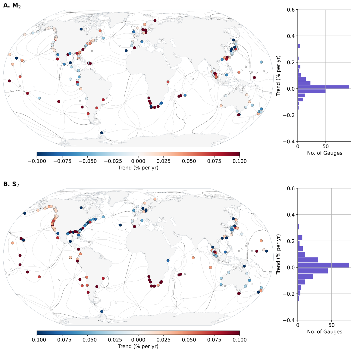
Figure 8. M_2 and S_2 amplitude percentage trend derived from UHSLC research quality tide gauges with at least 30 years of observations. The black contour lines are the phase lag of the respective constituents obtained from FES2022.
