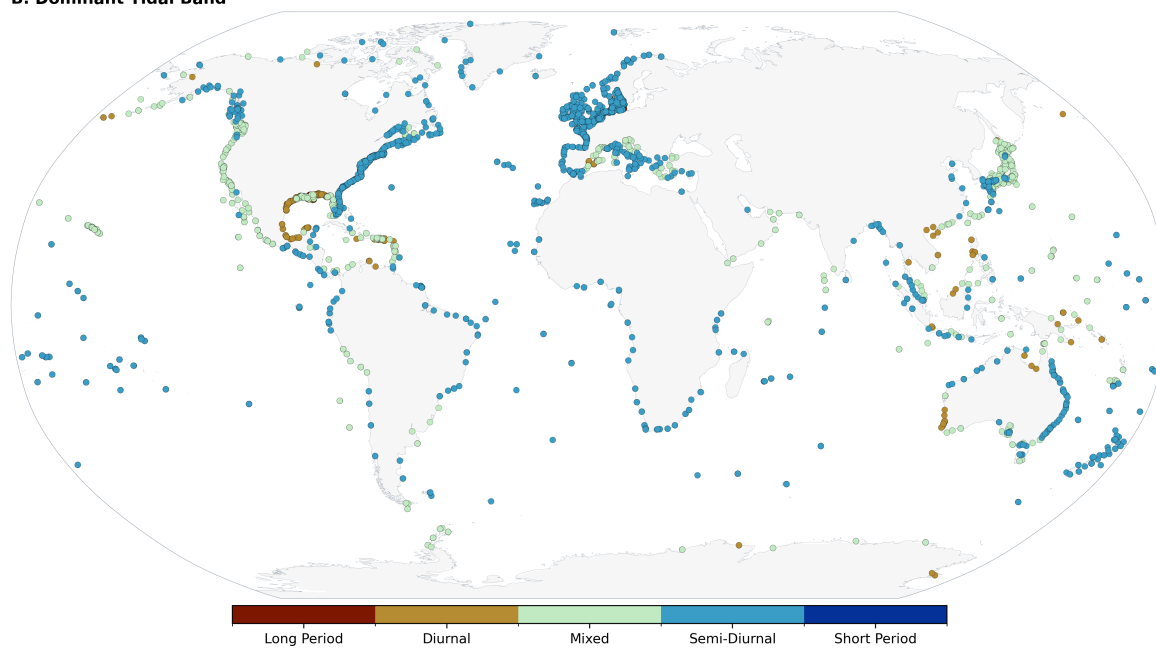
Figure 4. The tidal range and dominant tidal band for each tide gauge in GESLA-4. In Figure B2, examples are shown of tide gauges in each tidal band.
