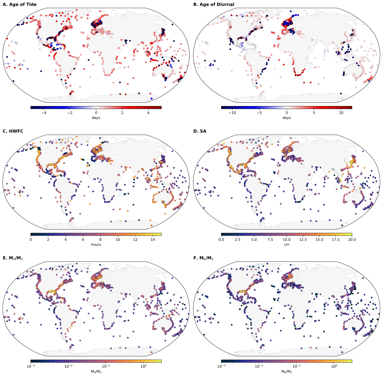
Figure 6. Age of Tide, Age of Diurnal tide, HWFC, Solar Annual (Sa) constituent, ratio of M_4/M_2 , and ratio of M_6/M_2 . A selection of these results is shown for the FES2022 model in Figure B3.
