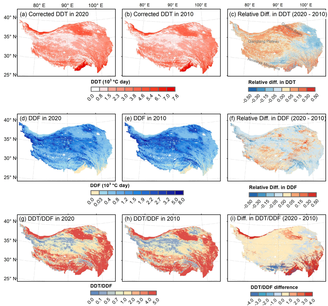
Figure 3 Spatial distribution and decadal changes of thermal forcing indices on the QTP. (a-e) displays the ground surface thawing index (and decadal change of (a-c) DDT), and its relative changes, (d-f) the freezing index, DDF and its relative changes. (g-i) the ratio of thawing to freezing indices. Left column shows the distributions in (DDT/DDF) and its decadal change. The left and middle columns present the spatial distribution for the 2020, middle column shows the distributions in period and 2010, and the period, respectively. The right column shows their decadal differences between 2020 and 2010. The relative differences in (c) and (f) are calculated using baseline denominators of 2000^{\circ}\text{C}\cdot\text{d} and 1200^{\circ}\text{C}\cdot\text{d} , respectively, which are the regional mean values of DDT and DDF averaged across both periods. For panels (c) and (i), positive values (red) indicate warming/instability, while negative values (blue) indicate cooling/stability. For panel (f), negative values (red) indicate winter warming (reduced freezing), while positive values (blue) indicate cooling.
