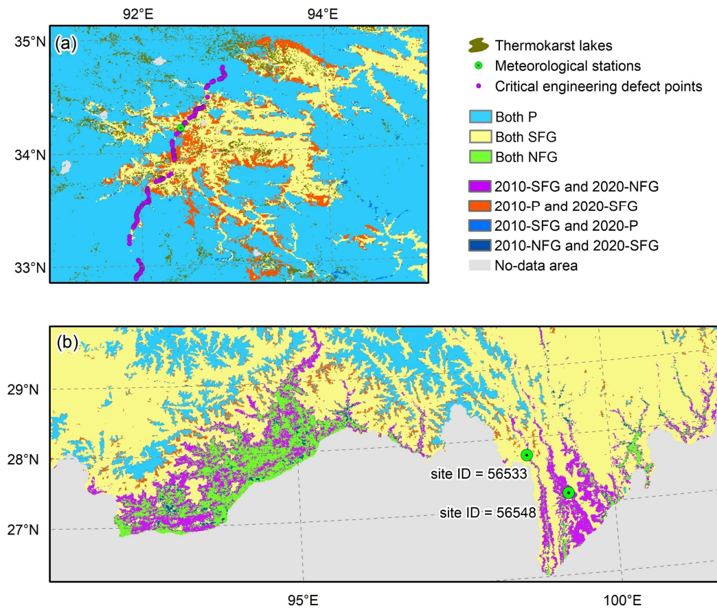
Figure 11 Distribution and changes of frozen ground types in two degradation hotspots on the QTP from 2010 to 2020 periods .
