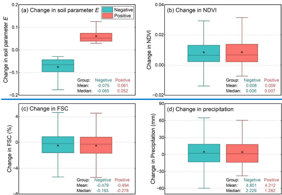
420 Figure 5 Distribution of decadal changes (2010–2020) in key environmental factors, categorized by the trend in soil parameter E . Boxplots compare changes in (a) soil parameter E , (b) NDVI, (c) FSC and (d) precipitation between regions of increased risk (positive group) and reduced risk (negative group). In each box plot, the center line shows the median, the box represents the lower and upper quartiles (25th–75th percentiles), and the whiskers extend to the furthest data points within 1.5 times the interquartile range. The ‘x’ marks the mean.
