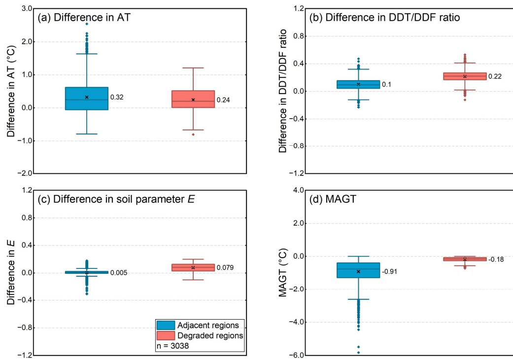
Figure 12 Comparison of key environmental variables between degraded regions (permafrost to SFG) and adjacent stable permafrost regions in subregion aA of Fig. 10b9b (Central QTP). The boxplots compare decadal changes (2010-2020) in (a) air temperature (AT), (b) the DDT/DDF ratio, and (c) the soil parameter E . For the changes shown in panels (a-c), positive values indicate an increase over the decade, while negative values indicate a decrease. Panel (d) compares the mean annual ground temperature (MAGT) in 2010-2019. In each box plot, the center line shows the median, the 'x' marks the mean, the box represents the lower and upper quartiles (25th-75th percentiles), and the whiskers extend to the furthest data points within 1.5 times the interquartile range. Data points beyond the whiskers are plotted individually as outliers.
