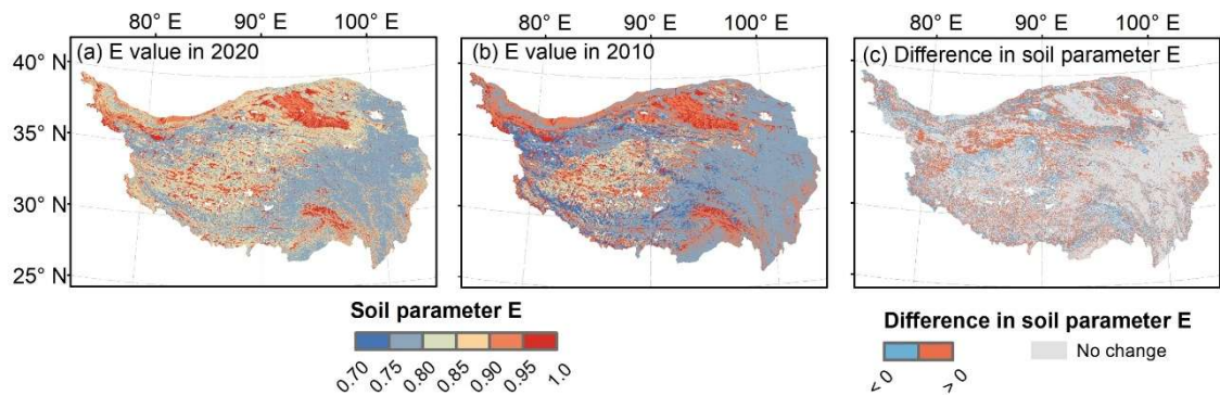
Figure 4 Spatial distribution of the soil parameter E in the 2020 period (a) and 2010 (b). (c) illustrates the difference (2020 minus 2010), where positive values (red) indicate an increase in E (conditions conducive to degradation) and negative values (blue) indicate a decrease. The 2010 E map was derived from Cao et al. (2023), whereas the 2020-period E map was predicted using a space-for-time substitution strategy.
