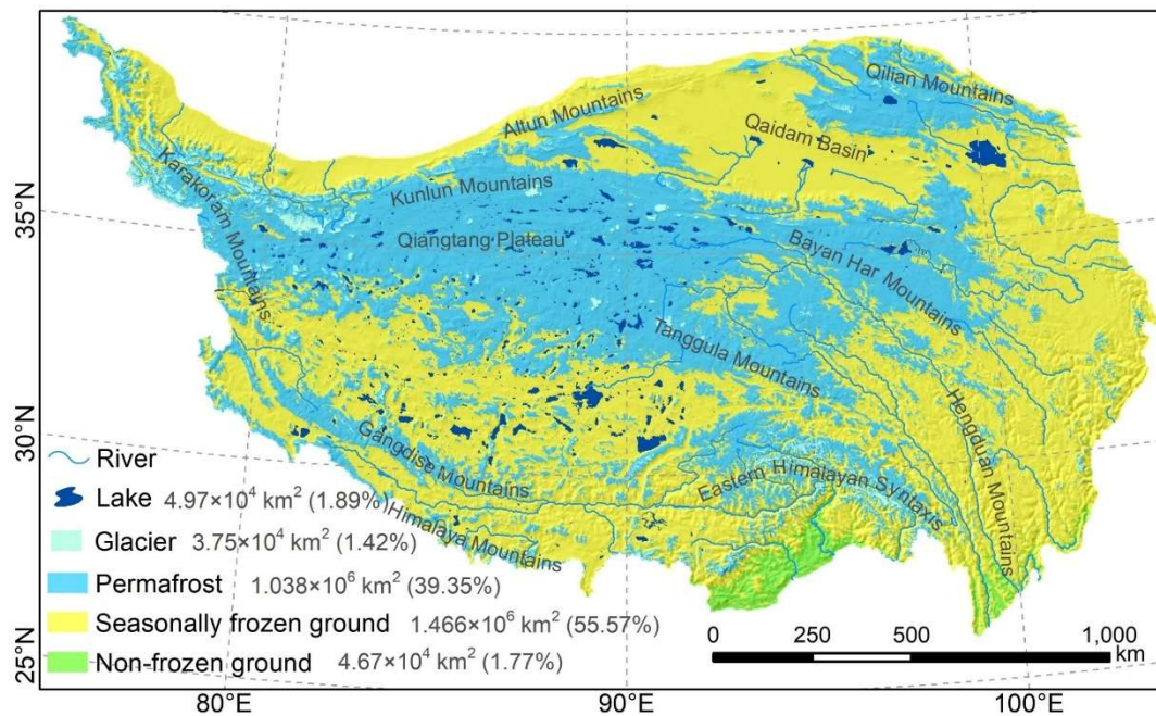
Figure 65 Map of frozen ground distribution at 1 km resolution over the QTP in the 2020 period. Areas and percentages of frozen soil types are present. Glacier extent data are derived from Ye et al. (2017), and the 2020 lake boundaries are obtained from Zhang et al. (2021).
