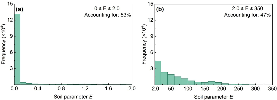
820 Figure B1. Frequency histograms of the soil parameter E predicted by the MLP model. (a) Distribution of values within the range of 0 \leq E \leq 2.0 , accounting for 53% of total pixels. (b) Distribution of values within the range of 2.0 \leq E \leq 350 , accounting for the remaining 47%.
