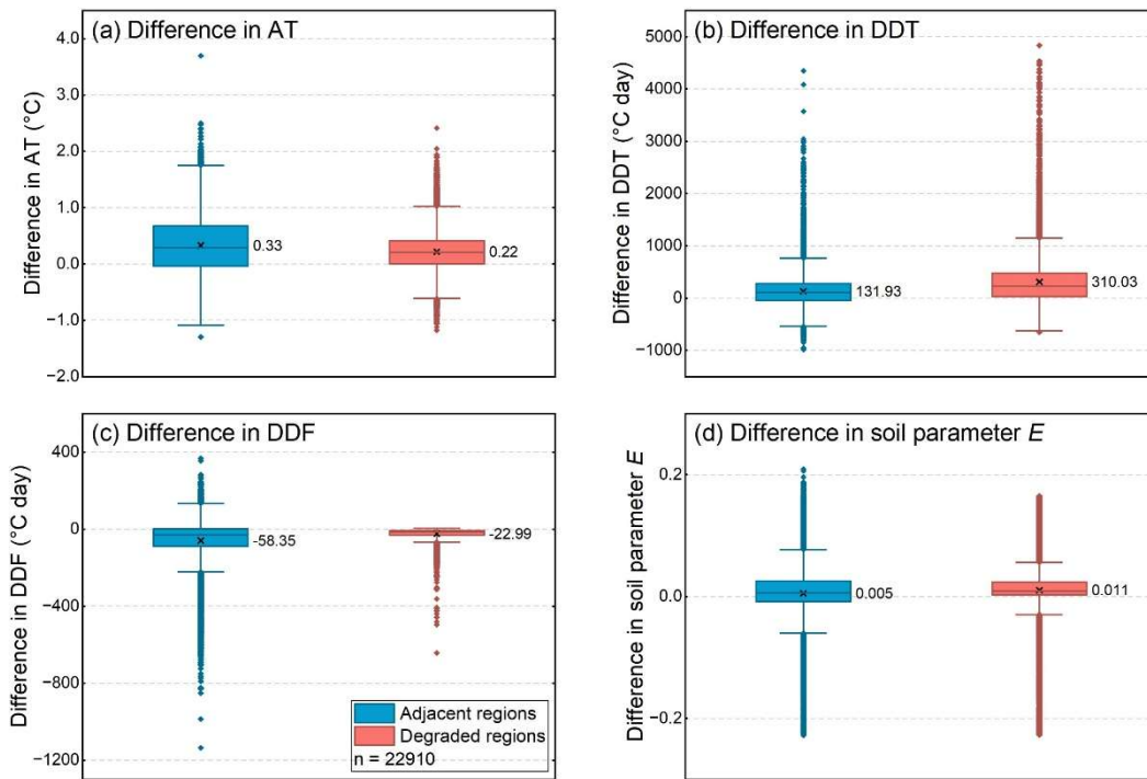
Figure 13 Comparison of key environmental variables between degraded regions (SFG to non-frozen ground) and adjacent SFG regions in subregion bB of Fig. 10b9b (Southern QTP). The panels compare decadal changes in (a) air temperature (AT), (b) DDT , (c) DDF , and (d) the soil parameter E . Positive values indicate an increase over the decade, while negative values indicate a decrease. In each box plot, the centre line shows the median, the 'x' marks the mean, the box represents the lower and upper quartiles (25th-75th percentiles), and whiskers extend to the furthest data points within 1.5 times the interquartile range. Data points beyond the whiskers are plotted individually as outliers.
