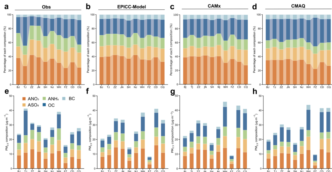
Figure 6. Comparison of simulated and observed aerosol components in representative Chinese cities. \text{ASO}_4 , \text{ANO}_3 , \text{ANH}_4 , \text{OC} , and \text{BC} denote sulfate, nitrate, ammonium, organic carbon, and black carbon in \text{PM}_{2.5} , respectively. The locations of monitoring sites are as follows: BJ (Beijing; 116.41^\circ \text{E} , 40.04^\circ \text{N} ), TJ (Tianjin; 117.21^\circ \text{E} , 39.17^\circ \text{N} ), ZZ (Zhengzhou; 113.73^\circ \text{E} , 34.77^\circ \text{N} ), JN (Jinan; 117.06^\circ \text{E} , 36.66^\circ \text{N} ), SH (Shanghai; 121.53^\circ \text{E} , 31.23^\circ \text{N} ), NJ (Nanjing; 118.76^\circ \text{E} , 32.07^\circ \text{N} ), WH (Wuhan; 114.37^\circ \text{E} , 30.54^\circ \text{N} ), FZ (Fuzhou; 119.31^\circ \text{E} , 26.10^\circ \text{N} ), CD (Chengdu; 104.09^\circ \text{E} , 30.64^\circ \text{N} ), and CQ (Chongqing; 106.47^\circ \text{E} , 29.62^\circ \text{N} ).
