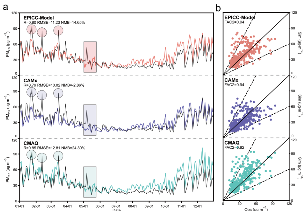
Figure 1. Comparison of simulated and observed daily PM_{2.5} concentrations (i.e., daily mean PM_{2.5} concentrations) across China in 2021. (a) shows the time series of daily PM_{2.5} , with the black line representing observations from 1,644 national air quality monitoring stations and colored lines indicating different CTMs. (b) presents scatter plots of modeled versus observed PM_{2.5} . All model outputs exclude dust aerosol contributions to isolate secondary particulate formation processes.
