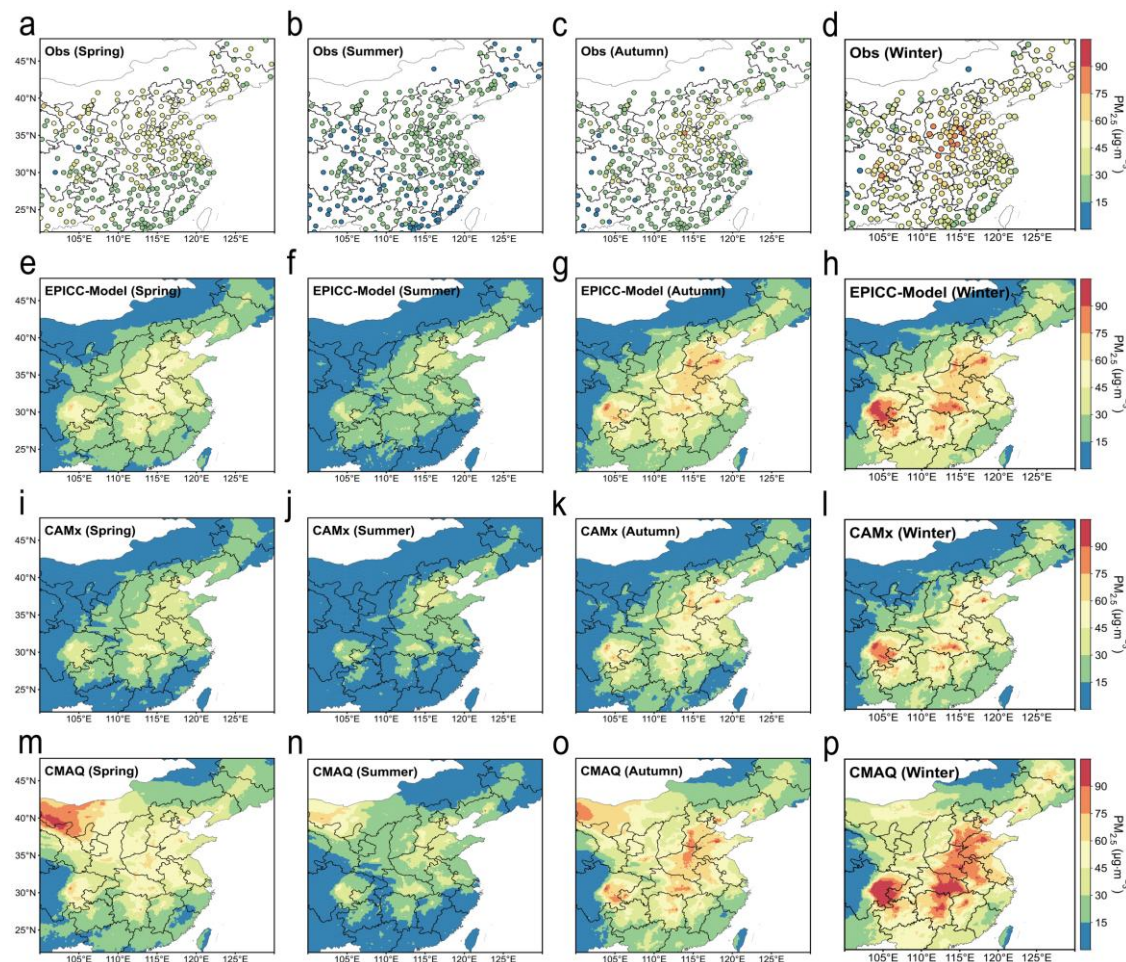
Figure 3. Seasonal spatial distributions of simulated \text{PM}_{2.5} concentrations, with spring (March-May), summer (June-August), autumn (September-November), and winter (December-February).
