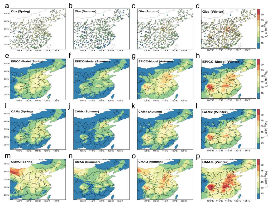
Figure 3. Seasonal spatial distributions of simulated PM 2.5 concentrations, with spring (March-May), summer (June-August), autumn (September-November), and winter (December-February).
