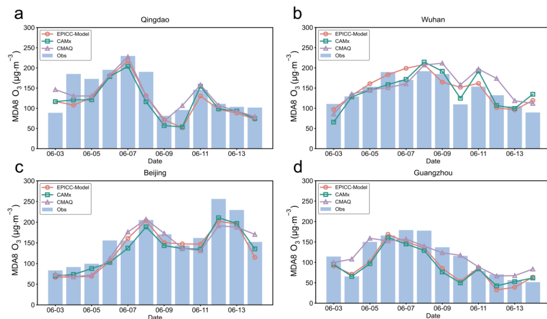
Figure 12. Time series of \text{O}_3 concentrations in key cities along the pollution belt.
