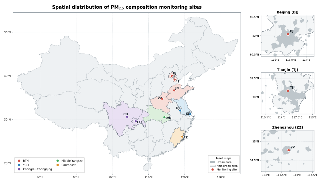
Figure R1. Spatial distribution of the ten PM 2.5 composition monitoring sites. The enlarged panels show the locations of the Beijing, Tianjin, and Zhengzhou sites relative to the mapped urban extents. Model concentrations were extracted from the grid cells containing the corresponding monitoring sites.
