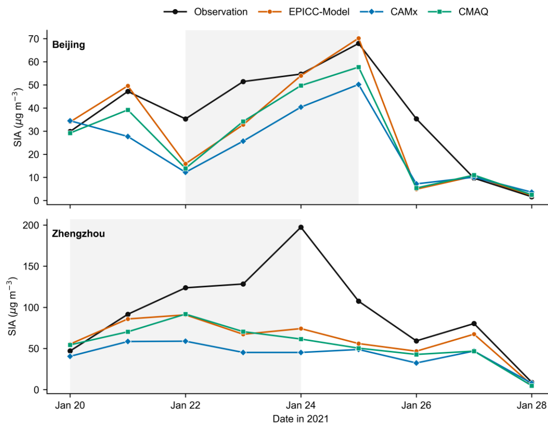
Figure R5. Observed and simulated daily SIA concentrations in Beijing and Zhengzhou during the 20-28 January 2021 \text{PM}_{2.5} episode. SIA is calculated as the sum of nitrate, sulfate, and ammonium. The shaded areas indicate the observed buildup periods used in the quantitative evaluation: 22-25 January in Beijing and 20-24 January in Zhengzhou.
