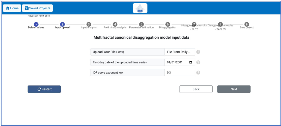
860 Figure A.8: Input interface of the Sub-hourly Disaggregation Module showing the required inputs, including the starting date of the rainfall series and the IDF scaling exponent n .
