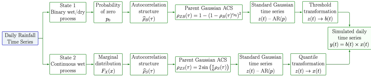
115 Figure 2: Workflow of Daily Rainfall Simulation Model. Equations details are described in the text.
