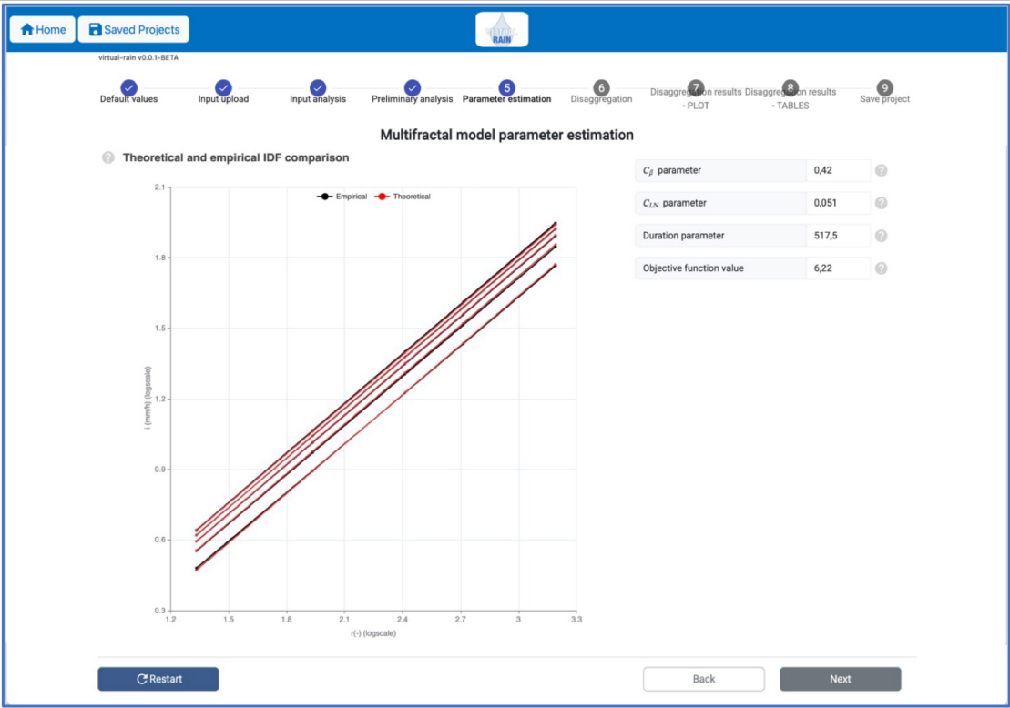
890 Figure A.11: MRC calibration interface showing the comparison between imposed and calibrated IDF curves for the selected return periods, together with the estimated MRC parameters and objective-function value.
