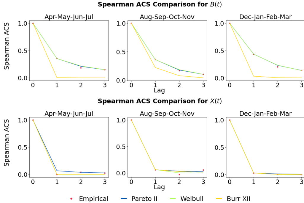
475 Figure 6: Comparison between empirical and fitted parametric ACSs for the B(t) and X(t) processes across the seasonal groups. The fitted curves are obtained by minimizing the Mean Absolute Error between empirical and theoretical Spearman ACSs.
