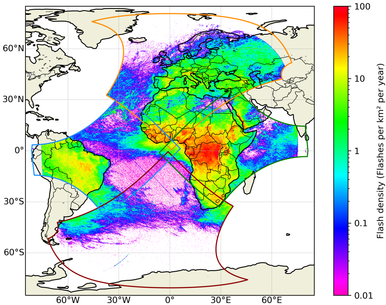
Figure 2. Spatial distribution of MTG-LI flash density (flashes km -2 y -1 ) over the full MTG-LI FOV from July 2024 to June 2025 on a 0.1° × 0.1° spatial grid.
