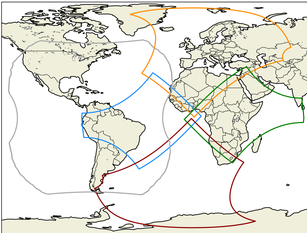
Figure 1. Field of view of GLM on GOES-East (GOES-16 and GOES-19) (gray), and of the four Sectors covered by MTG-LI cameras without considering the parallax correction effects described in the text (West in blue, North in orange, East in green, and South in red, respectively).
