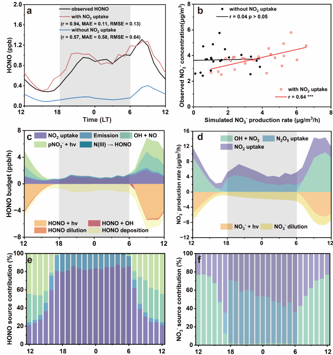
Figure 4. Quantified results from the multiphase chemical box model during SLB periods. (a) Diurnal variations in observed and simulated HONO concentrations with and without NO 2 uptake. (b) Relationship between the simulated NO 3 - production rate and observed concentration with and without NO 2 uptake. Diurnal variations of HONO (c) and NO 3 - budgets (d) during SLB days. Diurnal variations of source contributions to (e) HONO and (f) NO 3 - . The grey shaded areas represent the nighttime period.
