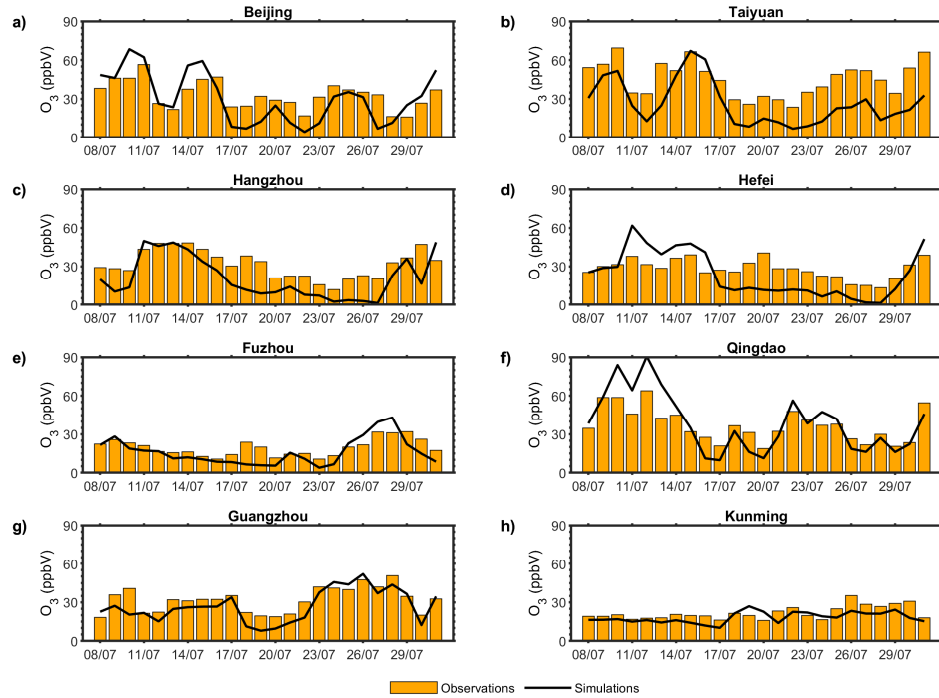
Figure 9. Time series of observed and simulated MDA8 \text{O}_3 concentrations in major cities of China from 8 to 31 July 2021. Panels (a)–(h) represent Beijing, Taiyuan, Hangzhou, Hefei, Fuzhou, Qingdao, Guangzhou, and Kunming, respectively. Time series of observed and simulated MDA8 \text{O}_3 concentrations in major cities of China on 8–31 July, 2021. Panels (a)–(h) represent Beijing, Taiyuan, Hangzhou, Hefei, Fuzhou, Qingdao, Guangzhou, and Kunming.
