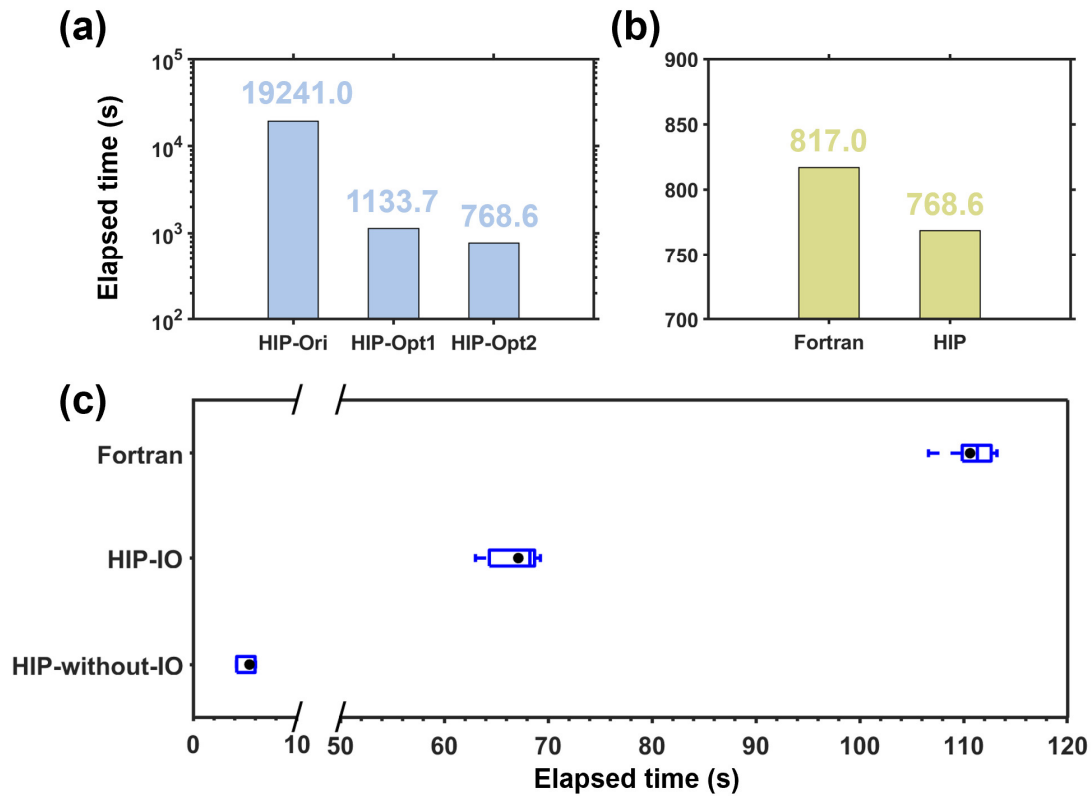
Figure 12. (a) The average hourly elapsed time required for a 28-hour simulation across the HIP-Ori, HIP-Opt1, and HIP-Opt2 versions HIP-Ori, HIP-Opt1, Opt2 versions ; (b) the average hourly elapsed time required for a 28-hour simulation between the Fortran and HIP-Opt2 versions; (c) the hourly elapsed time required for a 28-hour simulation across the original Fortran-based HADVPPM program on CPUs, the GPU-HADVPPM4HIP V1.0 with CPU-GPU data transfer, and the GPU-HADVPPM4HIP V1.0 without data transfer. The black dots represent the average values, and the
