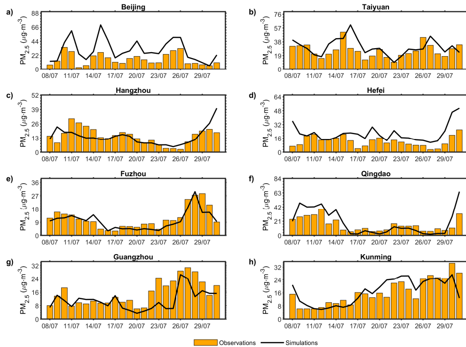
Figure 8. Time series of observed and simulated daily \text{PM}_{2.5} concentrations in major Chinese cities
