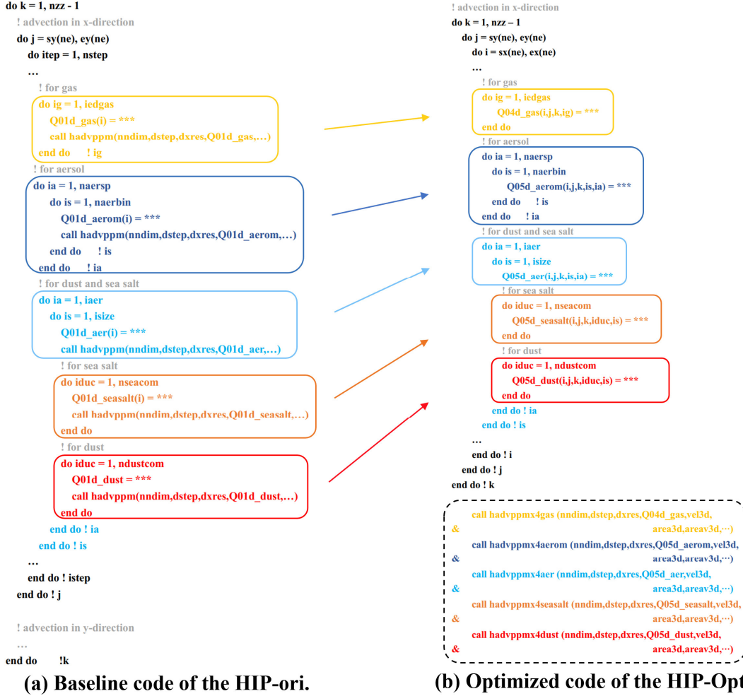
Figure 4. Code-level implementation of the CPU-GPU communication optimization. Panel (a) shows the baseline Fortran code for HIP-Ori, and panel (b) shows the optimized Fortran code for HIP-Opt1. The code-level implementation of CPU-GPU communication optimization. Panel (a) is the baseline Fortran code of the HIP-ori. Panel (b) is the optimized Fortran code of the HIP-Opt1.
