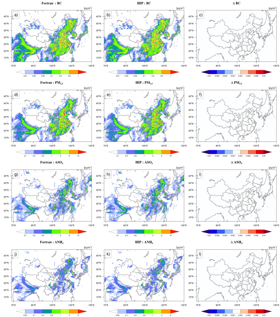
Figure 7. BC, PM 2.5 , ASO 4 , and ANH 4 concentrations outputted by the EPIC Model for the Fortran and HIP-Opt2 versions. Panels (a), (d), (g), and (j) are from the Fortran version. Panels (b), (e), (h), and (k) are from the HIP-Opt2 version. Panels (c), (f), (i), and (l) are the absolute errors (AEs) between the Fortran and HIP-Opt2 versions.
