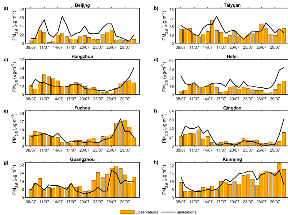
Figure 8. Time series of daily observed and simulated PM_{2.5} concentrations in major cities of China on 8-31 July, 2021. Panels (a) - (h) represent Beijing, Taiyuan, Hangzhou, Hefei, Fuzhou, Qingdao, Guangzhou, and Kunming.
