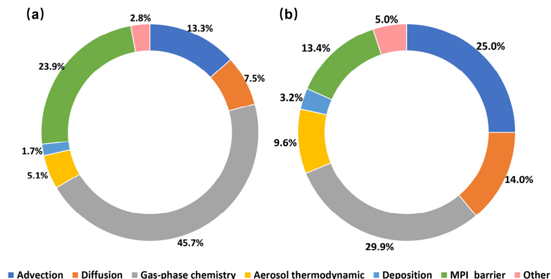
Figure 2. The computational time proportion among modules (a) for the Fortran version and (b) after implementing the gas-phase chemistry module on GPU-like accelerators for parallel computation.
