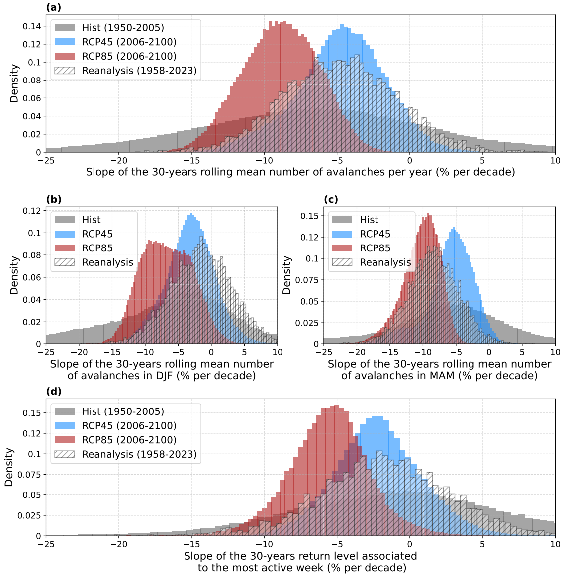
Figure A1. Distribution of the climatic trends based on ADAMONT simulations.
