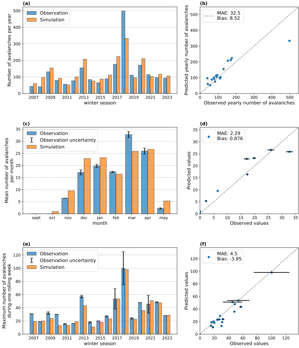
Figure 5. Evaluation of the model M_{d_1-d_2}^{2006-2023} M_{d_1-d_2}^{2007-2023} using the LOYO method on the annual number of avalanches (a, b), the mean number of avalanches per month over the 17 winter seasons (c, d), and the maximum number of avalanches during a week per winter season (e, f). The MAE and the bias are computed using the distance to the interval associated with the uncertainties (error bars on observations).
