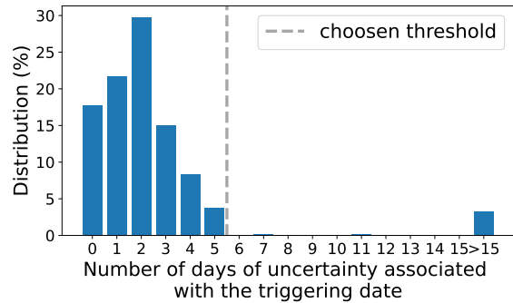
Figure 3. Distribution of the number of days of uncertainty concerning the triggering date from 2006 –winter season 2007 to 2023 in the studied area.
