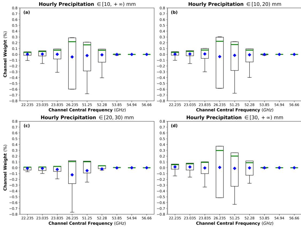
Figure 10. Boxplots of the differences in GMWR channel weights between the GWMRnMRL and GMWROnly experiments diagnosed by the adaptive observation weighting TCKF1D-Var framework. Results are shown for (a) all nocturnal heavy precipitation cases, (b) cases with hourly accumulated precipitation between 10 and 20 mm, (c) cases with hourly accumulated precipitation between 20 and 30 mm, and (d) cases with hourly accumulated precipitation exceeding 30 mm. The boxes represent the interquartile range (IQR), with the lower and upper edges corresponding to the first and third quartiles, respectively. The green horizontal lines indicate the median values, while the blue squares denote the mean values. Whiskers extend to 1.5 times the IQR, and red dots represent outliers beyond this range.
