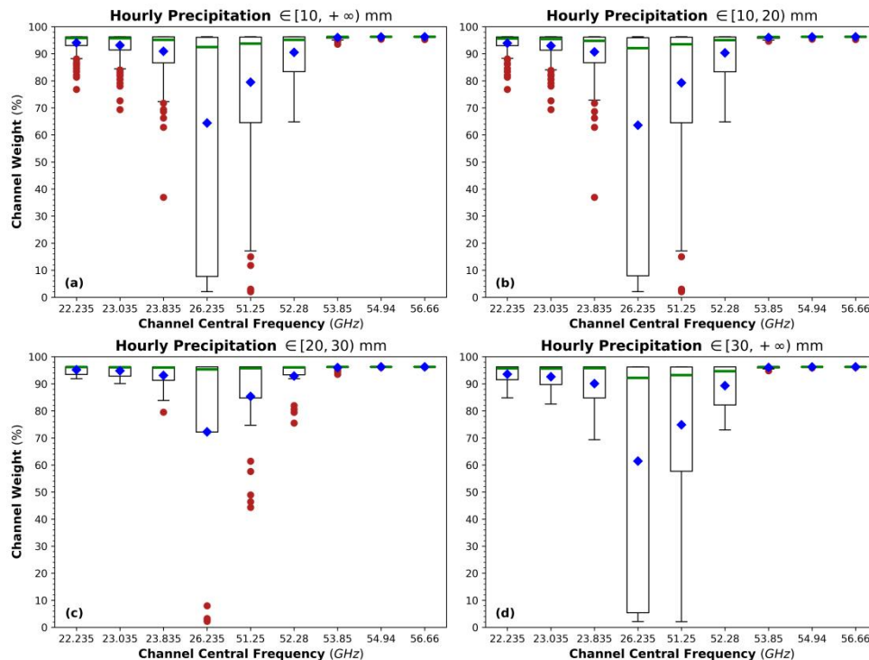
360 Figure 4. Boxplots of the adaptive observation weights assigned to the 9 GMWR channels by the adaptive observation weighting TCKF1D-Var framework. Results are shown for (a) all nocturnal heavy precipitation cases, (b) cases with hourly accumulated precipitation between 10 and 20 mm, (c) cases with hourly accumulated precipitation between 20 and 30 mm, and (d) cases with hourly accumulated precipitation exceeding 30 mm. The boxes represent the interquartile range, with the lower and upper edges
