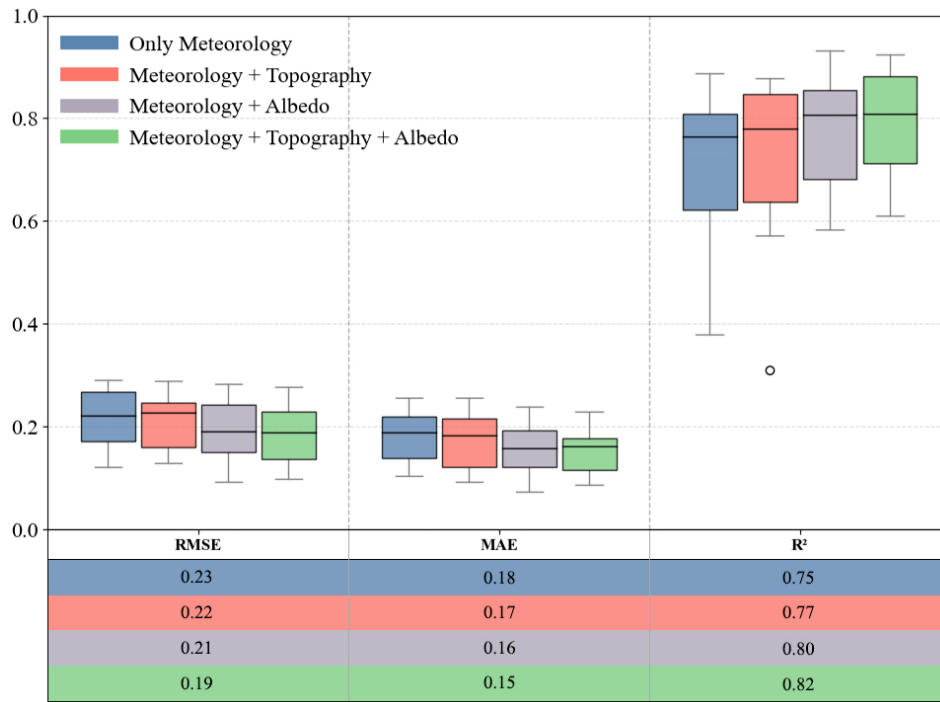
Figure 9 Comparison of FF-FCNN model performance with different input features.
