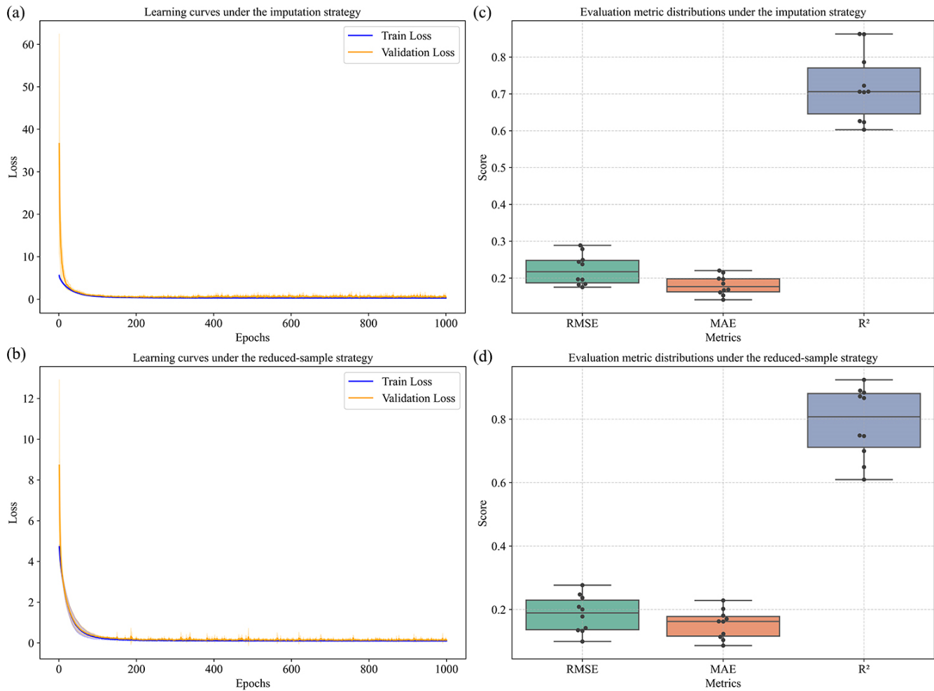
Figure 5 Assessment of overfitting risks and comparison of model performance under the two dataset construction strategies. (a)–(b) Training and validation mean loss curves with 10-fold random cross-validation. (c)–(d) Distribution of validation metrics.
