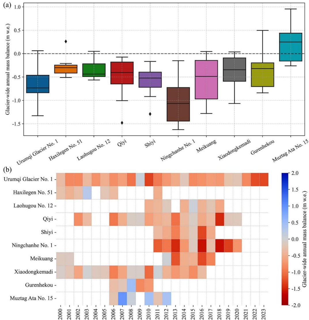
140 Figure 2 Spatiotemporal characteristics of glacier-wide annual mass balance for the ten continental-type glaciers. (a) Distribution of annual mass balance for each glacier. (b) Spatial and temporal variations in annual mass balance.
