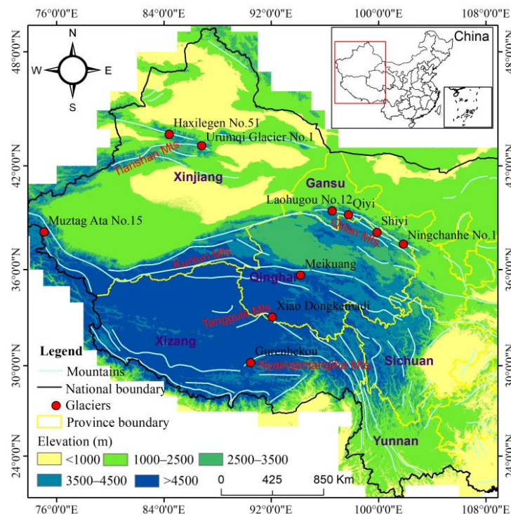
Figure 1 Spatial distribution of the ten continental-type glaciers in China.
