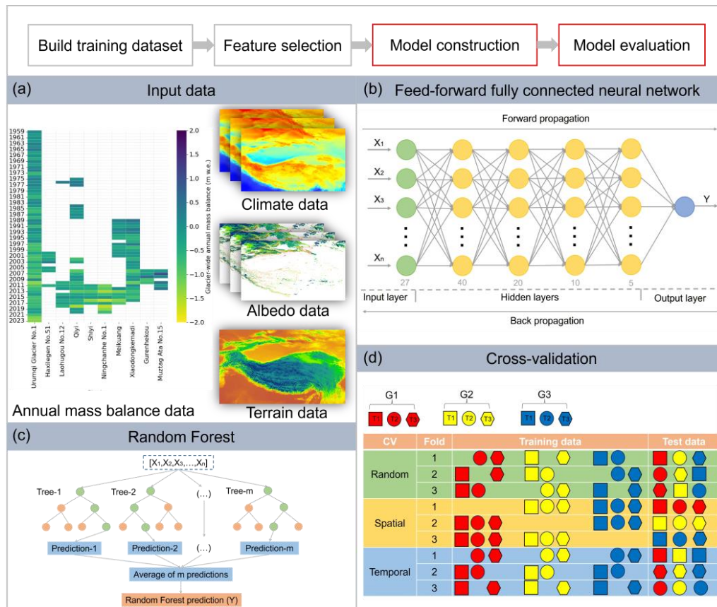
Figure 4 Schematic workflow of this study. (a) Input dataset used for RF and FF-FCNN models. (b) Architecture of the deep neural network. (c) RF model structure. (d) Schematic depiction of the model evaluation framework. The figure was recreated and modified from Meyer et al. (2018).
