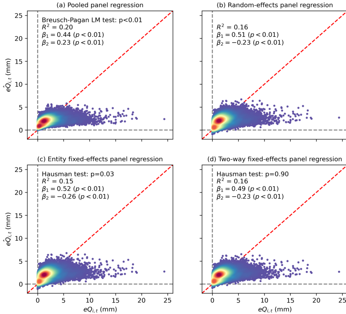
230 Figure 3. Streamflow reanalysis errors and the estimated errors for (a) pooled, (b) random-effects, (c) entity fixed-effects and (d) two-way 235 fixed-effects panel regression.
