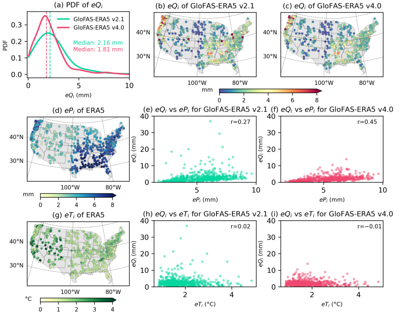
190 Figure 1. Statistical and spatial distributions of reanalysis errors. (a-c) Probability distribution function (PDF) and spatial distribution of streamflow reanalysis errors for GloFAS-ERA5 v2.1 and v4.0. (d-i) Spatial distribution of precipitation reanalysis errors and temperature reanalysis errors, as well as their relationships with streamflow reanalysis errors.
