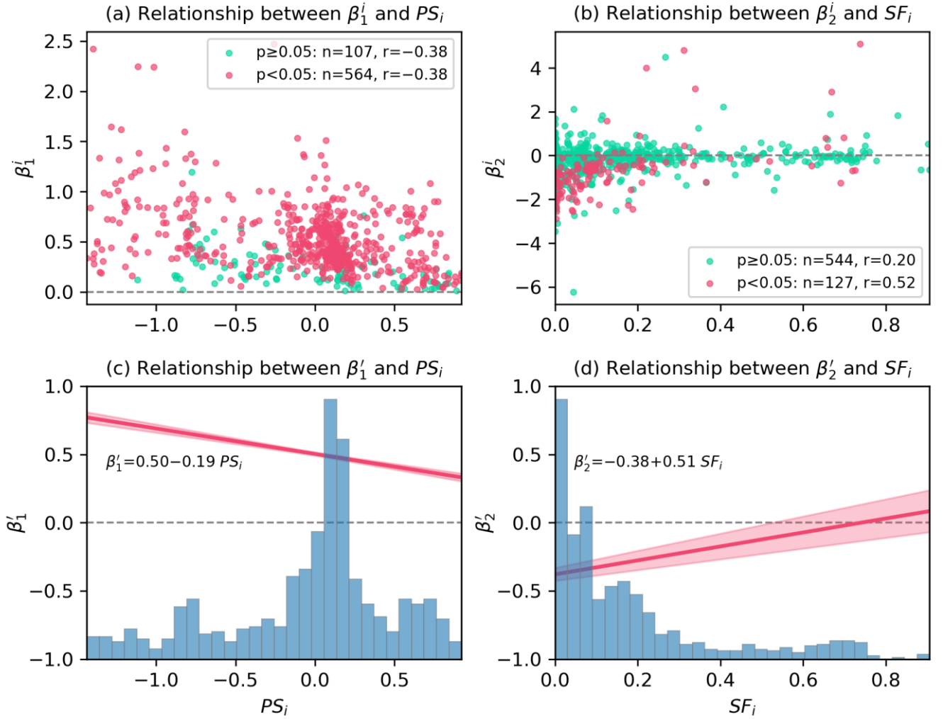
280 Figure 6. Relationships between effects of reanalysis errors and hydroclimatic attributes of catchments. Scatter plots illustrate the relationship between (a) effects of precipitation errors and precipitation seasonality and (b) effects of temperature errors and snow fraction. Panels (c) and (d) show the marginal effects of precipitation reanalysis errors as a function of precipitation seasonality and temperature reanalysis errors as a function of snow fraction, respectively. In (a) and (b), r and n respectively denote the Pearson's correlation coefficient and the number of catchments where the linear regression coefficients are statistically significant ( p < 0.05 ) or insignificant ( p \geq 0.05 ). In (c) and (d), the solid red lines represent the marginal effects derived from the random-effects panel regression with interaction terms in Eq. (10) with shaded 95% confidence intervals. The histograms show the distributions of respective catchment attributes. 285
