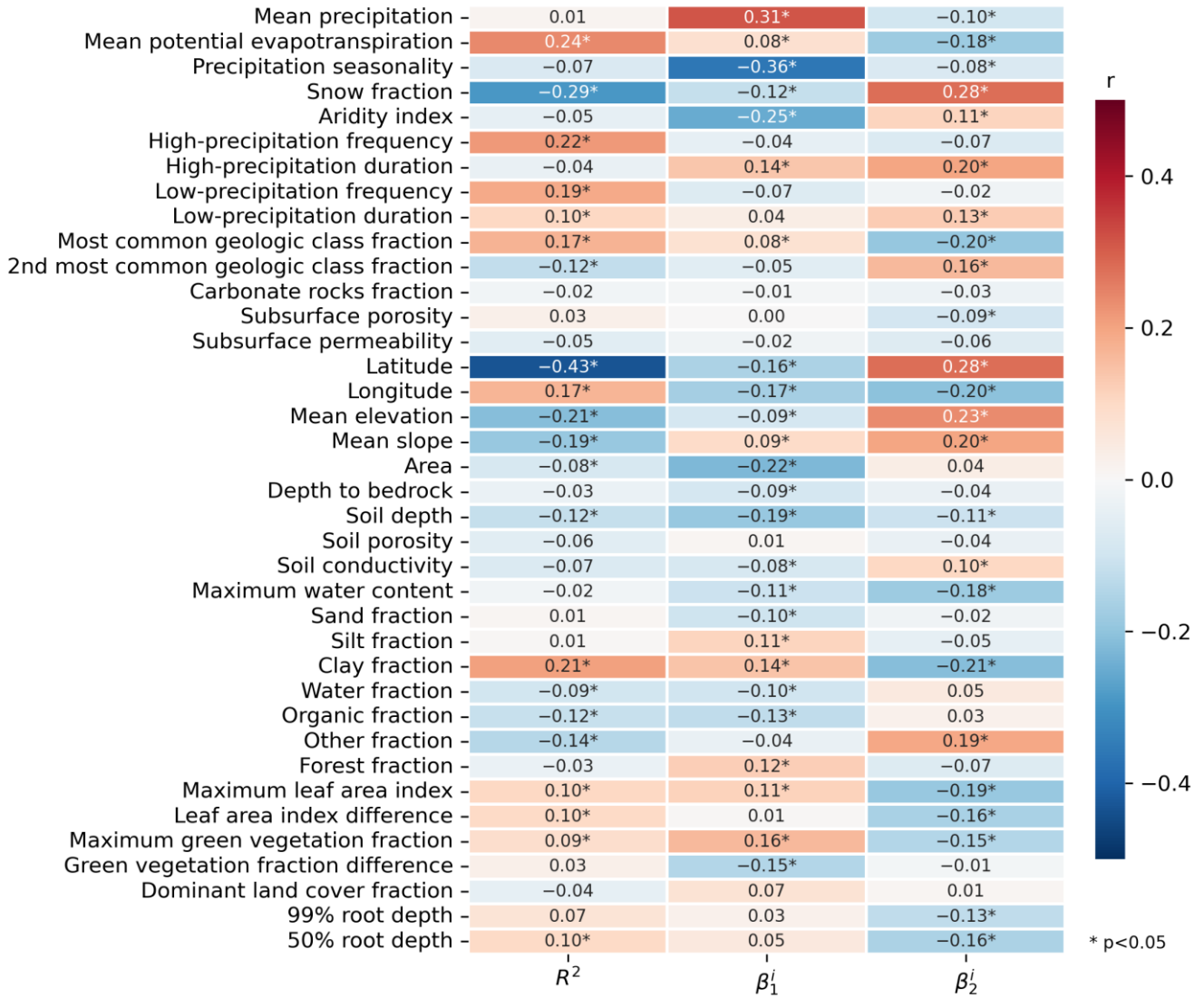
265 Figure 5. Pearson's correlation coefficients ( r ) between catchment attributes in the CAMELS dataset and the coefficient of determination ( R^2 ), 270 effects of precipitation reanalysis errors ( \beta_1^t ) and effects of temperature errors ( \beta_2^t ) for catchment-specific linear regression.
