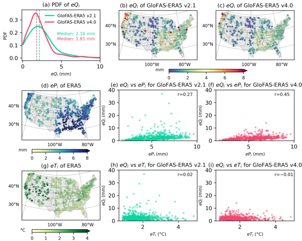
Figure 1. Statistical and spatial distributions of reanalysis errors. (a-c) Probability distribution function (PDF) and spatial distribution of streamflow reanalysis errors for GloFAS-ERA5 v2.1 and v4.0. (d-i) Spatial distribution of precipitation reanalysis errors and temperature reanalysis errors, as well as their relationships with streamflow reanalysis errors.
