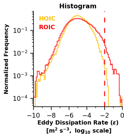
Figure C1. Normalized frequency histograms of ice crystals with different orientations at different turbulent dissipation rates, using the rigorous cloud identification scheme. The vertical red dashed line represents the turbulent dissipation rate threshold of 10^{-2} \text{ m}^2 \text{ s}^{-3} identified in this study, at which the occurrence frequency of HOICs decreases rapidly.
