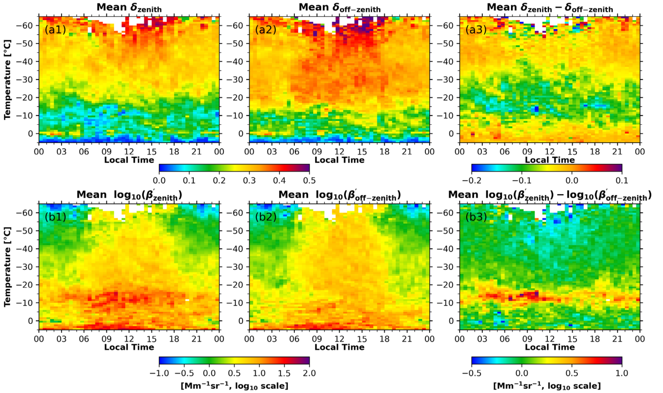
520 Figure 8. Local time versus temperature cross-sections of the mean values of: (a) volume depolarization ratio and (b) attenuated backscatter ( \log_{10} scale). Local time is given in China Standard Time (UTC+8). Panels correspond to (1) zenith-pointing lidar, (2) off-zenith pointing lidar, and (3) the difference between the zenith and off-zenith measurements.
