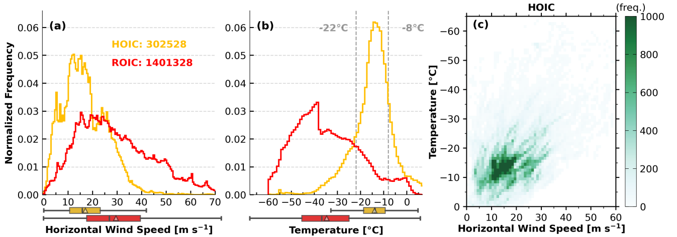
Figure 10. Environmental-variable distributions for the various cloud-phase classes during 2022. (a) The normalized histogram of horizontal wind speed for HOICs (orange) and ROICs (red), with boxplots shown below the x-axis. Boxes span the lower to upper quartiles; gray lines mark medians and triangles mark means. The whiskers reach either the data extremes or 1.5 times the interquartile range. (b) The normalized histogram of temperature for HOICs and ROICs, with boxplots shown below the x-axis. (c) Joint density of horizontal wind speed and ambient temperature for HOIC, with darker green marking more frequent HOIC observations.
