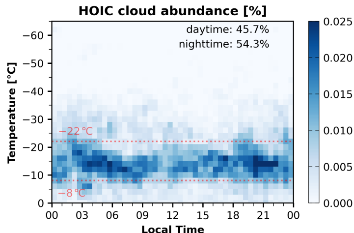
560 Figure 9. Local time-temperature cross-sections displaying the cloud abundance of HOICs based on a relaxed cloud mask. Local time is given in China Standard Time (UTC+8). The data are gridded with a 30-min temporal resolution and a 2-K temperature resolution. The daytime and nighttime proportions of HOIC are noted in the upper-right part. The upper and lower limits of the typical formation temperature regime for plate-like ice crystals ( -22^{\circ}\text{C} and -8^{\circ}\text{C} ) are also indicated with red dashed lines.
