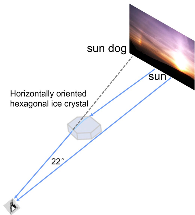
850 Figure A1. Schematic diagram illustrating the formation mechanism of sun dog. The solid blue line represents the parallel sunlights emitted by the sun, and the gray dashed line indicates the backward extension of the sunlight rays as seen by the observer. Sunlight undergoes two refractions within the prism facets of horizontally oriented hexagonal ice crystals, resulting in a 22° deviation in the light propagation path. The observer perceives a light spot at the intersection of the backward extensions of multiple light rays; this light spot is a virtual image, which is known as a sun dog (parhelion).
