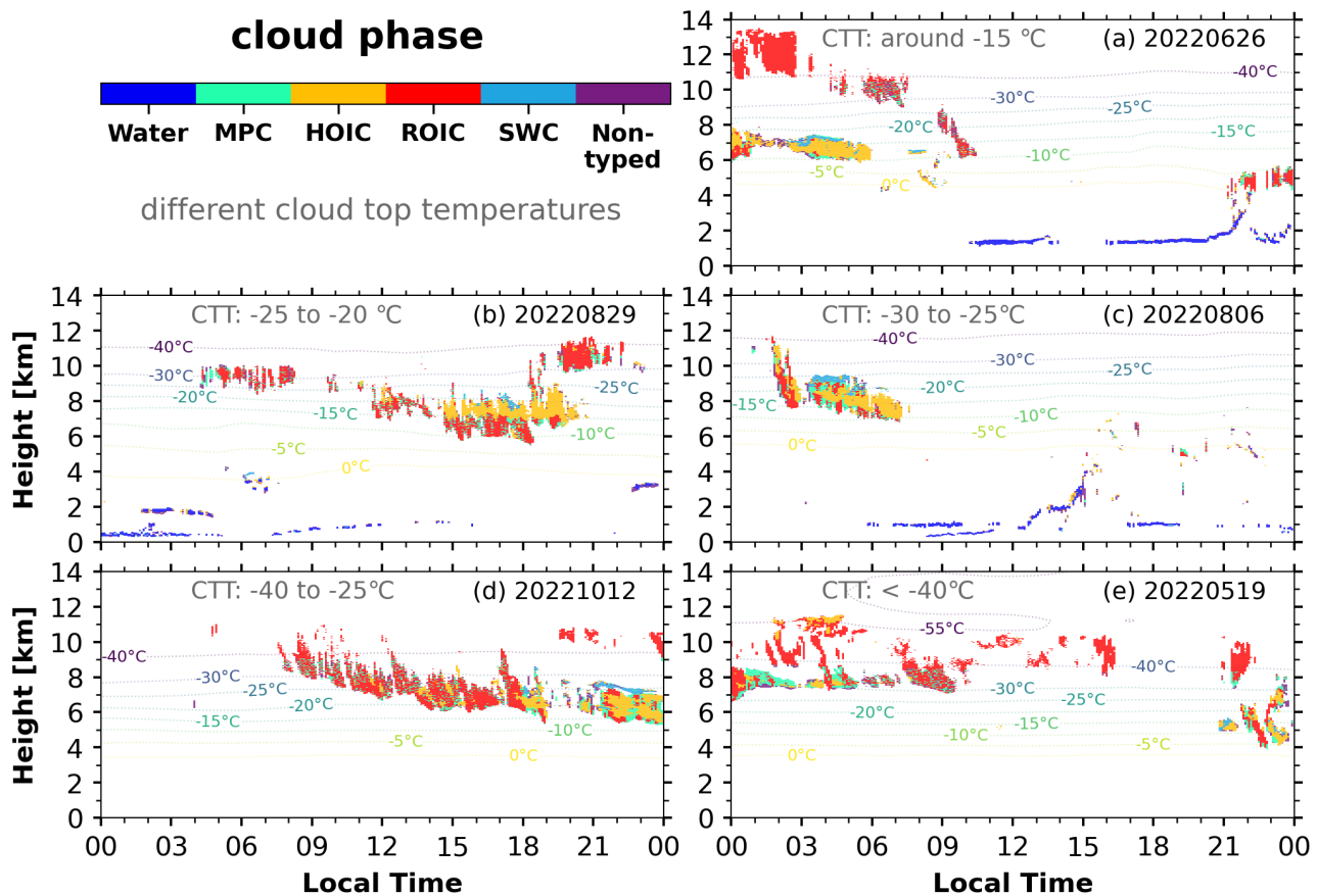
235 Figure 2. Cloud phase classification plots of horizontally oriented ice crystal (HOIC) cases under different cloud-top temperatures (CTT) across various days in 2022. (a) 26 June 2022 case, CTT around -15^{\circ}\text{C} ; (b) 29 August 2022 case, CTT from -25^{\circ}\text{C} to -20^{\circ}\text{C} ; (c) 6 August 2022 case, CTT from -30^{\circ}\text{C} to -25^{\circ}\text{C} ; (d) 12 October 2022 case, CTT from -40^{\circ}\text{C} to -25^{\circ}\text{C} ; (e) 19 May 2022 case, CTT around -55^{\circ}\text{C} (below -40^{\circ}\text{C} ). The relaxed cloud mask was used for these classifications.
