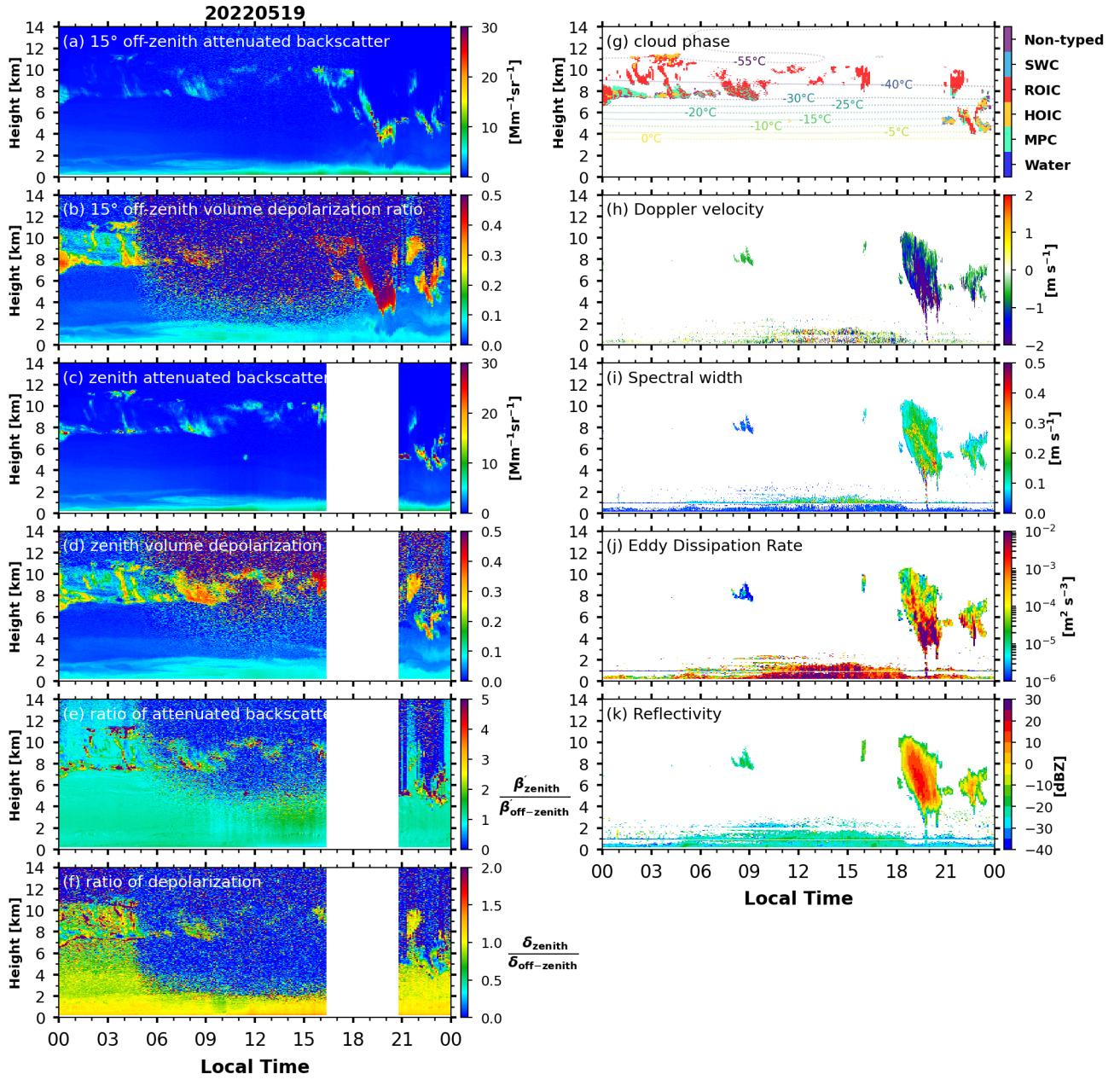
880 Figure B5. As in Fig. B1, but showing lidar and radar observations on 19 May 2022. The HOIC-containing layer has a cloud-top temperature around -55^\circ\text{C} .
