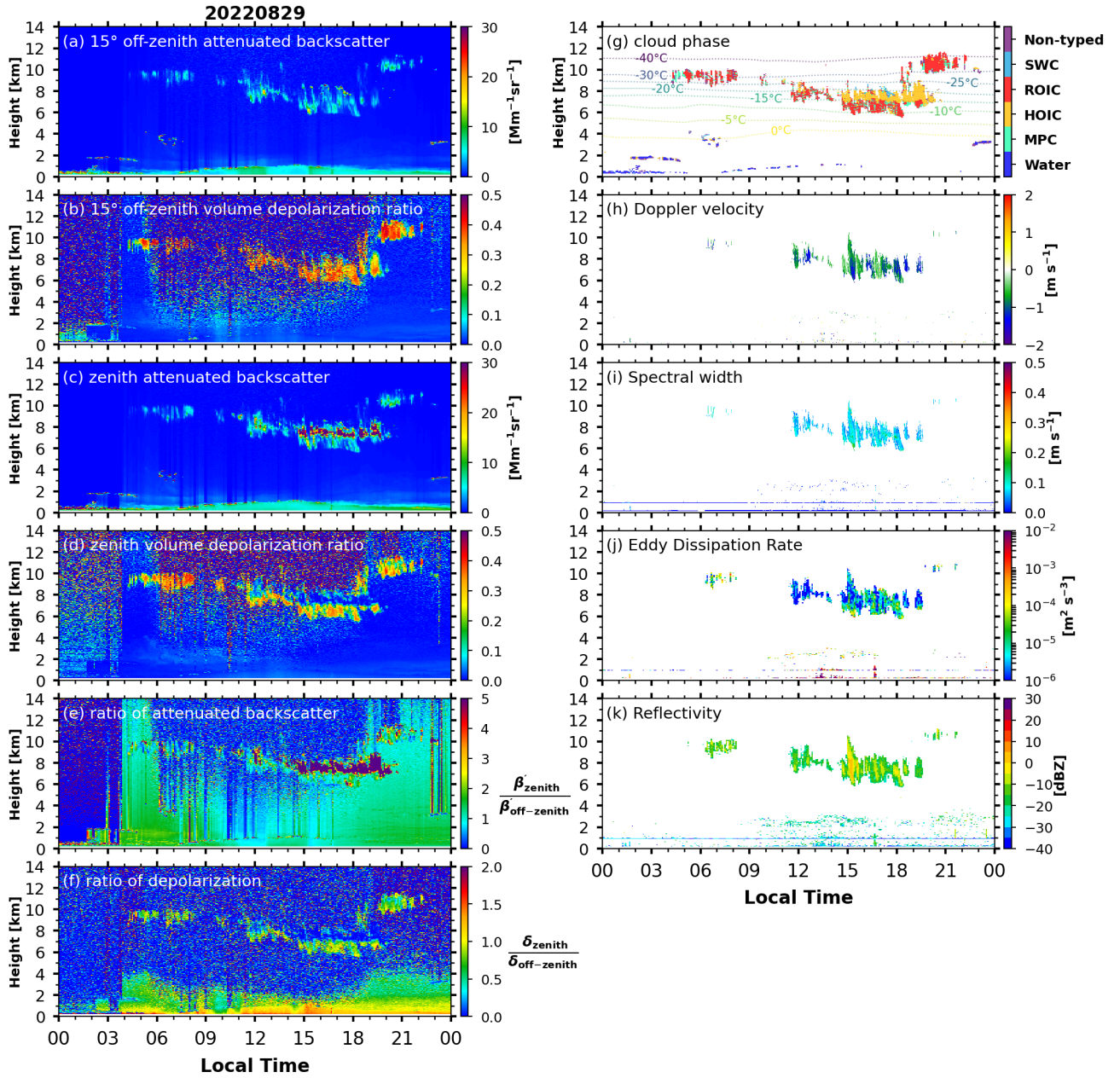
870 Figure B2. As in Fig. B1, but showing lidar and radar observations on 29 August 2022. The HOIC-containing layer has cloud-top temperature from -25 to -20 °C, corresponding to the plate-like crystal growth regime.
