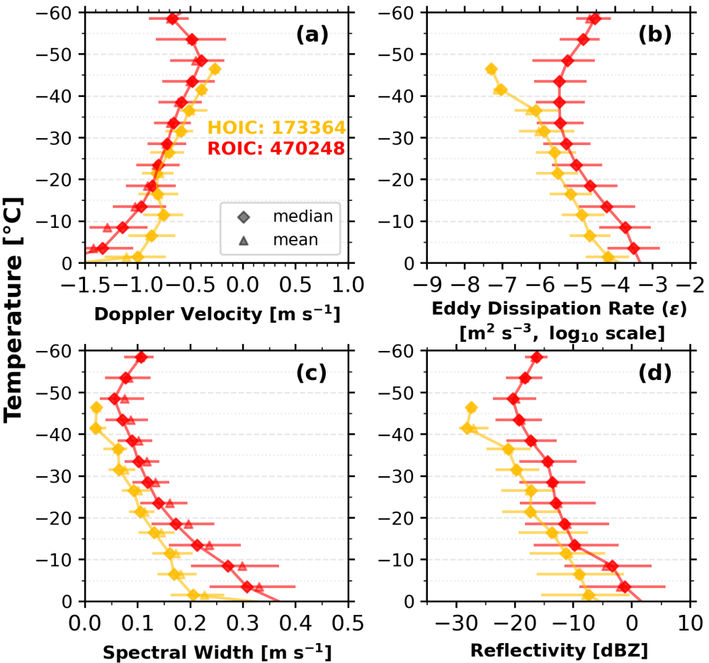
700 Figure 13. Distributions of cloud radar observations and retrievals across temperature intervals for different ice-crystal orientations: 705 (a) Doppler velocity; (b) eddy dissipation rate; (c) Doppler spectral width; and (d) radar reflectivity factor. Diamonds and triangles 710 denote the medians and means within each 5 °C temperature bin, respectively. The horizontal lines span the 25th–75th percentile range.
