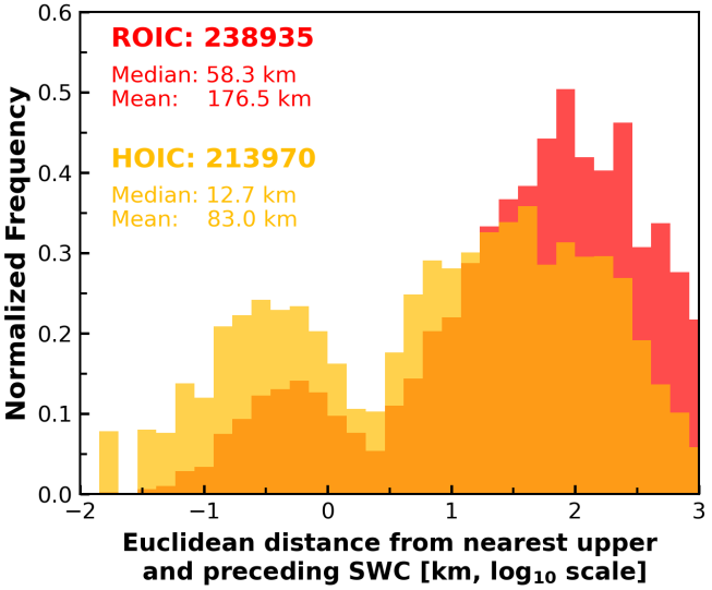
625 Figure 11. The normalized frequency of the Euclidean distances between HOICs, ROICs, and overlying SWCs. This normalized histogram utilizes data from the entire year of 2022, with the x-axis on a \log_{10} scale in kilometers (km). The orange and red shading give the HOIC and ROIC distributions, with their median and mean distances annotated in the top-left part. Note: To make the analysis physically consistent with ice-crystal sedimentation, the selected SWCs must temporally precede and be located spatially above the observed ice crystals.
