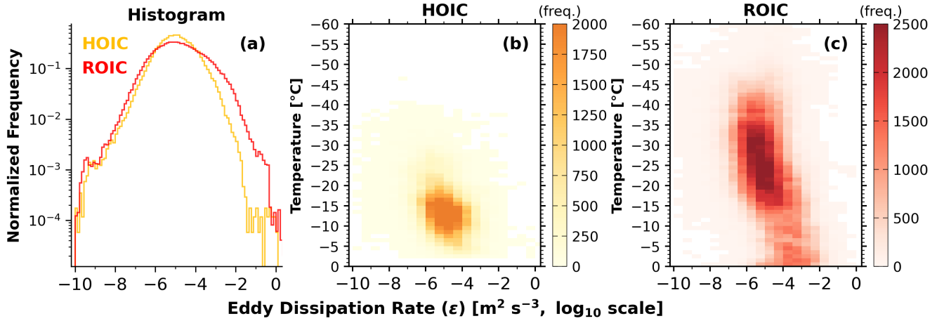
675 Figure 12. Statistical distributions of turbulent eddy dissipation rates (EDR, \epsilon ) for different orientations of ice crystals, based on the relaxed cloud mask. (a) Normalized histograms of ambient EDR for HOICs (orange) and ROICs (red), plotted on a \log_{10} scale. (b) Scatter density plot of EDR versus temperature for HOIC. (c) Scatter density plot of EDR versus temperature for ROIC.
