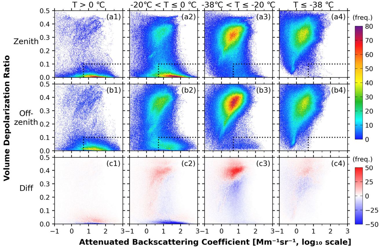
Figure 4. Volume depolarization ratio versus attenuated backscatter ( \log_{10} scale) density scatter plots across different temperature intervals for: (a) zenith-pointing lidar; (b) off-zenith pointing lidar; and (c) the density difference between off-zenith and zenith measurements. Data points are shown in blue where the zenith scatter density exceeds the off-zenith density, and in red where the off-zenith density is higher. Panels correspond to the following temperature regimes: (1) T > 0 °C; (2) -20 °C < T \leq 0 °C; (3) -38 °C < T \leq -20 °C; and (4) T \leq -38 °C. The liquid-water-cloud identification threshold is marked by the black dashed line at lower right (see Wu et al., 2025, Fig. 3c). This figure includes all cloud data points measured in 2022. During the gridding process, the resolutions for the \log_{10} \beta' and \delta were set to 0.01 and 0.2%, respectively.
