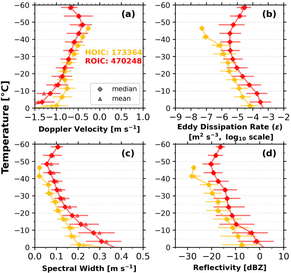
715 Figure 13. Distributions of cloud radar observations and retrievals across temperature intervals for different ice-crystal orientations: (a) Doppler velocity; (b) eddy dissipation rate; (c) Doppler spectral width; and (d) radar reflectivity factor. Diamonds and triangles denote the medians and means within each 5 °C temperature bin, respectively. The horizontal lines span the 25th–75th percentile range.
