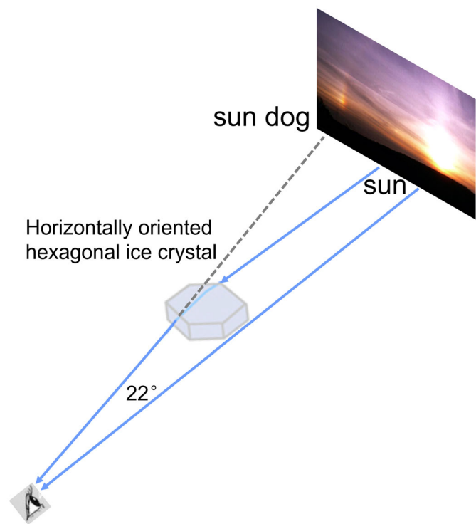
865 Figure A1. Schematic diagram illustrating the formation mechanism of sun dog. The solid blue line represents the parallel sunlights emitted by the sun, and the gray dashed line indicates the backward extension of the sunlight rays as seen by the observer. Sunlight undergoes two refractions within the prism facets of horizontally oriented hexagonal ice crystals, resulting in a 22° deviation in the light propagation path. The observer perceives a light spot at the intersection of the backward extensions of multiple light rays; this light spot is a virtual image, which is known as a sun dog (parhelion).
