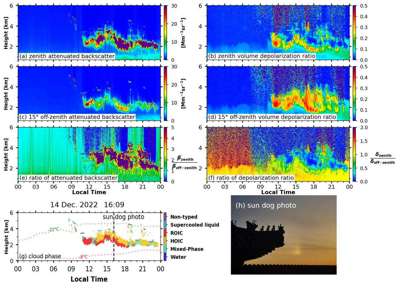
Figure 1. Lidar observations ((a)-(f)), cloud phase categorization (g), and sun dog photo (h) on 14 December 2022 (5 min / 15 m resolution for (a)-(g)). (a) Zenith-pointing lidar attenuated backscatter. (b) Zenith-pointing lidar volume depolarization ratio. (c) 15° off-zenith-pointing lidar attenuated backscatter. (d) 15° off-zenith-pointing volume depolarization ratio. (e) The ratio of attenuated backscatter for zenith-pointing and off-zenith-pointing lidar. (f) The ratio of volume depolarization ratio for zenith-pointing and off-zenith-pointing lidar. (g) Cloud phase categorization results with an isotherm from ERA5 data and a vertical dashed line indicating the sun dog observation time. (h) Sun dog (parhelion) photograph with traditional Chinese-style roof photographed at 16:09 (local time, UTC+8), 14 December 2022, approximately 3 km from the lidar station (the Summer Palace, Beijing). Photo courtesy of Hai Feng, used with permission.
