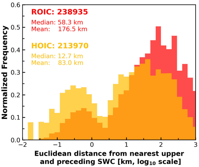
640 Figure 11. The normalized frequency of the Euclidean distances between HOICs, ROICs, and overlying SWCs. This normalized histogram utilizes data from the entire year of 2022, with the x-axis on a log 10 scale in kilometers (km). The orange and red shading give the HOIC and ROIC distributions, with their median and mean distances annotated in the top-left part. Note: To ensure a causal relationship To make the analysis physically consistent with ice-crystal sedimentation , the selected SWCs must temporally precede and be located spatially above the observed ice crystals.
