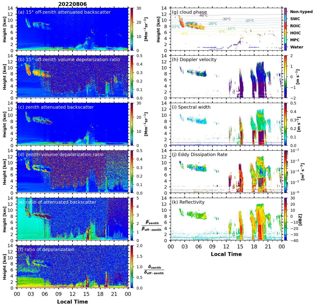
Figure B3. As in Fig. B1, but showing lidar and radar observations on 6 August 2022. The HOIC-containing layer has cloud-top temperature of approximately -30 to -25 °C, corresponding to the plate-based polycrystal growth regime.
