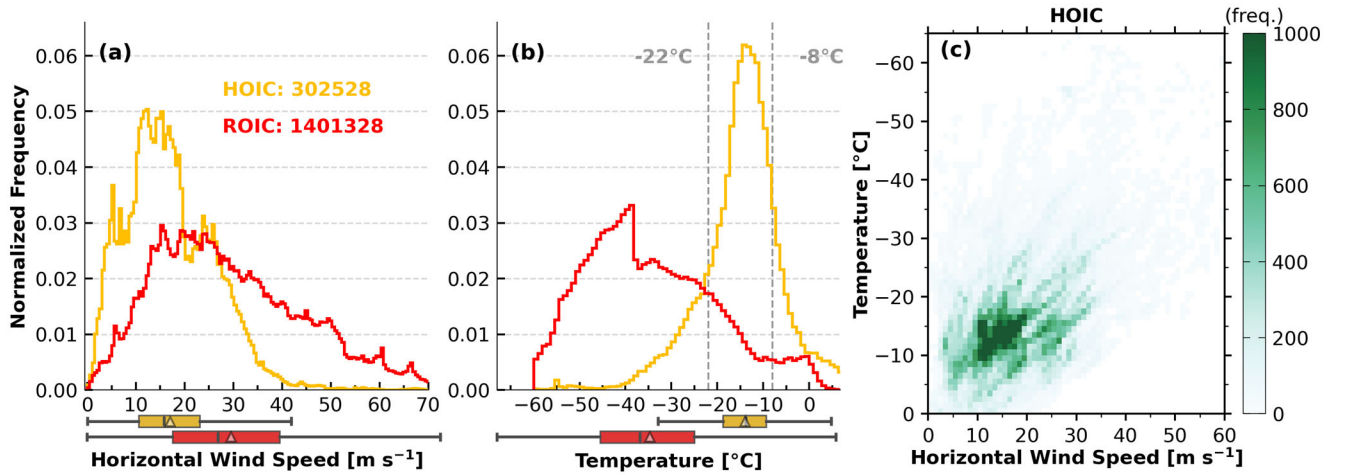
605 Figure 10. Environmental-variable distributions for the various cloud-phase classes during 2022. (a) The normalized histogram of horizontal wind speed for HOICs (orange) and ROICs (red), with boxplots shown below the x-axis. Boxes span the lower to upper quartiles; gray lines mark medians and triangles mark means. The whiskers reach either the data extremes or 1.5 times the interquartile range. (b) The normalized histogram of temperature for HOICs and ROICs, with boxplots shown below the x-axis. (c) Joint density of horizontal wind speed and ambient temperature for HOIC, with darker green marking more frequent HOIC 610 observations.
