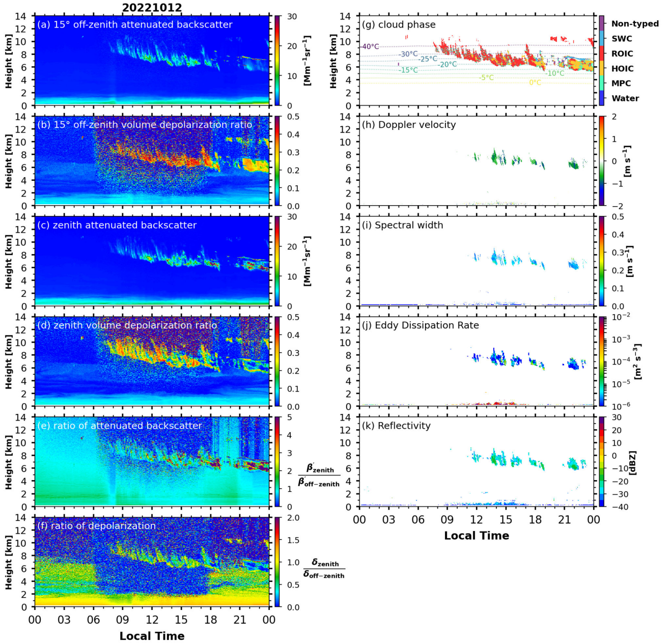
Figure B4. As in Fig. B1, but showing lidar and radar observations on 12 October 2022. The HOIC-containing layer has cloud-top temperature from -40 to -25 °C.
