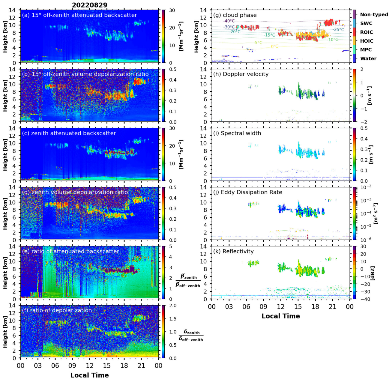
885 Figure B2. As in Fig. B1, but showing lidar and radar observations on 29 August 2022. The HOIC-containing layer has cloud-top temperature from -25 to -20 °C, corresponding to the plate-like crystal growth regime.
