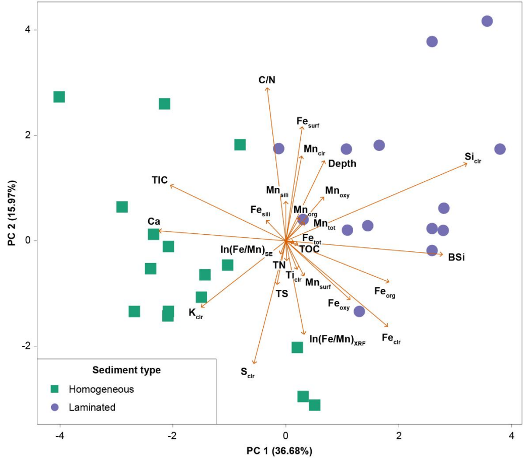
Figure A3: Robust principal component analysis biplot based on multivariable dataset from 30 surface samples. One sample was removed due to an error in the sequential extraction measurement.
