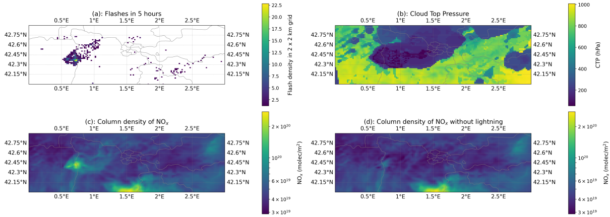
Figure 3. WRF-Chem simulation results for 6 July 2024 at 13:50 UTC, focused on the region of interest. (a): Assimilated lightning flashes between 08:50 and 13:50 UTC reported by Meteosat 12 LI. (b): Cloud Top Pressure (CTP). (c): Vertical Column Density of \text{NO}_x . (d): Vertical column density of \text{NO}_x in the simulation without fresh \text{LNO}_x , i.e., with \text{LNO}_x deactivated after 07:00 UTC. Meteosat 12 LI lightning data © EUMETSAT.
