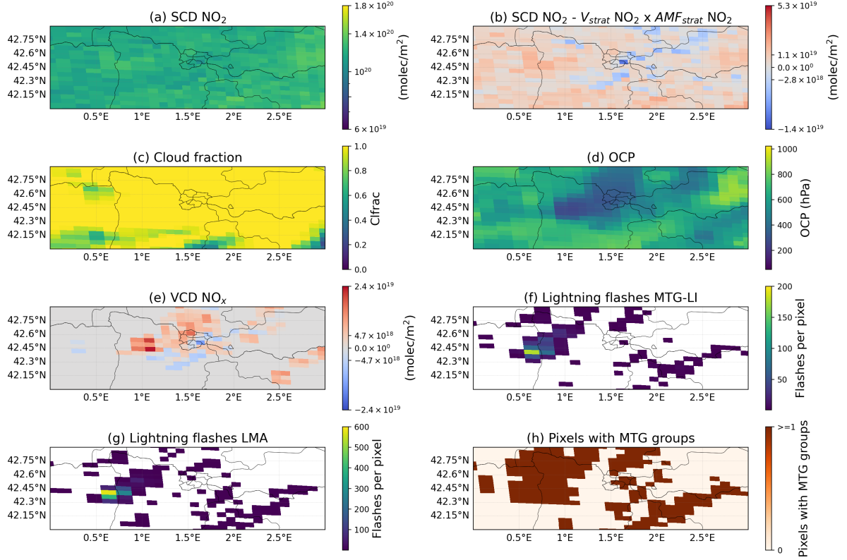
Figure 5. TROP-DLR product of orbit 34875, Meteosat 12 LI and LMA lightning data for the case 6 July 2024. (a): Slant Column Density (SCD) \text{NO}_2 provided by the TROP-DLR \text{NO}_2 research product. (b): SCD \text{NO}_2 minus the stratospheric vertical column density multiplied by the stratospheric air mass factor of \text{NO}_2 ( \text{AMF}_{\text{strat}} ) obtained from the TROP-DLR \text{NO}_2 research product. (c) and (d): Cloud Fraction (CF) and Optical Centroid Pressure (OCP) from the TROP-DLR \text{NO}_2 research product, respectively. (e): \text{VCD NO}_x ( V_{\text{tropNO}_x} from equation (3)) over pixels satisfying the Deep Convective Constraint (DCC). (f) and (g): Lightning flashes during the 5 h period per TROPOMI pixel before the TROPOMI overpass reported by Meteosat 12 LI and the LMA, respectively. (h): TROPOMI pixels containing at least one lightning group detected by Meteosat 12 LI. Sentinel-5P TROPOMI data © ESA, processed by DLR. Meteosat 12 LI lightning data © EUMETSAT.
