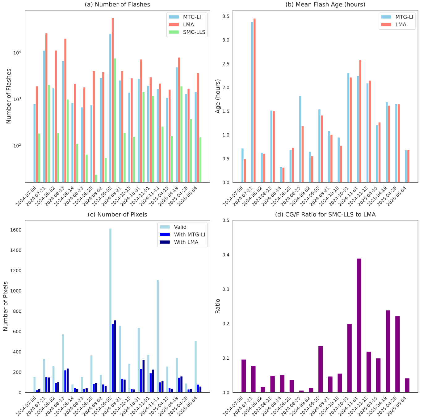
Figure 6. Total number flashes detected by Meteosat 12 LI, LMA and CG flashes detected by LLS-SMC up to 5 h before the overpass of TROPOMI (a), mean age of the flashes detected by Meteosat 12 LI and the LMA (b), total number of valid TROPOMI pixels satisfying the Deep Convective Constraint (DCC), total number of TROPOMI pixels with Meteosat 12 LI or LMA flashes satisfying the DCC (c), and ratio of the total number of CG flashes to all flashes detected by the LMA.
