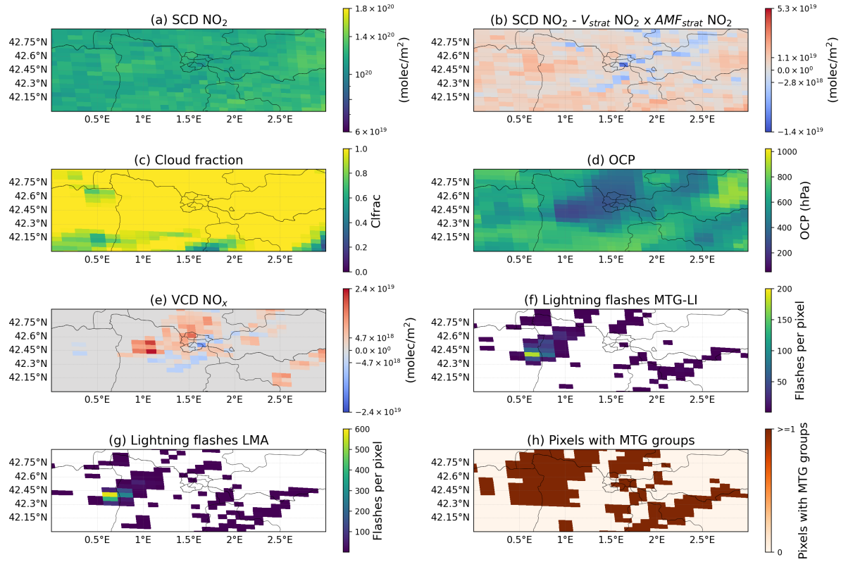
Figure 5. TROP-DLR product of orbit 34875, MTG-LI/Meteosat 12 LI and LMA lightning data for the case 6 July 2024. (a): Slant Column Density (SCD) \text{NO}_2 provided by the TROP-DLR \text{NO}_2 research product. (b): SCD \text{NO}_2 minus the stratospheric vertical column density and divided to multiplied by the stratospheric air mass factor of \text{NO}_2 ( AMF_{\text{strat}} ) obtained from the TROP-DLR \text{NO}_2 research product. (c) and (d): Cloud Fraction (CF) and Optical Centroid Pressure (OCP) from the TROP-DLR \text{NO}_2 research product, respectively. (e): VCD \text{NO}_x ( V_{\text{tropNO}_x} from equation (3) over pixels satisfying the Deep Convective Constraint (DCC). (f) and (g): Lightning flashes during the 5 h period per TROPOMI pixel before the TROPOMI overpass reported by MTG-LI/Meteosat 12 LI and the LMA, respectively. (h): TROPOMI pixels containing at least one lightning group detected by MTG-LI/Meteosat 12 LI . Sentinel-5P TROPOMI data © ESA, processed by DLR. Meteosat 12 LI lightning data © EUMETSAT.
