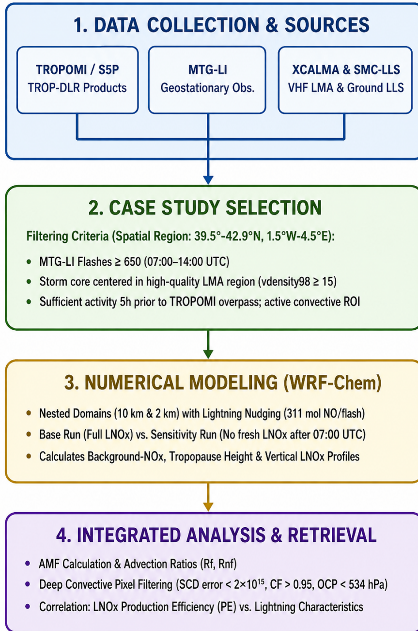
Figure 1. Overview of the methodological framework used to investigate lightning-produced \text{NO}_x using satellite observations, ground-based lightning measurements, and numerical modeling.
