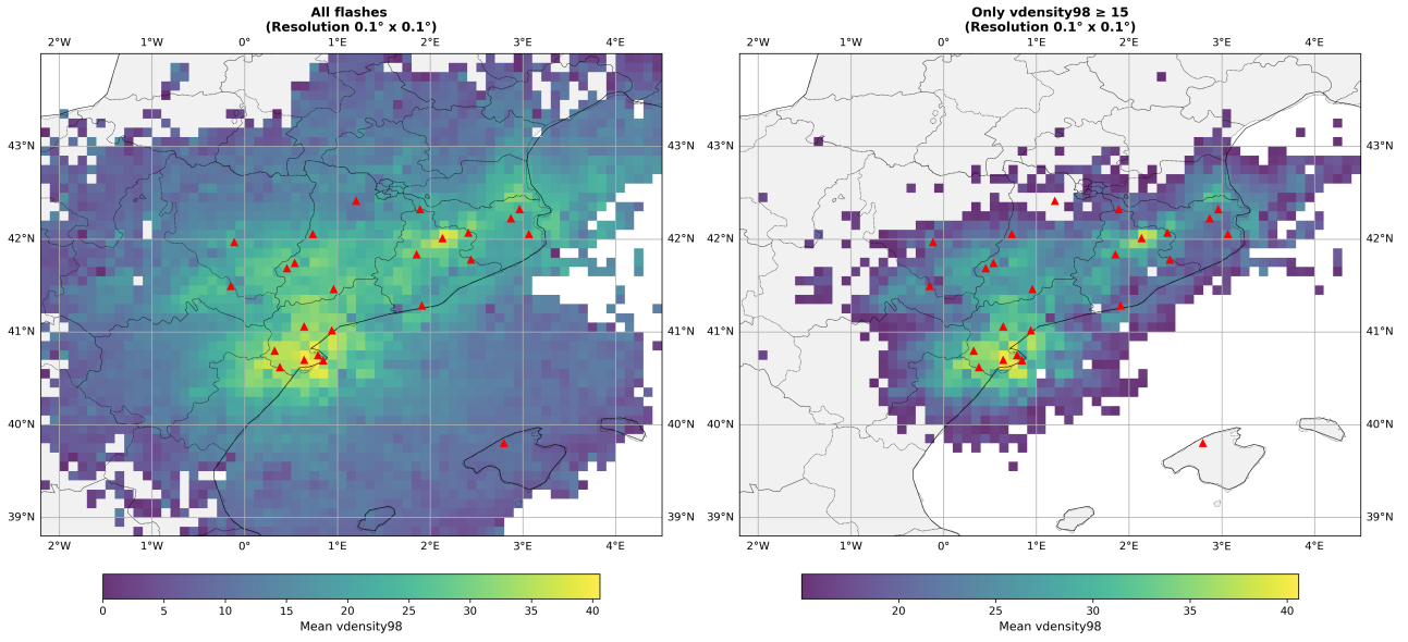
Figure 2. Left panel: 98 th percentile vertical density score ( vdensity98 ) averaged over all the flashes analyzed in this study and contained in each 0.1^\circ \times 0.1^\circ . Right panel: Masked data showing only pixels with vdensity98 \geq 15 , showing the region with the best quality XCALMA data. Locations of the XCALMA sensors are included (red triangles).
