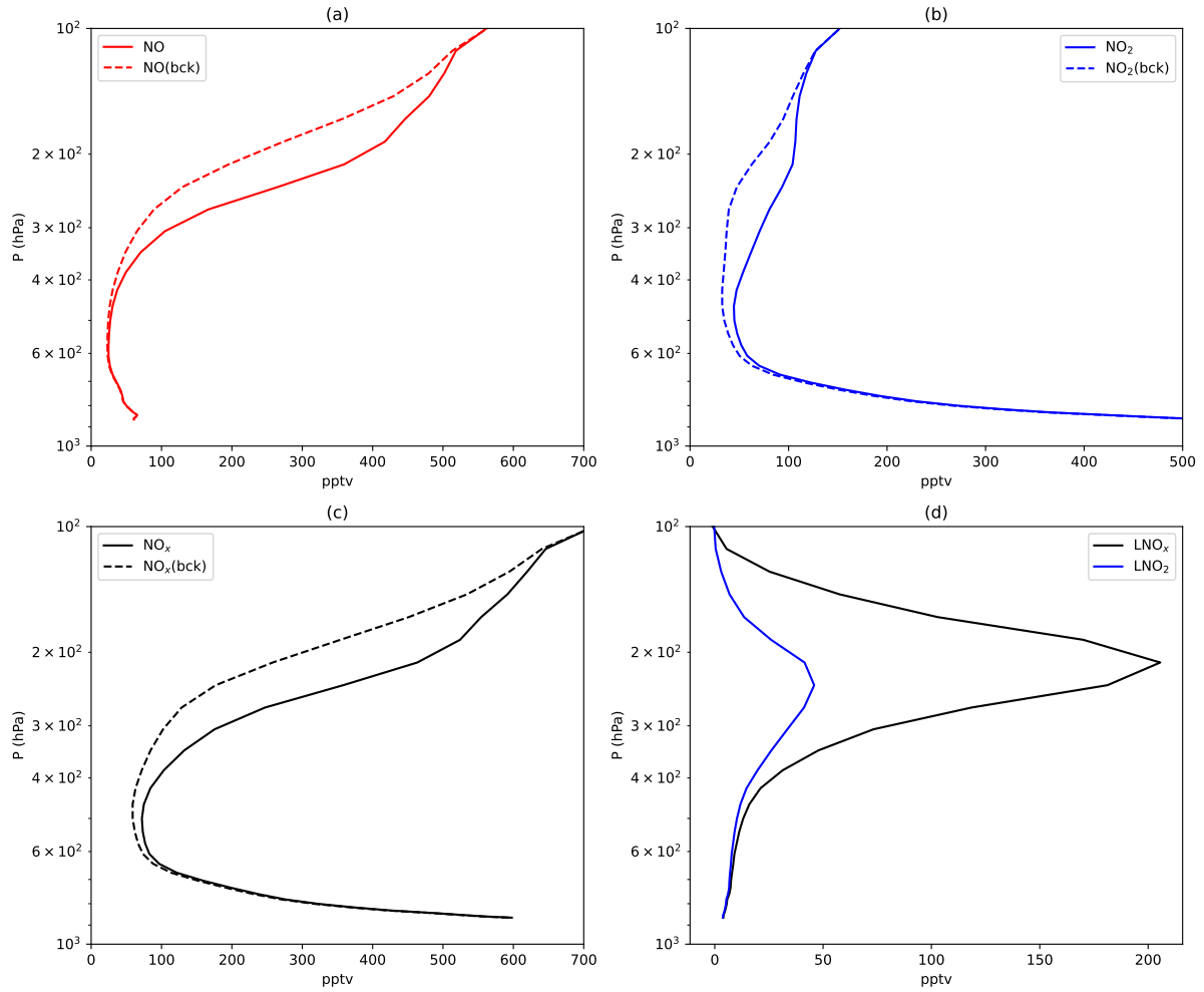
Figure 4. Vertical mixing ratio profiles of NO (a), NO 2 (b), NO x (c), LNO x and LNO 2 (d) extracted from WRF-Chem simulations with (solid lines) and without (dashed lines) fresh LNO x on 6 July 2024 at 13:50 UTC (close to the TROPOMI overpass (background: bck)).
