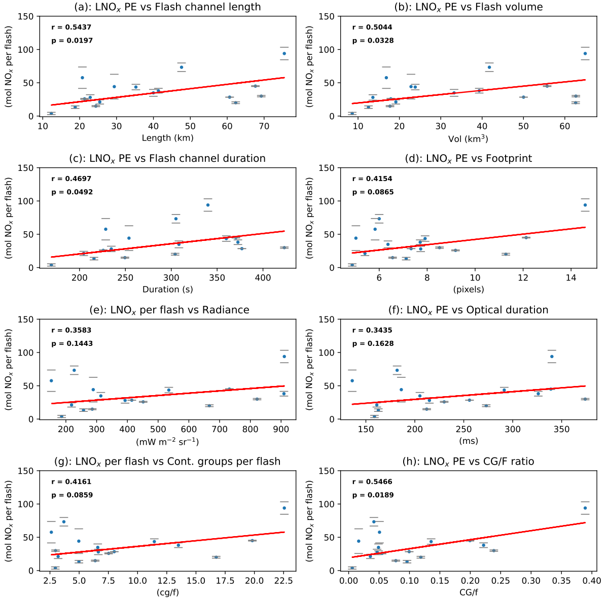
Figure 8. Pearson correlation between the LNO x PE and the most important lightning characteristics included in this study. The average LNO x PE (blue points) is obtained as the average between the LNO x PE estimates by using both MTG-LI-Meteosat 12 LI and the LMA for each analyzed case, while each pair of grey bars are the values of the LNO x PE estimates by using MTG-LI-Meteosat 12 LI and the LMA separately. The flash channel length, the flash volume and the flash durations in panels (a), (b) and (c) are the average values calculated from LMA measurements. The footprint, the radiance, the flash durations and the total number of contiguous groups per flash in panels (d), (e), (f) and (g) are the average values calculated from MTG-LI-Meteosat 12 LI measurements. The average ratio of CG to total flashes in panel (h) is obtained from LLS-SMC and LMA lightning measurements. Each subplot includes the Pearson correlation coefficient r and its corresponding p - value, as well as a linear fitting of the blue points (red line). These results are based on calculations with \tau = 5 h.
