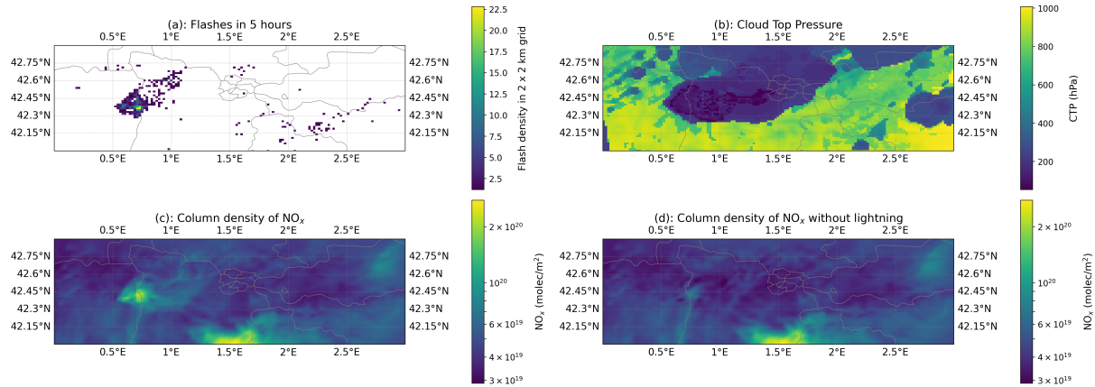
Figure 3. WRF-Chem simulation results for 6 July 2024 at 13:50 UTC, focused on the region of interest. (a): Assimilated lightning flashes between 08:50 and 13:50 UTC reported by MTG-LI Meteosat 12 LI . (b): Cloud Top Pressure (CTP). (c): Vertical Column Density of \text{NO}_x . (d): Vertical column density of \text{NO}_x in the simulation without fresh \text{LNO}_x , i.e., with \text{LNO}_x deactivated after 07:00 UTC. Meteosat 12 LI lightning data © EUMETSAT .
