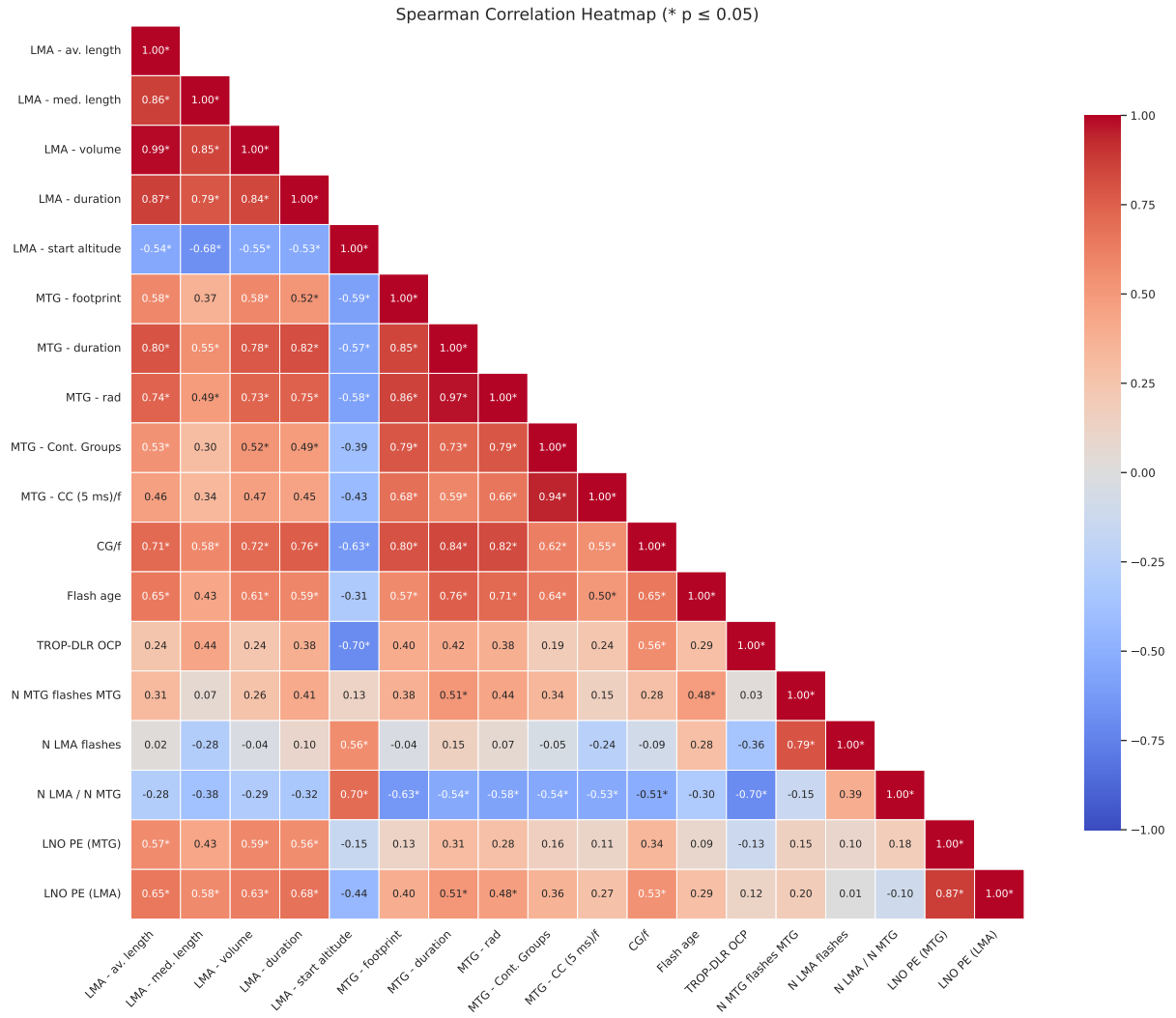
Figure 7. Spearman correlation heatmap of the most important lightning characteristics and LNO x PE estimates. These results are based on calculations with \tau = 5 h.
