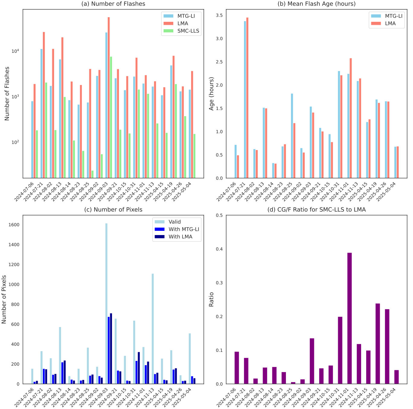
Figure 6. Total number flashes detected by MTG-LI Meteosat 12 LI , LMA and CG flashes detected by LLS-SMC up to 5 h before the overpass of TROPOMI (a), mean age of the flashes detected by MTG-LI Meteosat 12 LI and the LMA (b), total number of valid TROPOMI pixels satisfying the Deep Convective Constraint (DCC), total number of TROPOMI pixels with MTG-LI Meteosat 12 LI or LMA flashes satisfying the DCC (c), and ratio of the total number of CG flashes to all flashes detected by the LMA.
