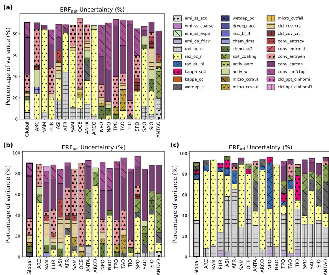
Figure R1. Same as Fig. 7 but with parameters related to anthropogenic, biomass burning, and DMS emissions fixed at their prior medians. Parameters contributing less than 3 % of the total uncertainty are not shown.
