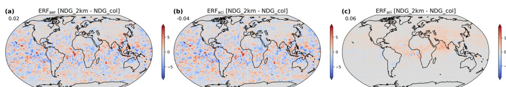
Figure R2. Differences in annual-mean (a) ERF aer , (b) ERF aci , and (c) ERF ari between the above-2km nudging (NDG_2km) and full-column nudging (NDG_col) experiments, based on single-model runs.
