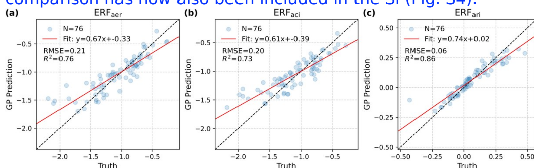
Figure R3. Comparison of globally averaged GP emulator predictions with test data (truth) for (a) ERF aer , (b) ERF aci , and (c) ERF ari .
