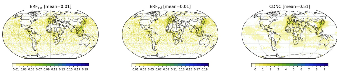
Figure R4. Parametric uncertainties ( 2\sigma across 200,000 emulated model variants) of ERFaer ( \text{W m}^{-2} ), ERFaci ( \text{W m}^{-2} ), and CDNC ( \text{cm}^{-3} ) over 1850–2025, caused by shipping \text{SO}_2 emissions ( emi_shp_so2 ). The fields are the same as those shown in Figs. S7, S8, and S15, but are displayed here using narrower colorbar ranges.
