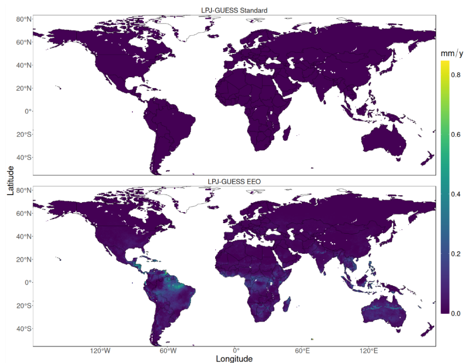
Fig. R1: Annual soil moisture deficit (transpirational demand – available soil water) on model timesteps at which soil moisture is depleted (average 1990-2010).
