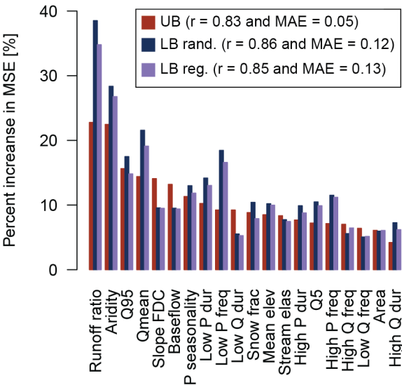
300 Figure 7: Importance of catchment attributes for predicting model performance NPE for the upper benchmark (UB), the lower benchmark represented by the ensemble mean of 1000 parameterizations (LB rand.), and the lower benchmark based on regionally donated parameter sets (LB reg.) of all CAMELS datasets using a random forest model. The importance of each variable is expressed in terms of the percentage increase in mean squared error (MSE) if that variable is randomly permuted for the prediction of NPE. If a catchment attribute is more important, the related percentage increase in MSE is higher. The performance of the random forest model for the test data was quantified by the Pearson correlation coefficient (r) and the mean absolute error (MAE).
