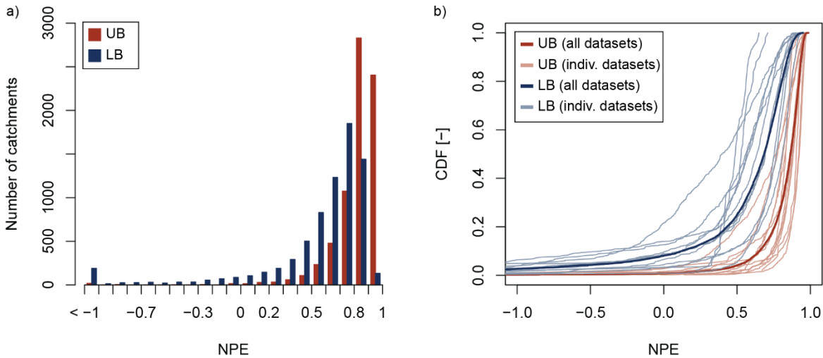
Figure 5: Model performances (NPE) for the upper benchmark (UB) and lower benchmark (LB; represented by the ensemble mean of 1000 parameterizations). a) Histogram showing the values for all CAMELS datasets. b) Cumulative distribution functions (CDFs) for all CAMELS datasets and the individual CAMELS datasets.
