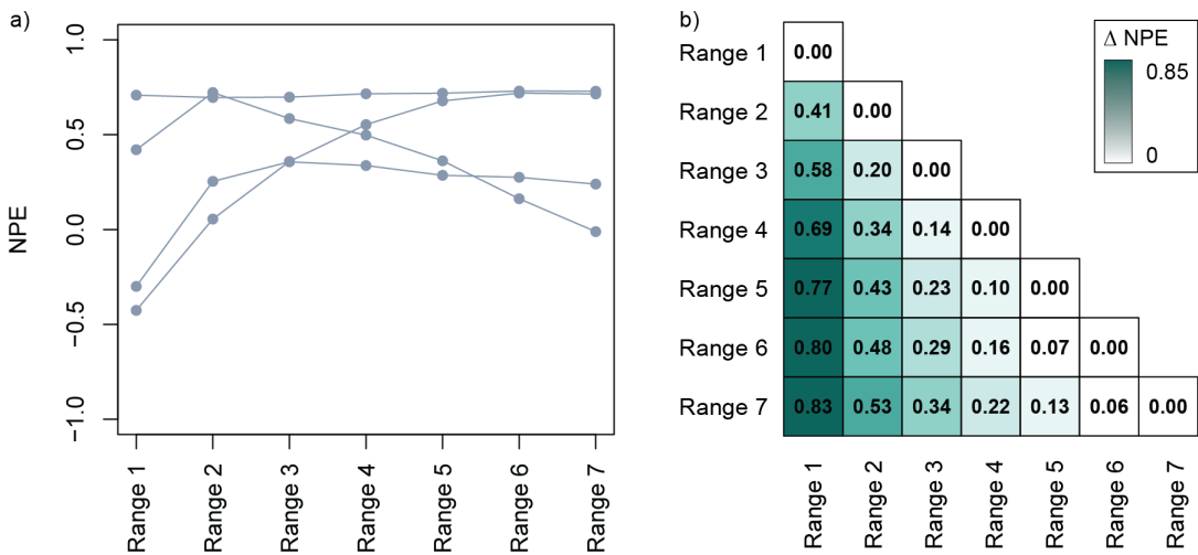
Figure 3: Effect of parameter ranges on the performance (NPE) of the lower benchmark. a) NPE-values for four example catchments, and b) pairwise mean absolute differences of the NPE values (based on all 128 test catchments from Australia, Brazil, Chile, and the US). Note that Range 1 corresponds to the parameter ranges between LL_1 and UL_1 Range 2 corresponds to the parameter ranges between LL_2 and UL_2, etcetera (see Table 3 for definitions and values). In other words, ranges varied from narrow (Range 1) to wide (Range 7).
