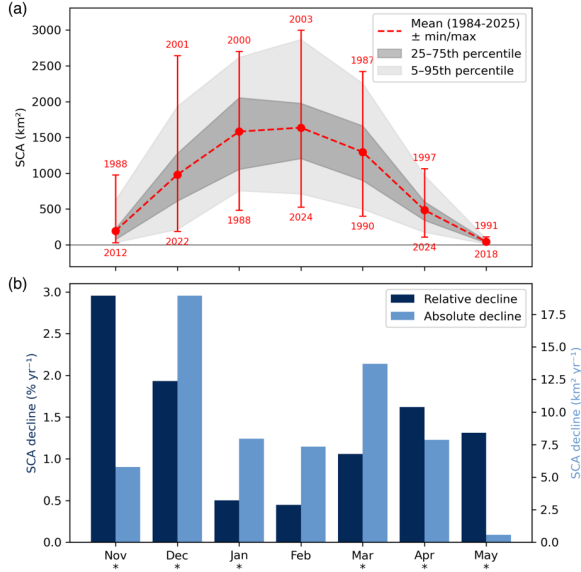
Figure 6: (a) Monthly mean, minimum, maximum, and 25-75th and 5-95th percentiles of snow cover area (SCA) across the snow season. (b) Decline in SCA, shown in absolute and relative terms, calculated based on the mean SCA for the period 1984-2025. Asterisks (*) denote statistically significant trends. All metrics are calculated for the entire study area.
