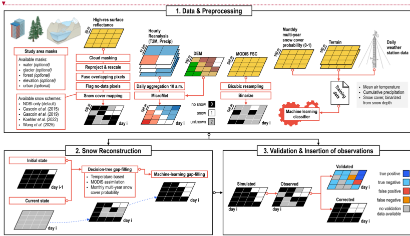
Figure 2: Schematic of the snowMapper v1.0 model.
