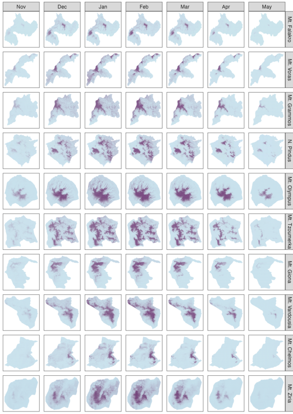
Figure A2: Monthly multiyear snow cover probabilities, calculated for the massifs of the study area (north to south) from all available Landsat & Sentinel-2 clear-sky observations between November 1984 and May 2025.
