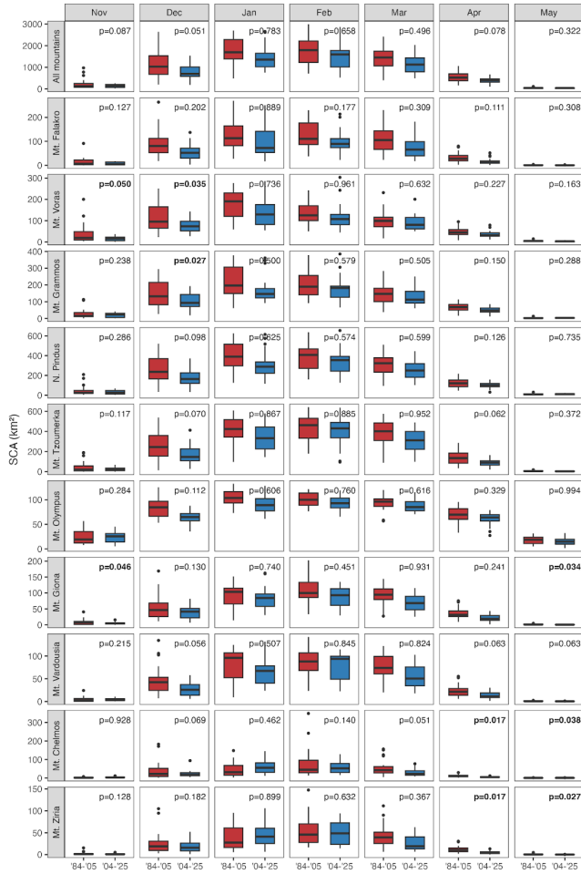
710 Figure A6: Monthly SCA variability per massif for the periods 1984-2005 and 2004-2025. P-values indicate the statistical significance of differences in variability between the two periods. Bold text denotes statistically significant differences.
