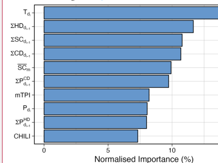
Figure 3: Normalised importance of each predictor variable in the snowMapper random forest classifier.
