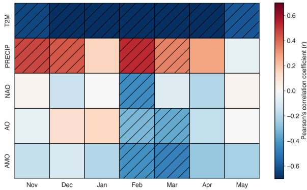
560 Figure 9: Pearson correlation coefficients between SCA and monthly mean 2 m air temperature (T2M), monthly cumulative precipitation (PRECIP), and major regional climate indices (NAO, AO, AMO) across all massifs in the study area. Red and blue indicate positive and negative correlations, respectively, and hatching denotes statistically significant values.
