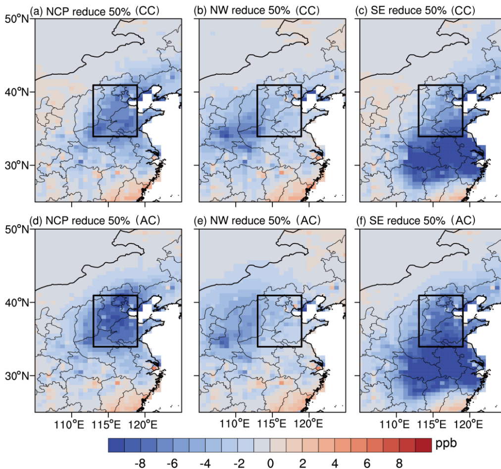
Figure 8. Response of MDA8 ozone concentration to 50% reductions in both \text{NO}_x and VOCs emissions in the (a, d) NCP, (b, e) NW, and (c, f) SE regions under cyclonic-like circulation (upper panel) and anticyclonic circulation (lower panel). The black rectangles denote the NCP. The NW and SE regions are indicated in Fig. S1.
