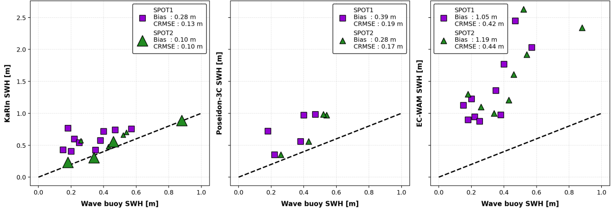
Figure 1: Scatter plots of the SWH measured by KaRIn (left panel), Poseidon-3C (middle panel) and the ECMWF model (right panel) versus the wave buoy estimated SWH. In the left panel, marker size qualitatively represents the cross-track distance of each wave buoy: approximately 12 km (SPOT1, SWOT track 388), 15 km (both buoys, SWOT track 485), and 40 km (SPOT2, SWOT track 388).
