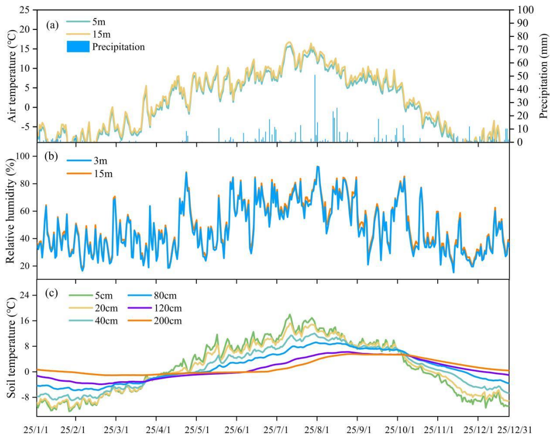
Fig. S1. Variations in air temperature and soil temperature in the QLB.
