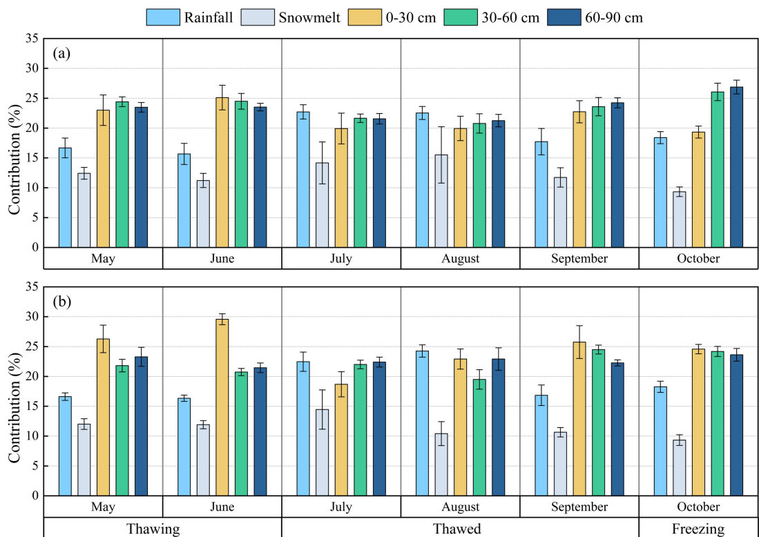
Fig. 7. Contribution of rainfall, snowmelt, and soil water from different depths to groundwater during the FT periods. (a) Middle and upper reaches. (b) Downstream.
