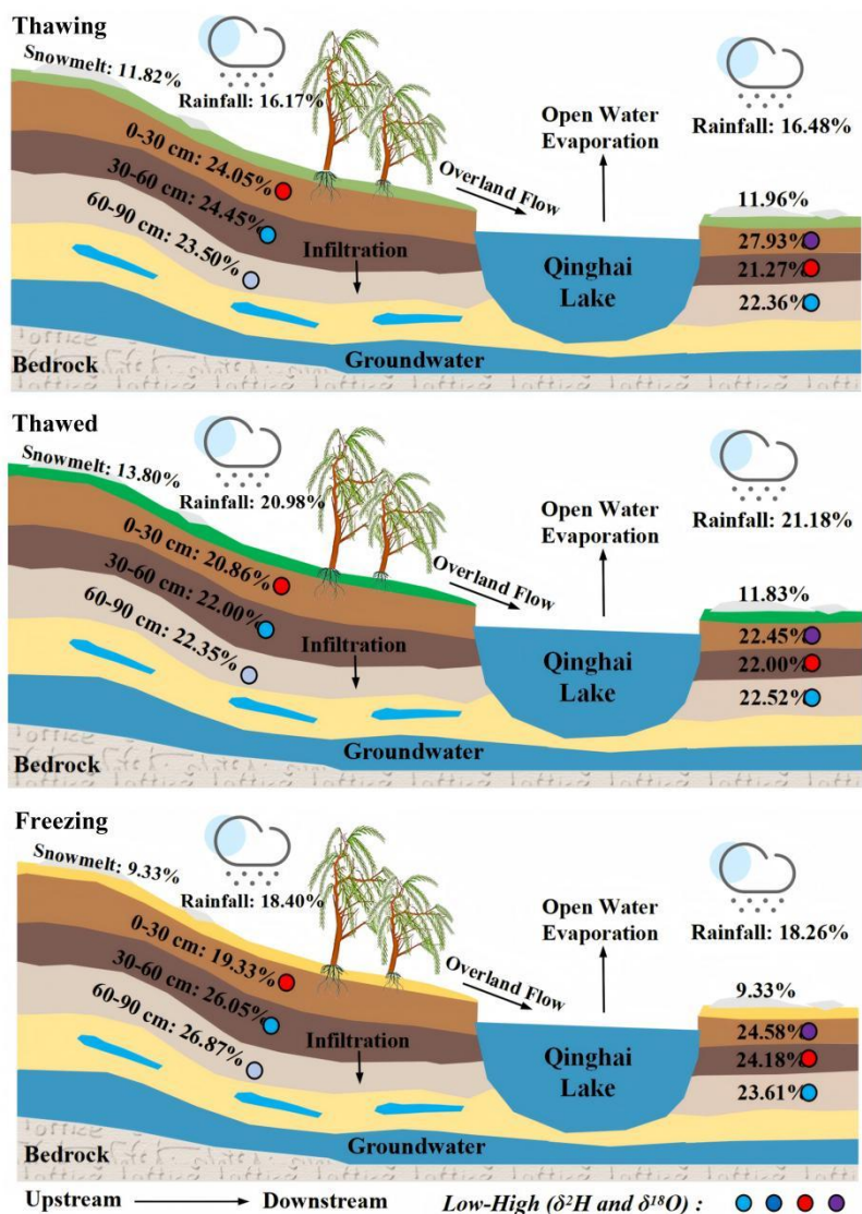
511 512 Fig. 8. Graphical summary of the contributions of rainfall, snowmelt, and soil water 513 from different depths to groundwater recharge during the FT periods.
