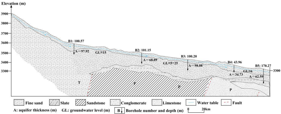
Fig. 2. Hydrogeologic profile of the QLB (based on Peng et al., 2015; Li et al., 2022; Peng et al., 2023).
