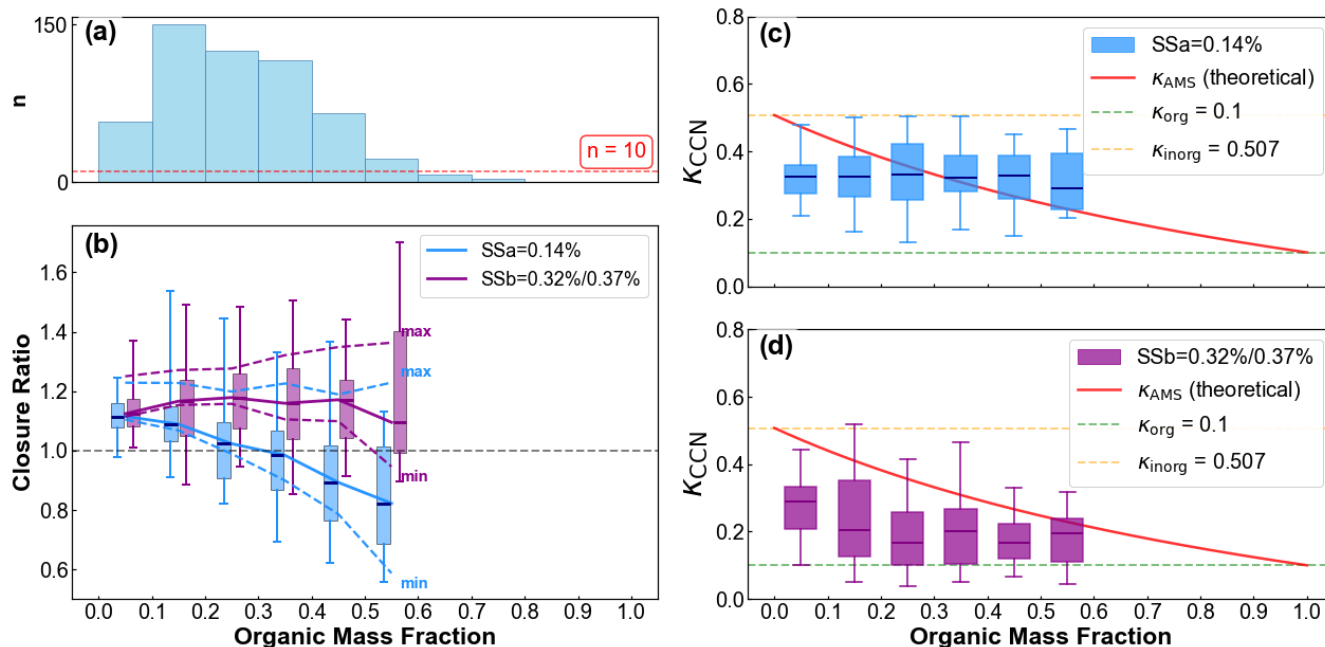
400 Figure 9. Relationship between CR and observed hygroscopicity ( \kappa_{\text{ccn}} ) with MFor g for ACE-ENA. (a) number of flight legs in each MFor g bins. (b) box plots of CR as a function of MFor g at two supersaturations (SSa = 0.14%, SSb = 0.32/0.37%). Dashed lines represent the sensitivity results of maximum and minimum values of median CR derived from the extreme range of density and hygroscopicity parameters reported in literature. (c–d) Comparison between \kappa derived from aerosol and CCN number concentration ( \kappa_{\text{ccn}} , box plots) and from AMS-measured chemical composition ( \kappa_{\text{AMS}} , red line), c for SSa and d for SSb. The pre-defined 405 hygroscopicity for organics and inorganics ( \kappa_{\text{inorg}} = 0.507 , \kappa_{\text{org}} = 0.1 ) are also plotted in dash. In all box plots, the horizontal line indicates the median, the box boundaries represent the 25th and 75th percentiles, and the whiskers extend to the 5th and 95th percentiles. Only data sample number > 10 was plotted in (b), (c) and (d).
