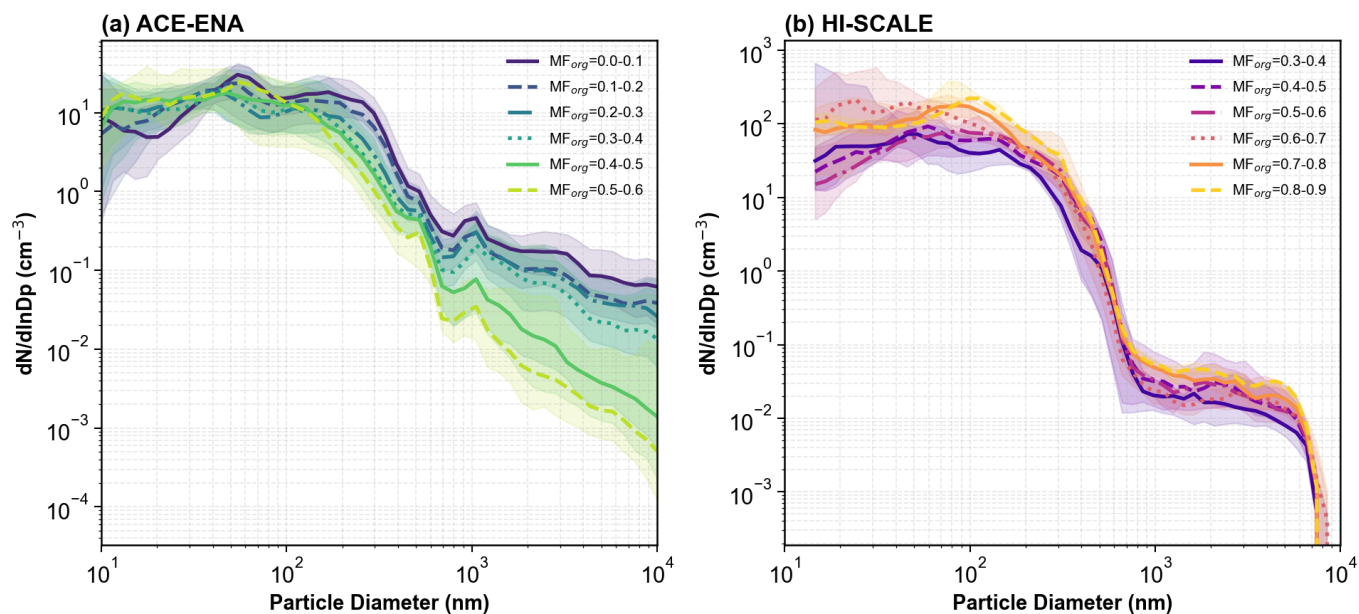
375 Figure 8. Aerosol particle size distribution in different MForg ranges in (a) ACE-ENA and (b) HI-SCALE.
