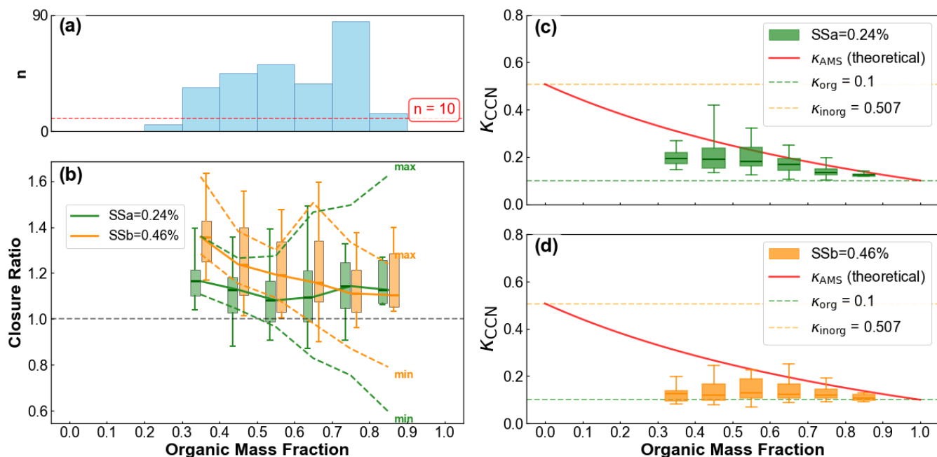
445 Figure 10. Same as Figure 9 but for HI-SCALE.
