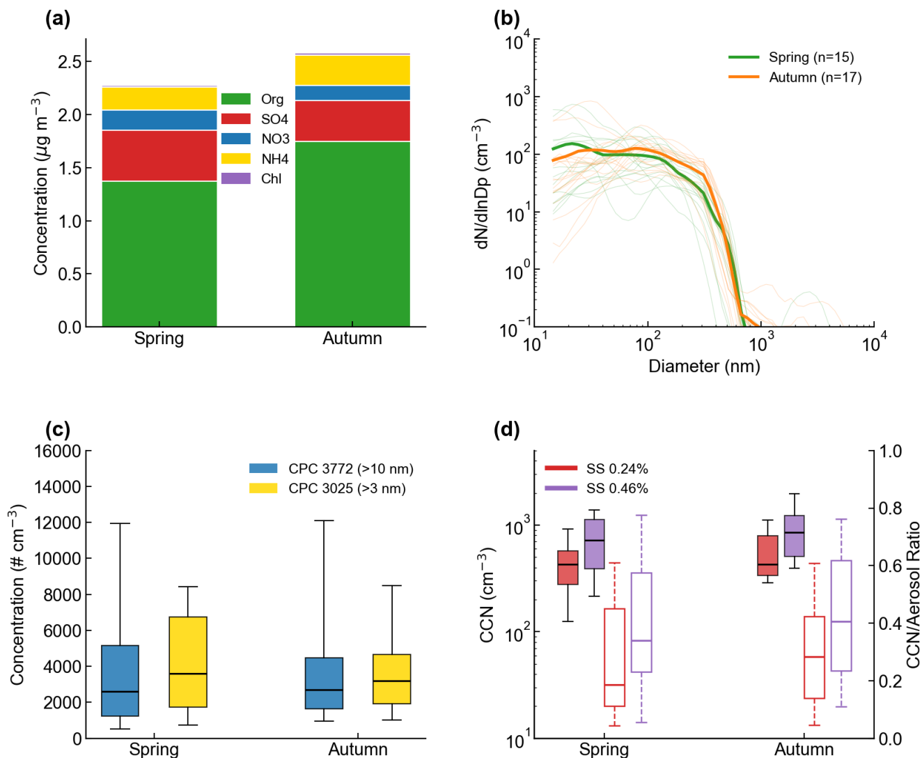
265 Figure 4. Same as Figure 3, but for the HI-SCALE campaign (continental environment) and here spring is for IOP1 (April 5 - May 20, 2016) and autumn is for IOP2 (August 29 – September 17, 2016).
