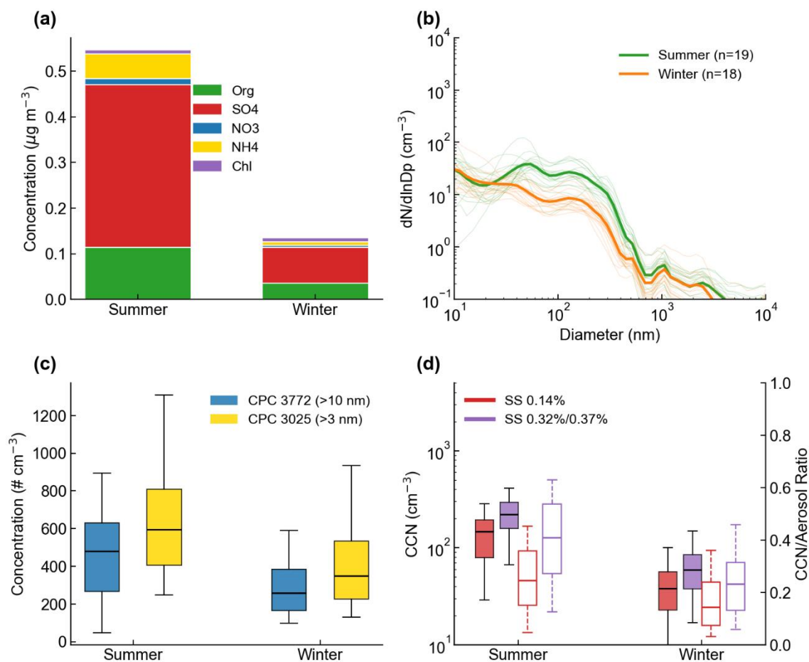
230 Figure 3. Seasonal variations of aerosol and CCN properties during the ACE-ENA campaign (marine environment). (a) Aerosol chemical composition measured by AMS. (b) Seasonal-mean (thick) and flight-mean (thin) aerosol number size distributions from BEASD, n refers to the number of dates. (c) Total aerosol number concentrations measured by CPC 3772 (> 10 nm) and CPC 3025 (> 3 nm). (d) CCN number concentrations and activation fraction (the ratio of CCN number concentration over aerosol number concentrations, dashed lines) at two supersaturations (SSa = 0.14%, SSb = 0.32% in summer and 0.37% in winter, respectively). 235 Summer is for IOP1 (June 21- July 20, 2017) and winter is for IOP2 (January 19 –February 19,2018). In the box plots, the center
