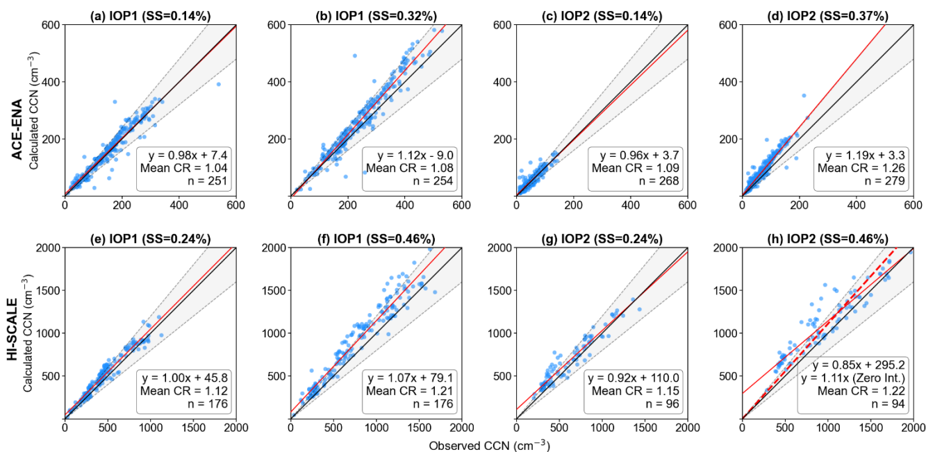
320 Figure 6. Same as Figure 5, but stratified by season and supersaturation level.
