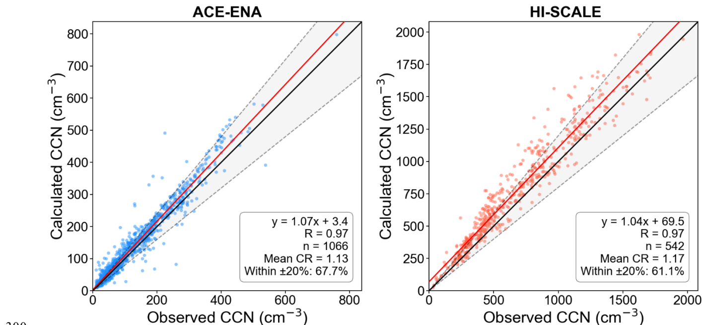
Figure 5. Comparison of observed and calculated CCN number concentrations for ACE-ENA (left) and HI-SCALE (right). Each dot represents mean CCN concentration of one flight leg. The black line denotes the 1:1 reference line, with the gray shaded area represents the ±20% range. The red line indicates the best-fit linear regression. The linear fitting function, R value, sample number, mean Closure Ratio (CR = calculated CCN/ observed CCN) and percentage of samples within ±20% range are given in the figure inserts.
