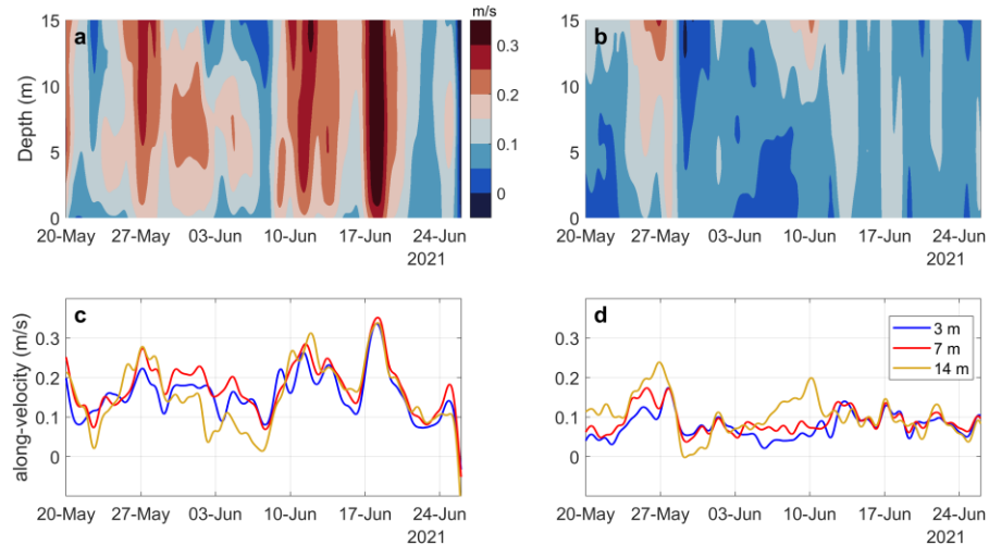
Figure 12.44. Low-pass filtered currents correspond to SBN-NW (a, c), and to SBN-S (b, d). The upper panels (a, b) show depth-time distributions of along-axis velocity, obtained by rotating the velocity field onto the principal axis of variability (PCA), which defines the dominant flow direction. The panels (c, d) present time series at selected depths from the bottom (3, 7, and 14 m).
