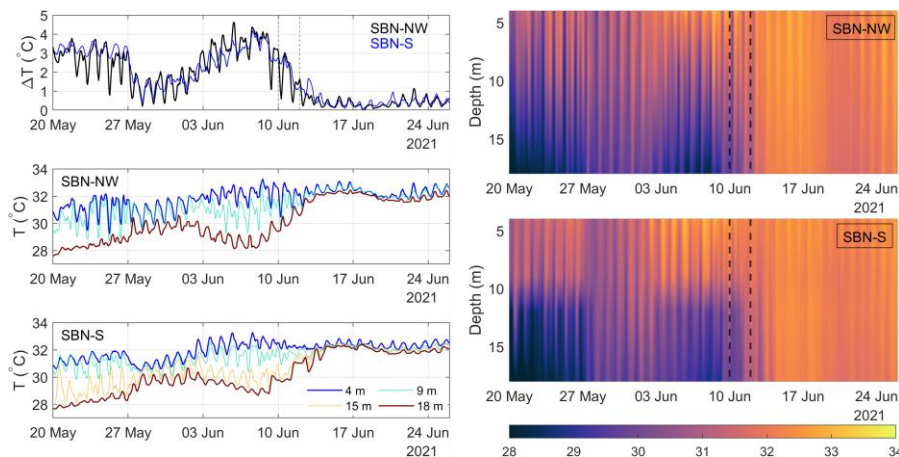
Figure 11.10. Representative episode of strong vertical thermal variability at SBN-NW and SBN-S. Left column: (top) near-surface to near-bottom temperature difference ( \Delta T = 4\text{m} - 18\text{m} ); (middle and bottom) temperature time series at instrumented depths (6 h moving mean) for SBN-NW and SBN-S, respectively. Right column: corresponding depth-time temperature fields derived from the discrete sensors at each site. Contour plots are used to synthesize the vertical structure from discrete depth measurements.
