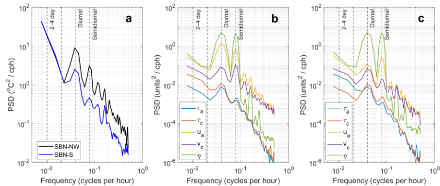
Figure 14.13. Power spectral density (PSD) of vertical temperature difference ( \Delta T = 4\text{m} - 18\text{m} ) at SBN-NW (black) and SBN-S (blue) (a). PSD of forcing components projected onto the local principal axes at SBN-NW (b) and SBN-S (c), including along- and across-axis wind stress ( \tau_a , \tau_c ), current velocity ( U_a , U_c ), and sea level ( \eta ). Vertical dashed lines indicate characteristic bands (2–4day, diurnal, semidiurnal).
