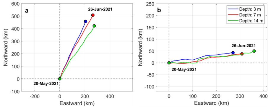
Figure 13.12. Progressive vector diagrams of the hourly ADCP currents at SBN-NW (a) and SBN-S (b), for selected depths (3, 7, and 14 m), for the period 20 May-26 June 2021.
