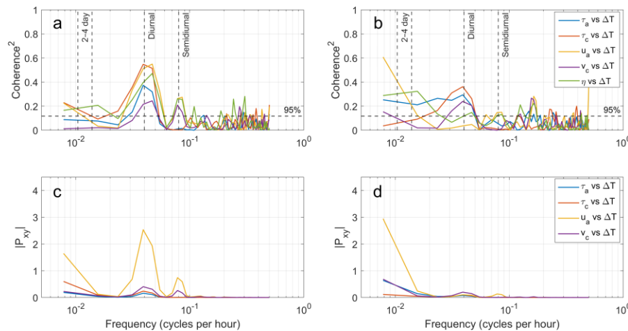
Figure 15.4. Magnitude-squared coherence and cross-spectral density magnitude between \Delta T (18m – 4m) and forcing components at SBN-NW (a, c) and SBN-S (b, d). Wind forcing is represented by along- and across-axis wind stress ( \tau_a, \tau_c ), then current velocity ( u_a, v_c ), and sea level ( \eta ). Dashed vertical lines indicate the 2–4 day, diurnal, and semidiurnal bands, and the horizontal dashed line marks the 95% coherence significance threshold.
