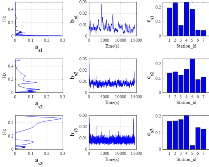
Figure 4: Decomposition results for SW-NTF on May 2, 2021
