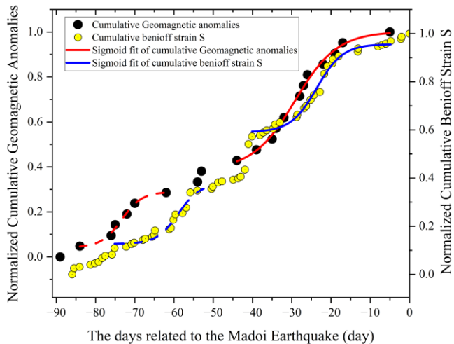
Figure 10: Comparison between cumulative geomagnetic anomalies and cumulative Benioff strain. Black dots represent cumulative geomagnetic anomalies, yellow dots denote cumulative Benioff strain, red and blue curves show the sigmoidal fits for the geomagnetic anomalies and cumulative Benioff strain, respectively. Dashed lines indicate the first acceleration phase, while solid lines represent the second acceleration phase.
