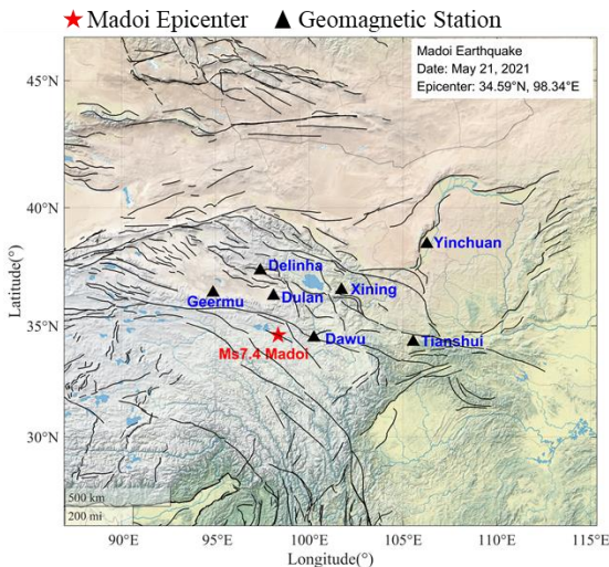
Figure 1: Epicenter of the Madoi earthquake and distribution of geomagnetic stations. The red star denotes the epicenter, black triangles represent geomagnetic stations, and black lines indicate fault lines.
